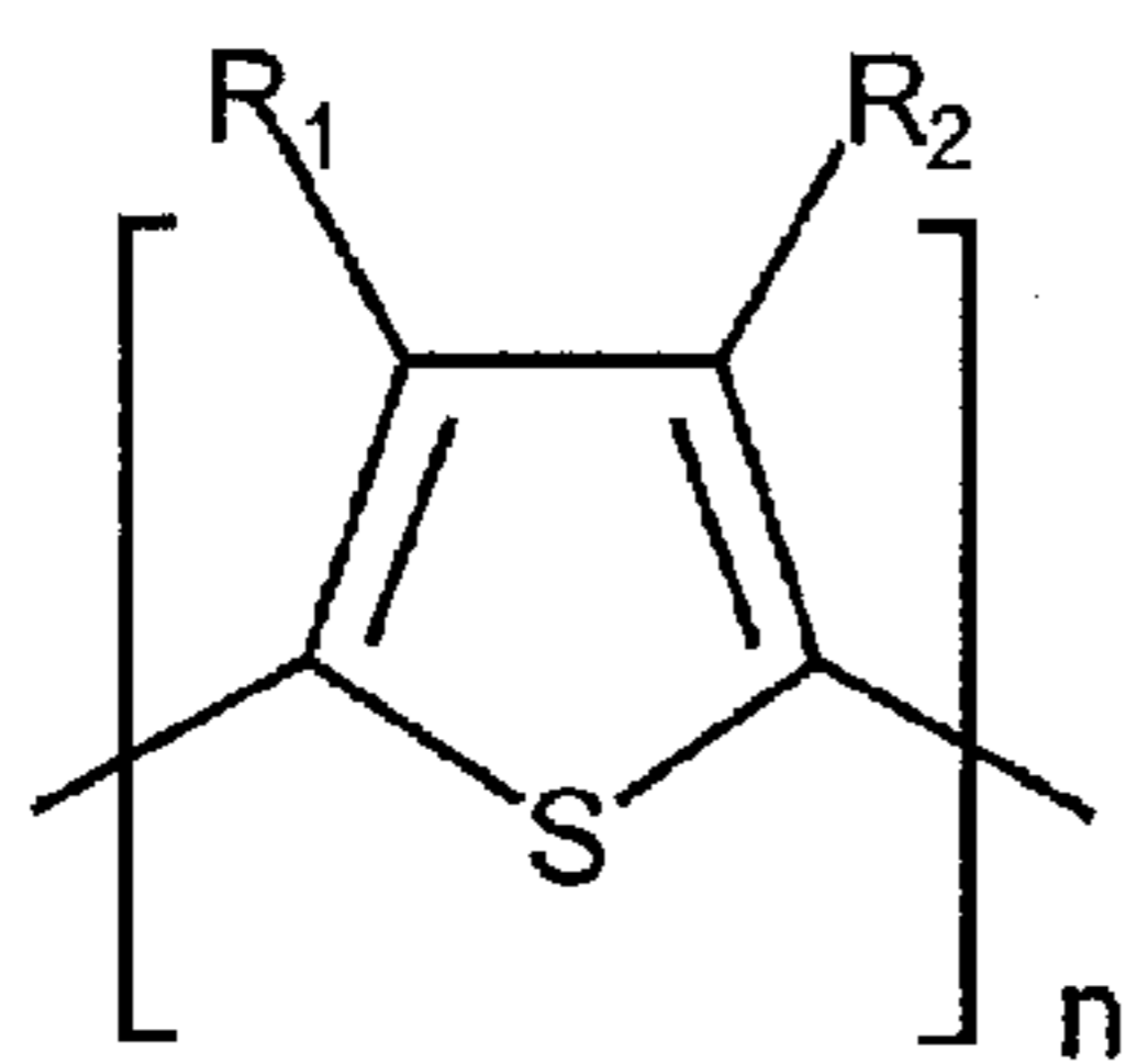
Polythiophene
