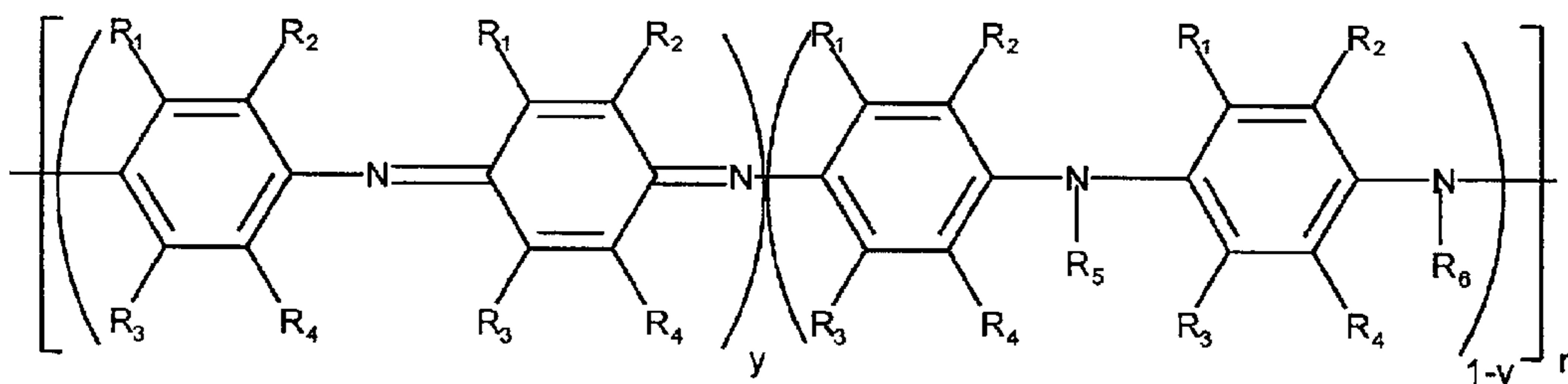
Polyaniline
