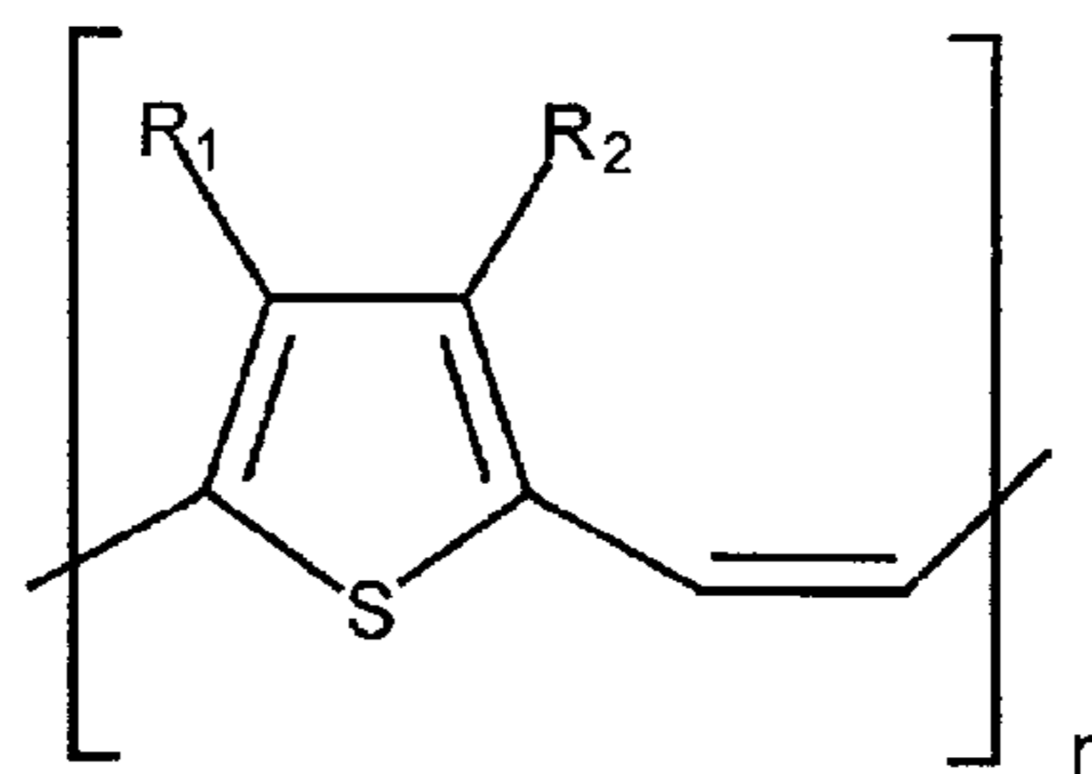
Polythiophenevinylene
