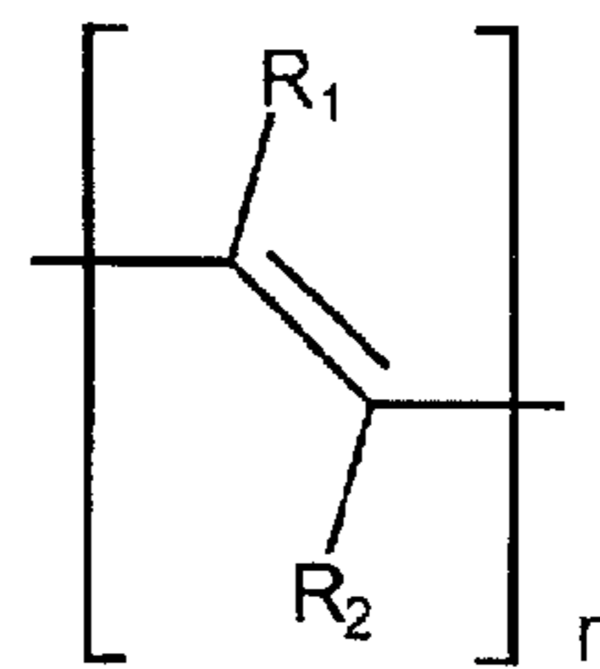
Polyacetylene
