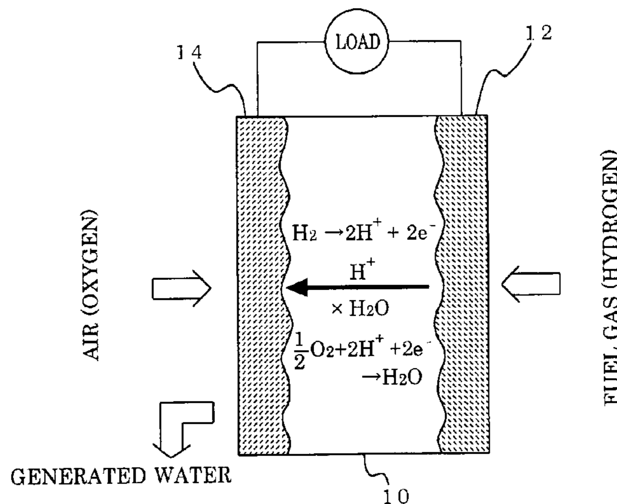
BASIC STRUCTURE OF PROTON-EXCHANGE MEMBRANE FUEL CELL
