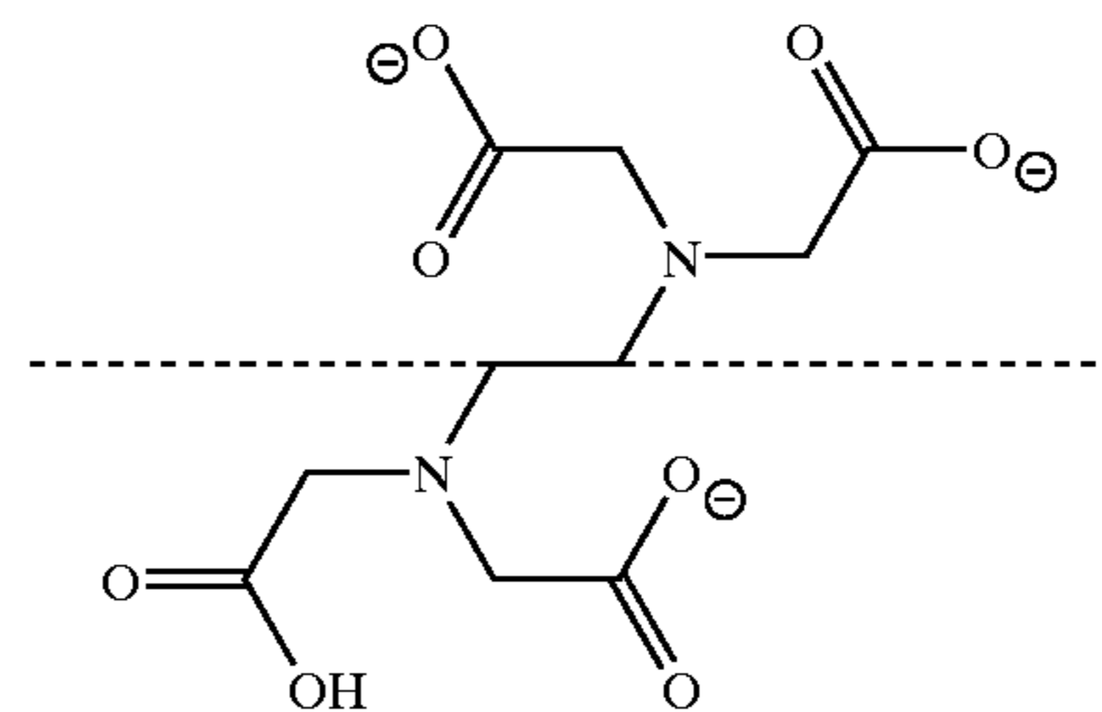
FIG. 1: The structure of ethane 1,2-diamine N,N,N',N' tetraacetic acid (EDTA). The dashed line shows the axis of two-fold rotational symmetry.
