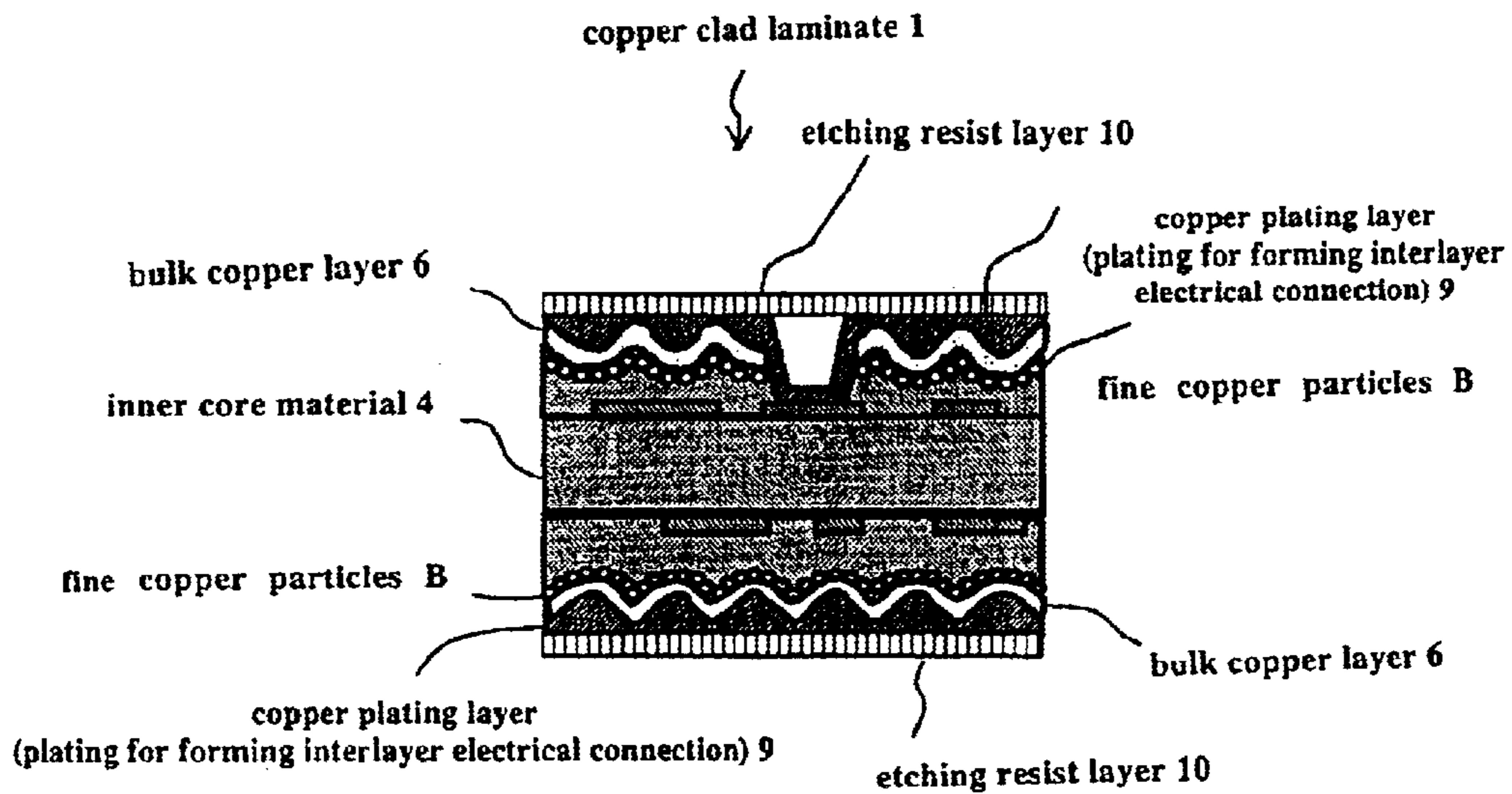
(e) Forming Etching Resist Layers
