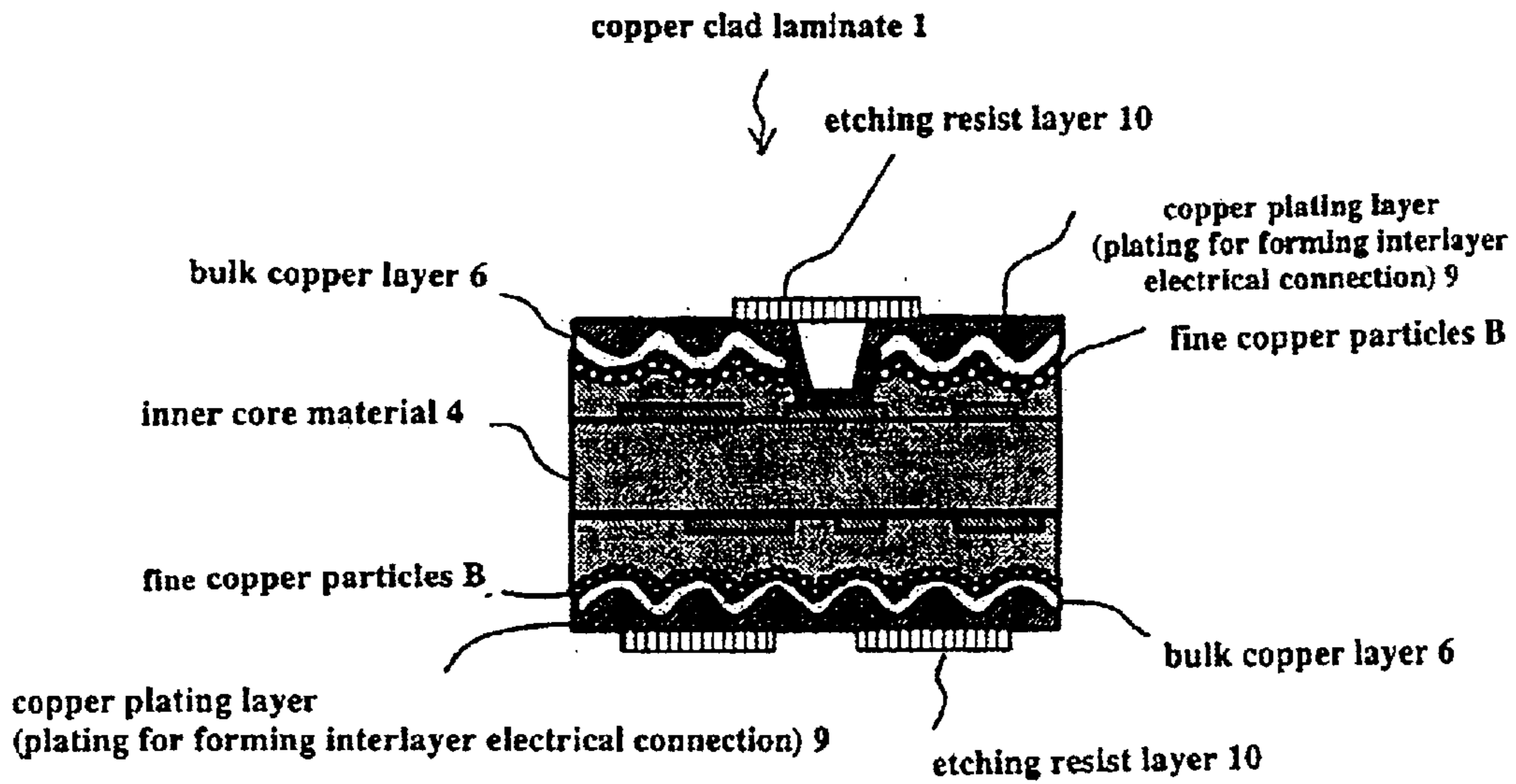
(f) Exposing and Developing the Etching Resist Layers
