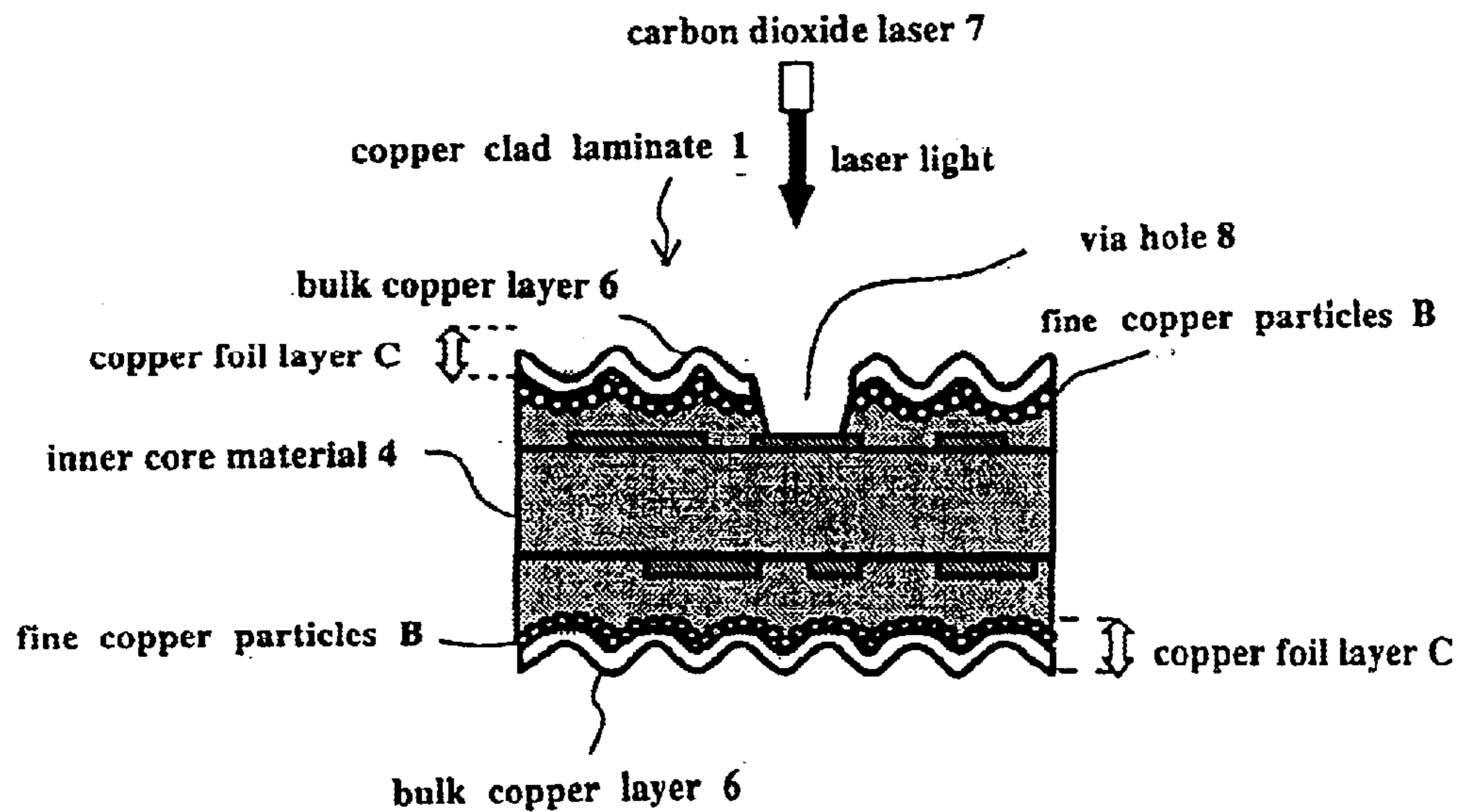
(c) Laser Treatment for Forming Holes
