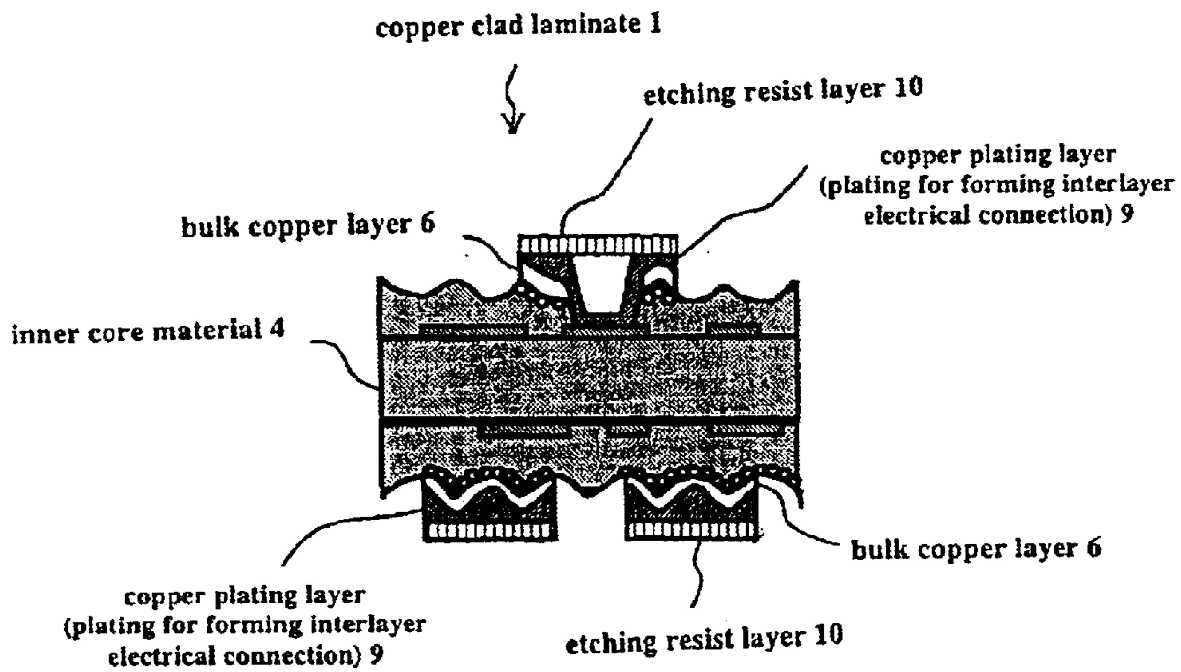
(g) Copper Etching
