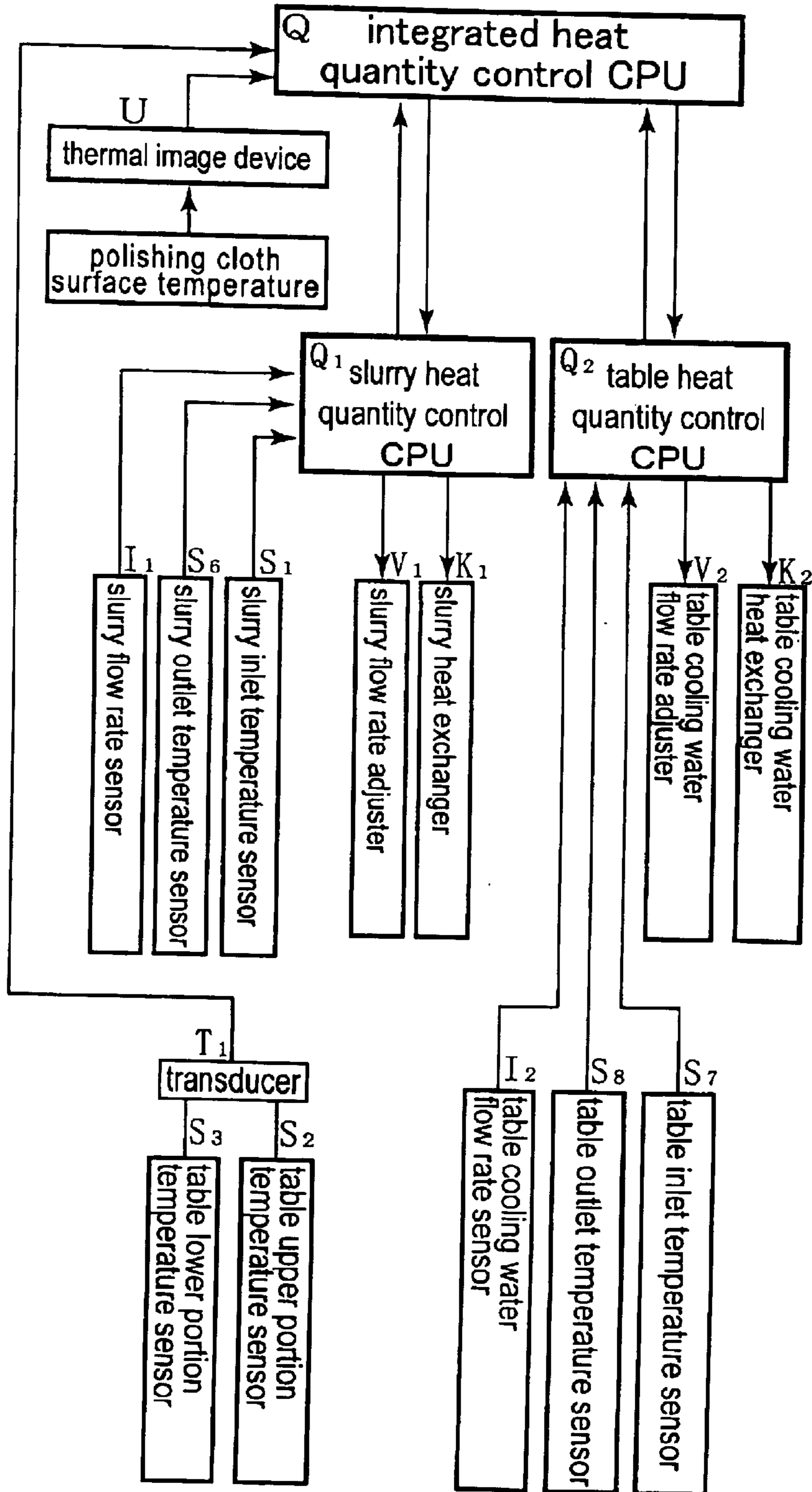
integrated heat quantity control flow chart
