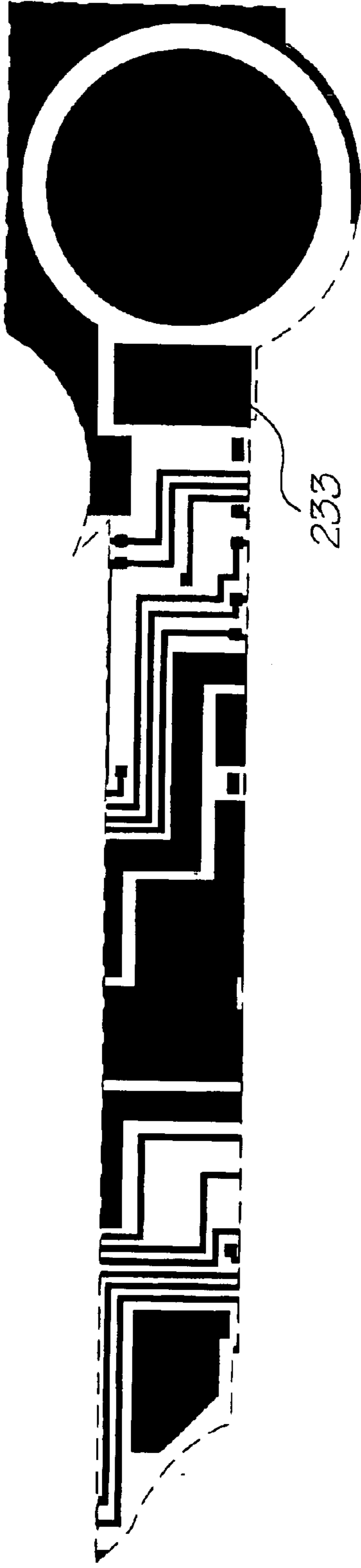
Metal 2 mask
