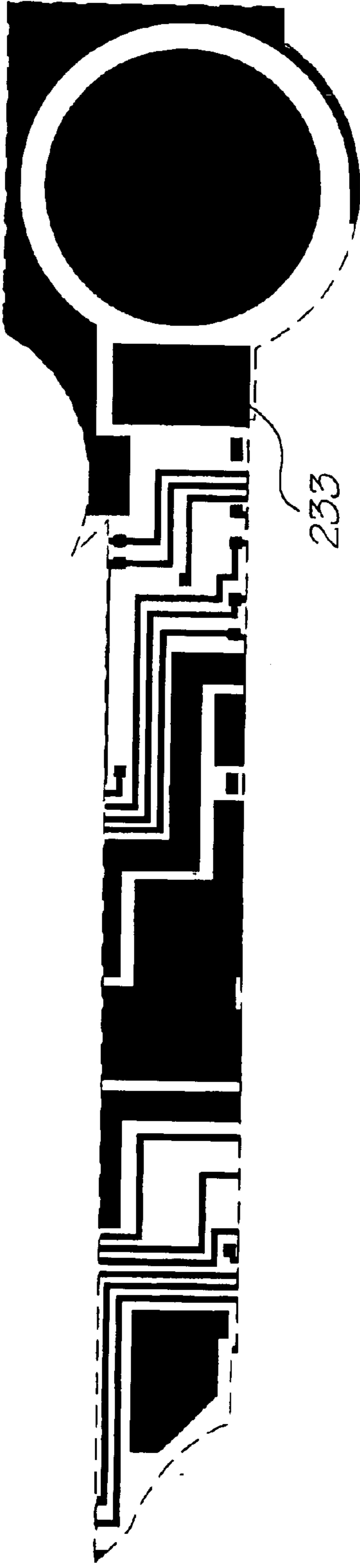
Metal 2 mask
