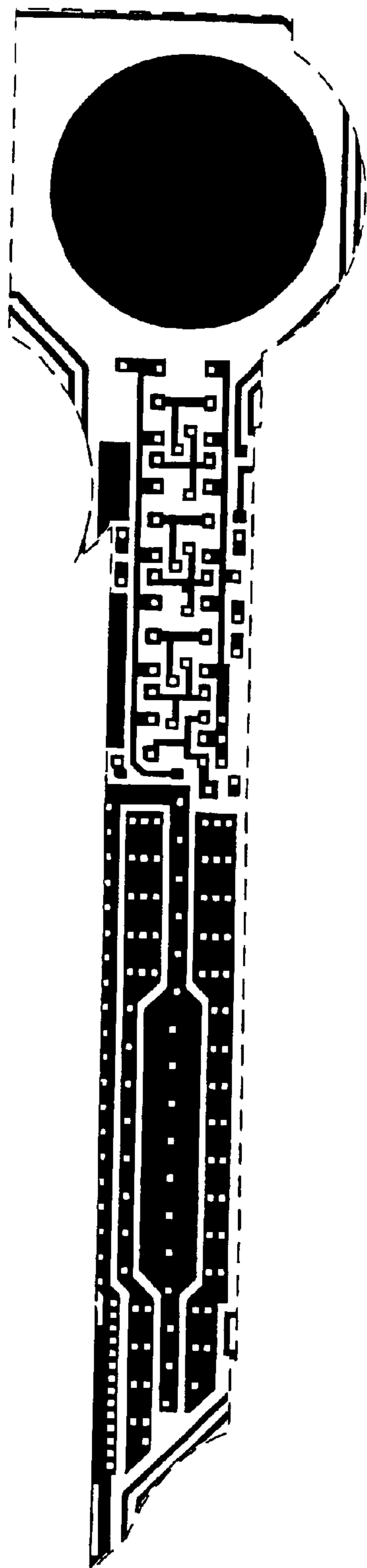
Metal 1 mask
