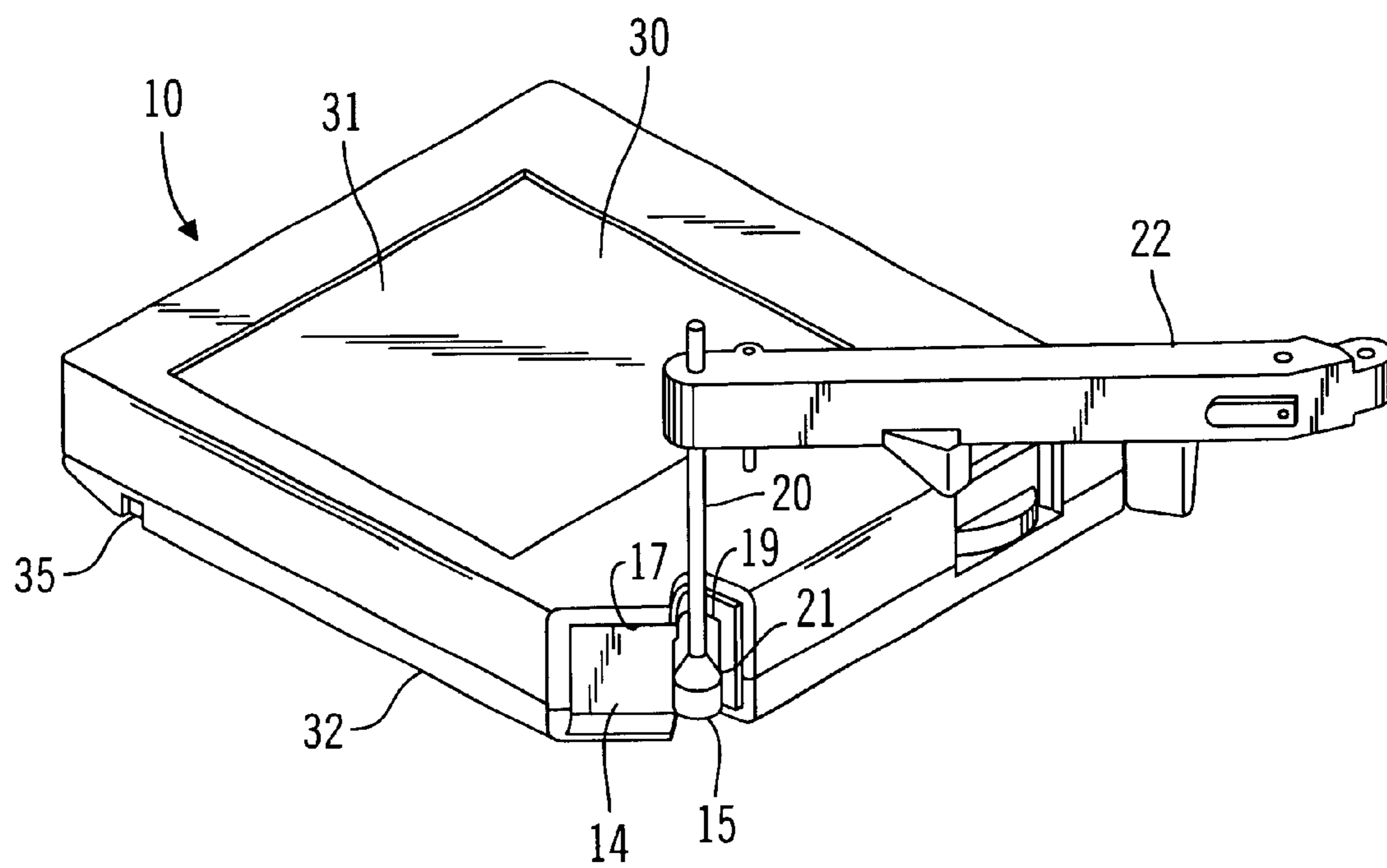
FIG. 1 PRIOR ART
