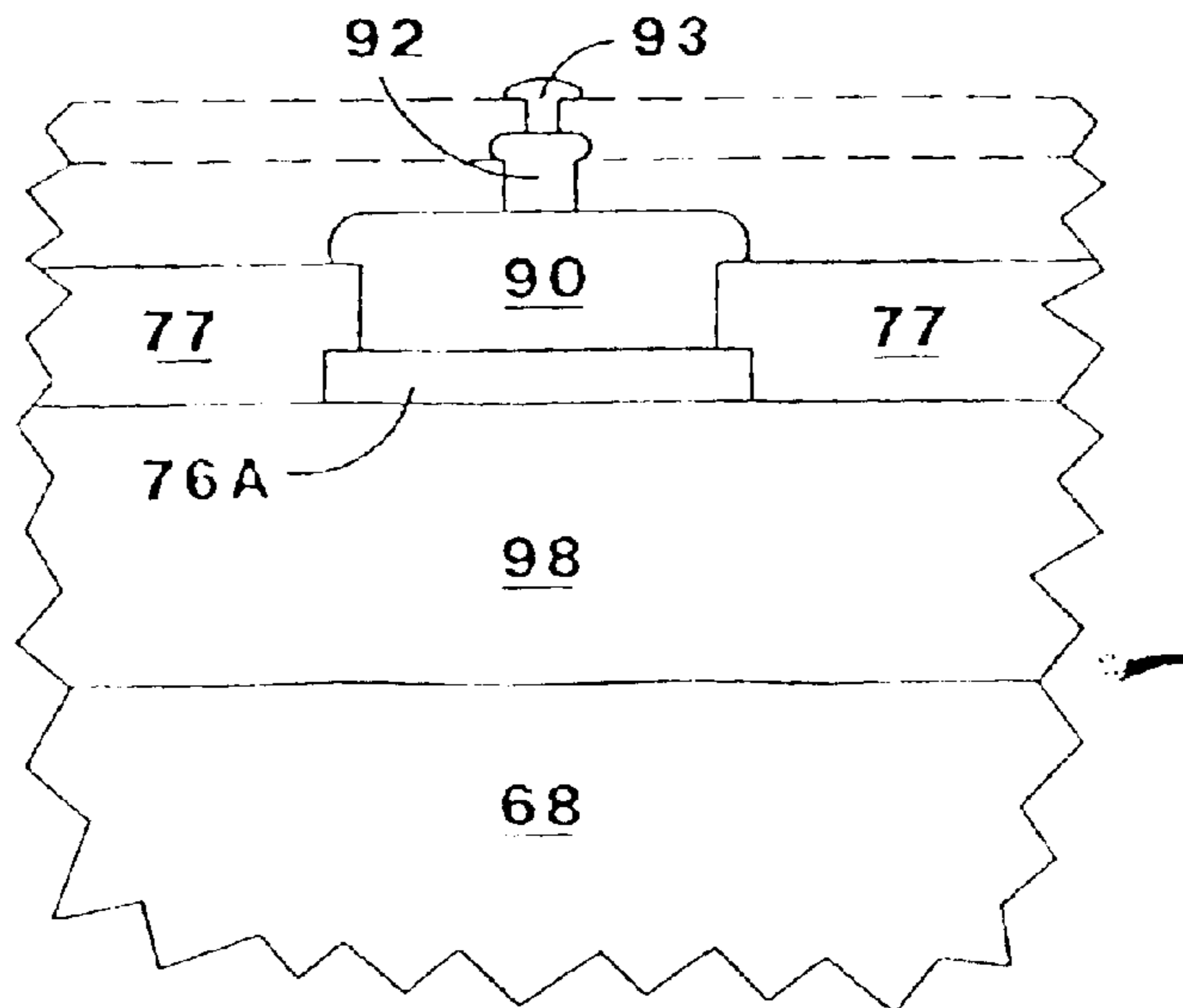
FIG. 11 PRIOR ART
