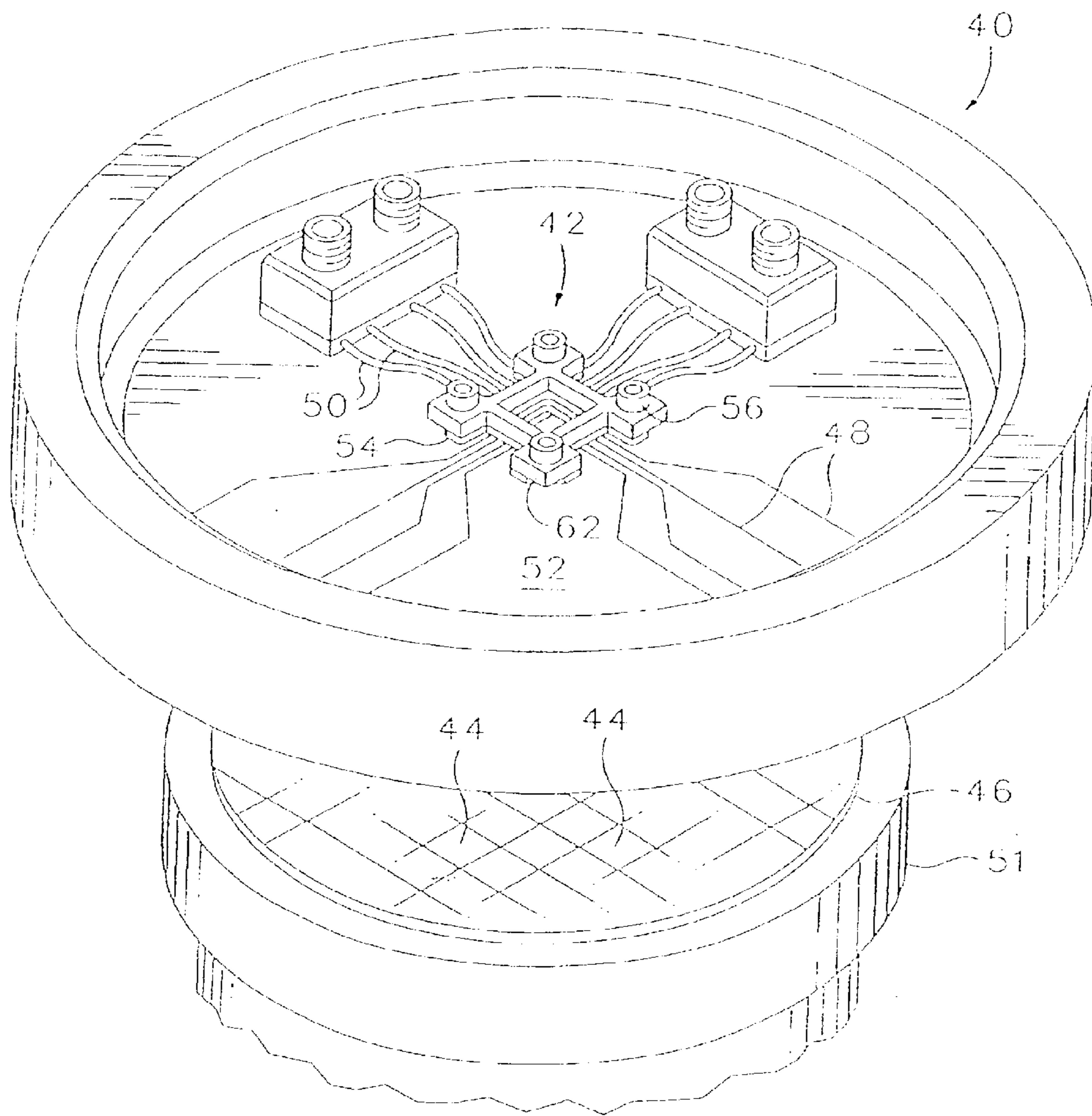
FIG. 1 PRIOR ART
