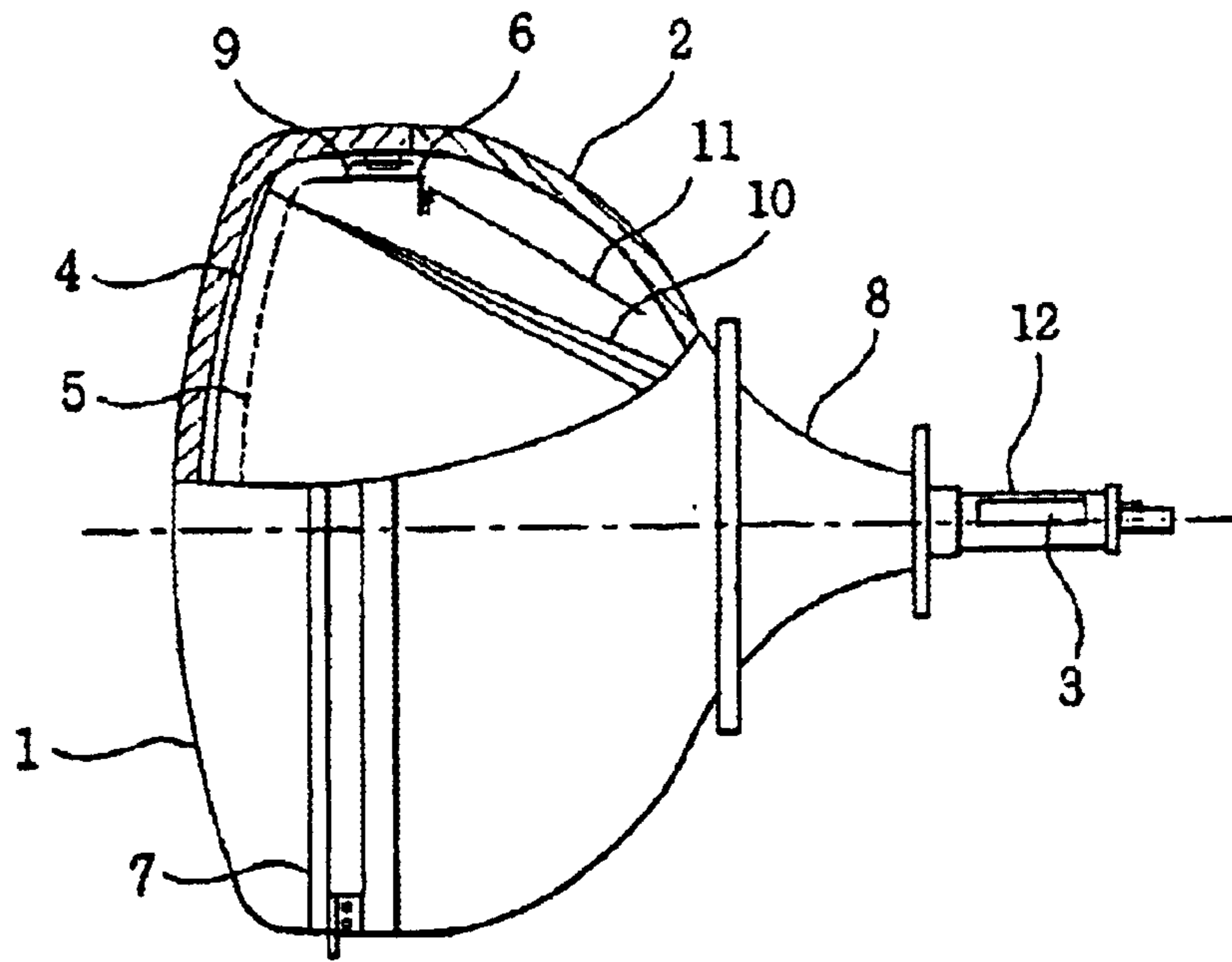
FIG. 1 BACKGROUND ART
