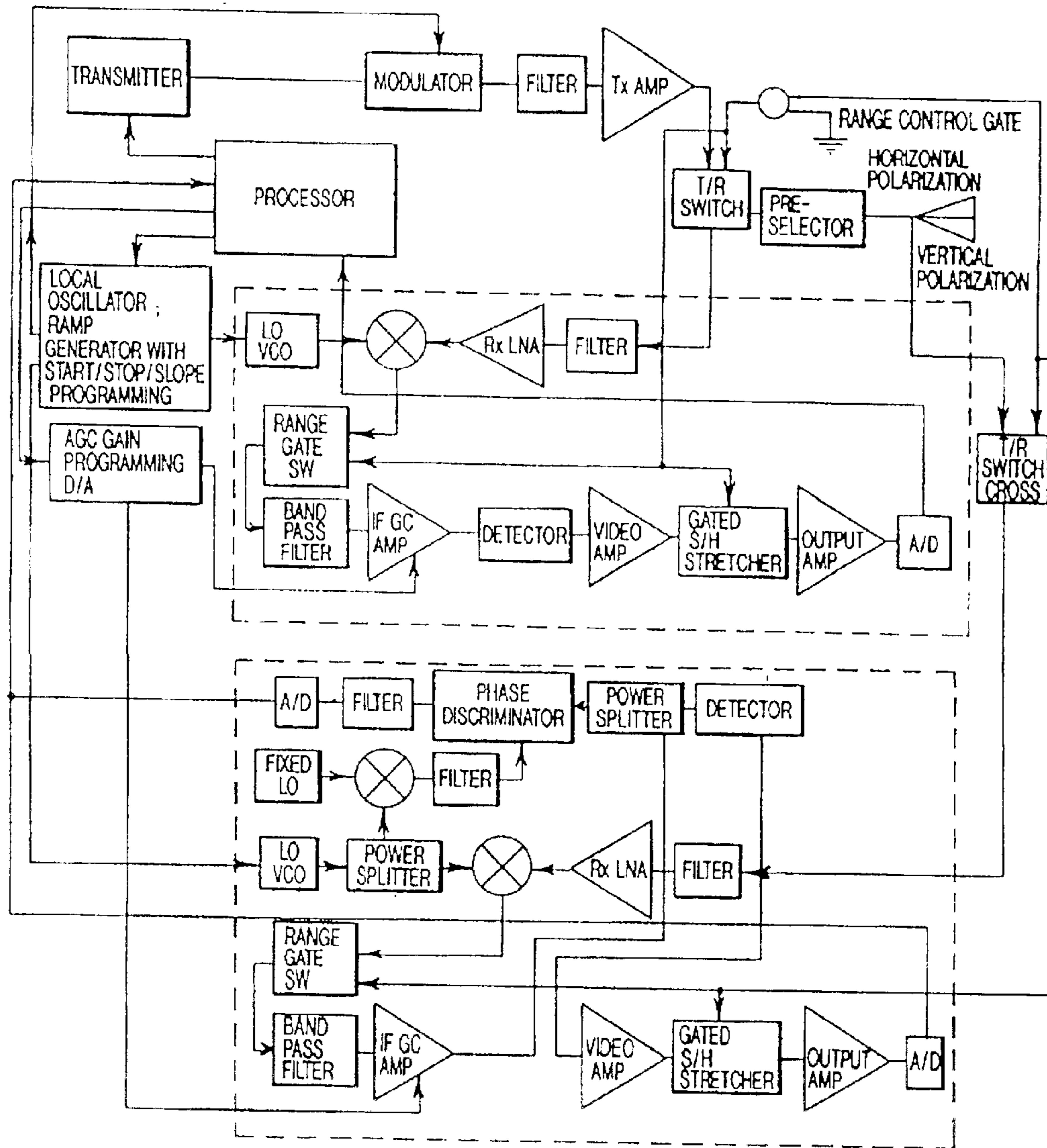
PHASE MEASUREMENT AT IF BLOCK DIAGRAM
