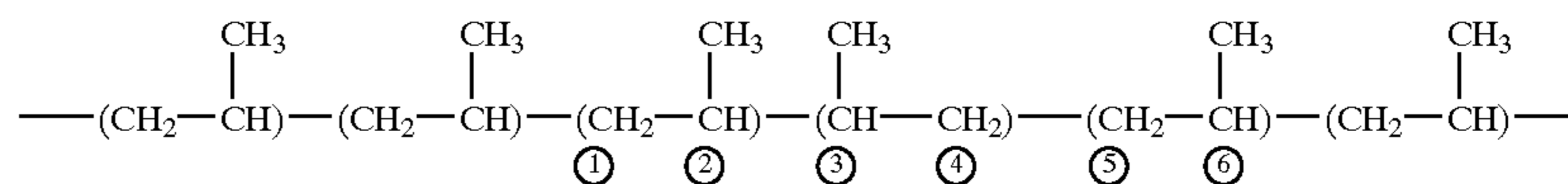
Substructure (II):
