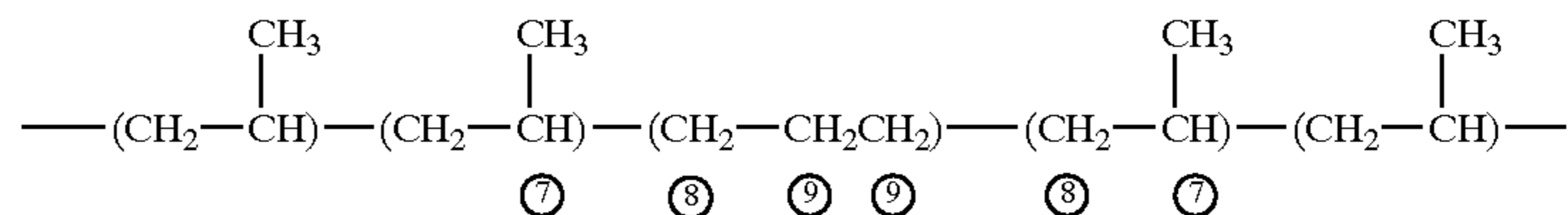
Substructure (II):
