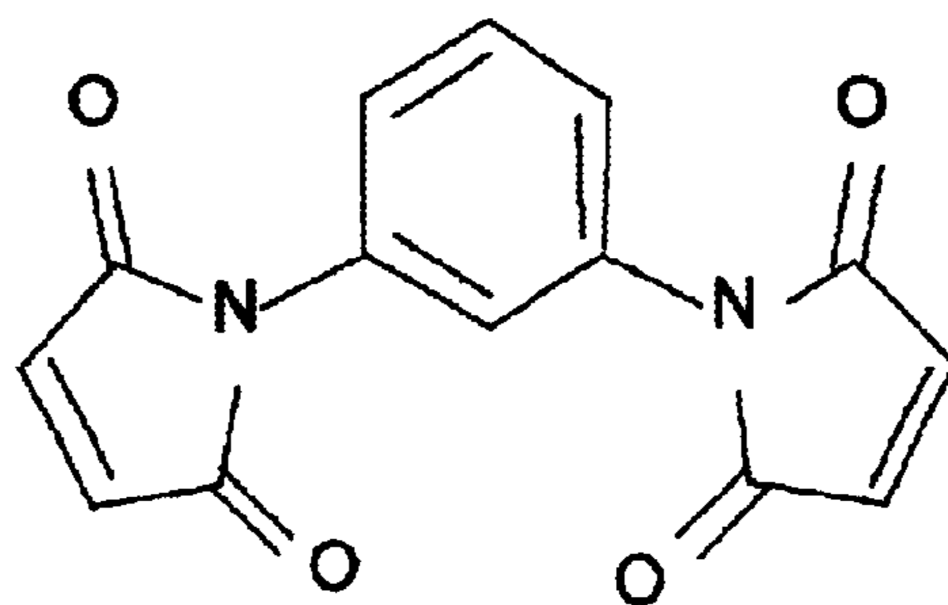
N,N'-m-phenylene-bismaleimide
