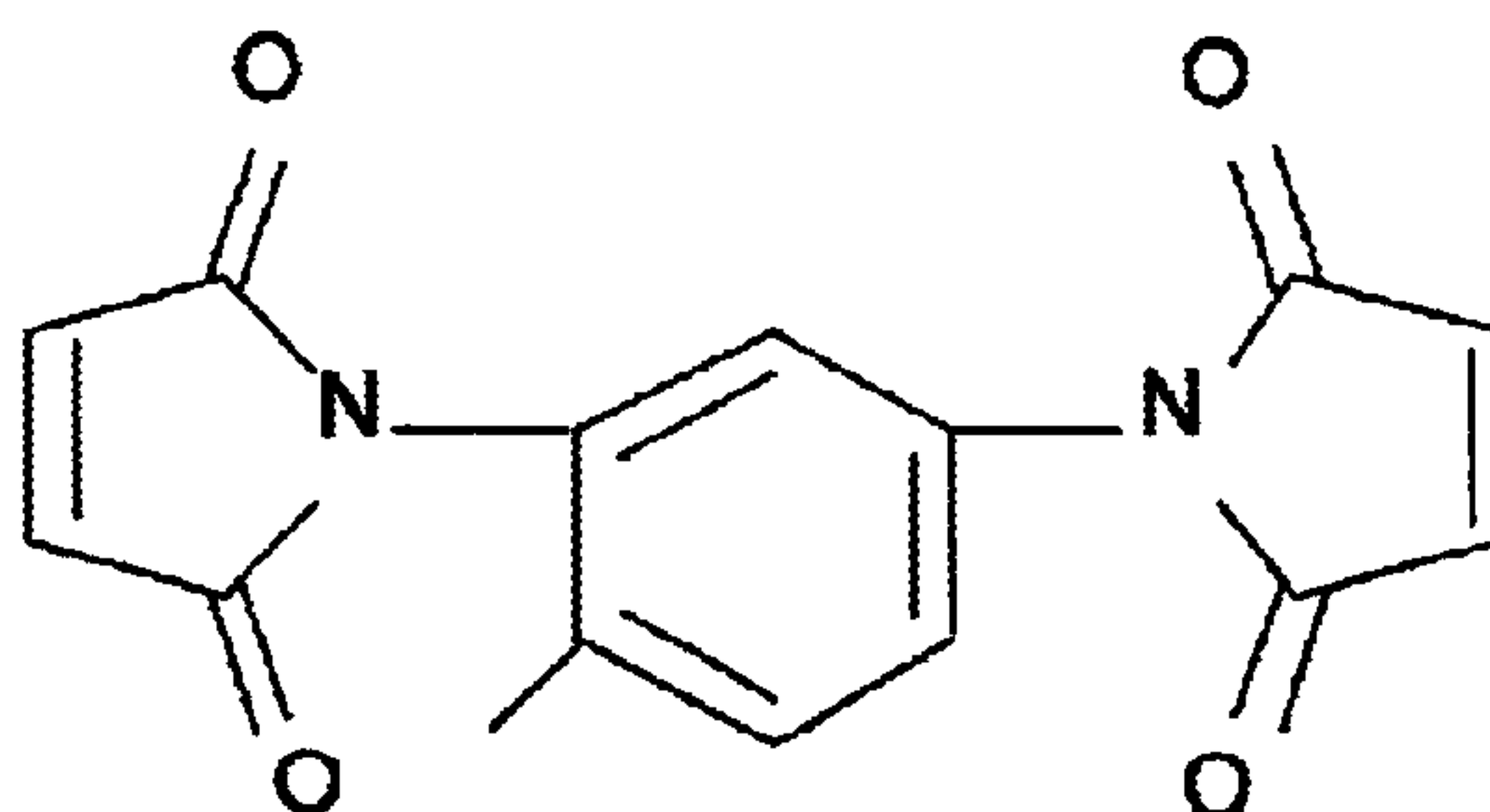
N,N'-(4-methyl-1,3-phenylene)-bismaleimide
