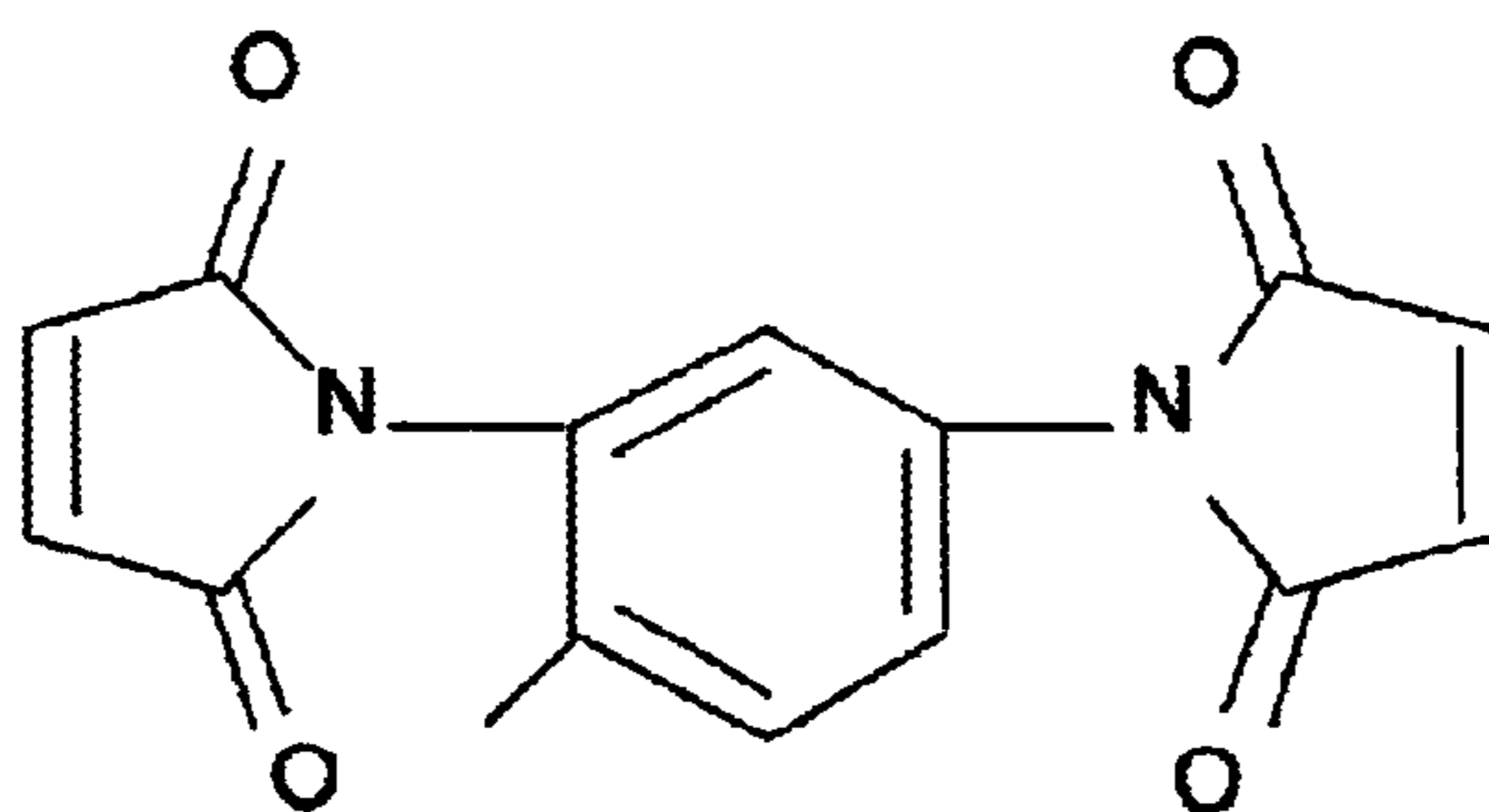
N,N'-(4-methyl-1,3-phenylene)-bismaleimide
