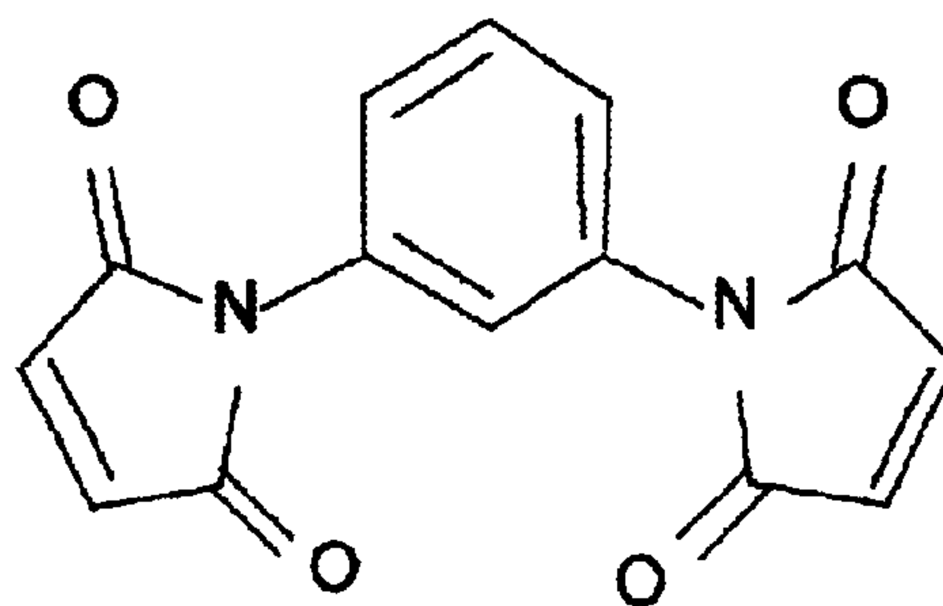
N,N'-m-phenylene-bismaleimide
