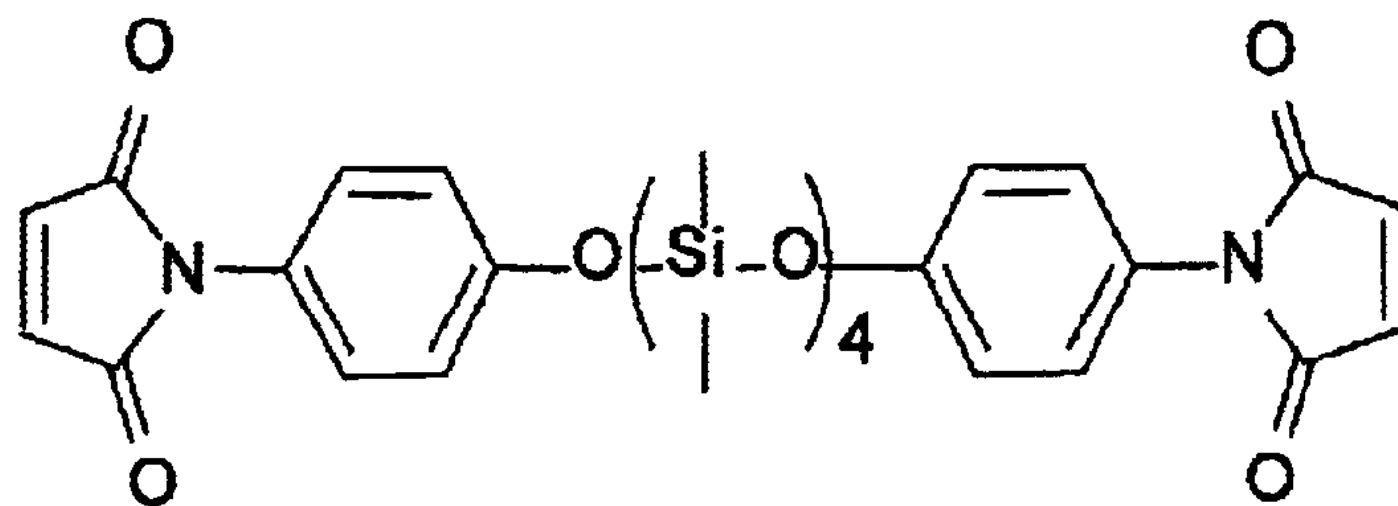
((\text{C}_4\text{H}_2\text{O}_2\text{N})\text{C}_6\text{H}_4)_2(\text{OSi}(\text{CH}_3)_2)_4\text{O}
