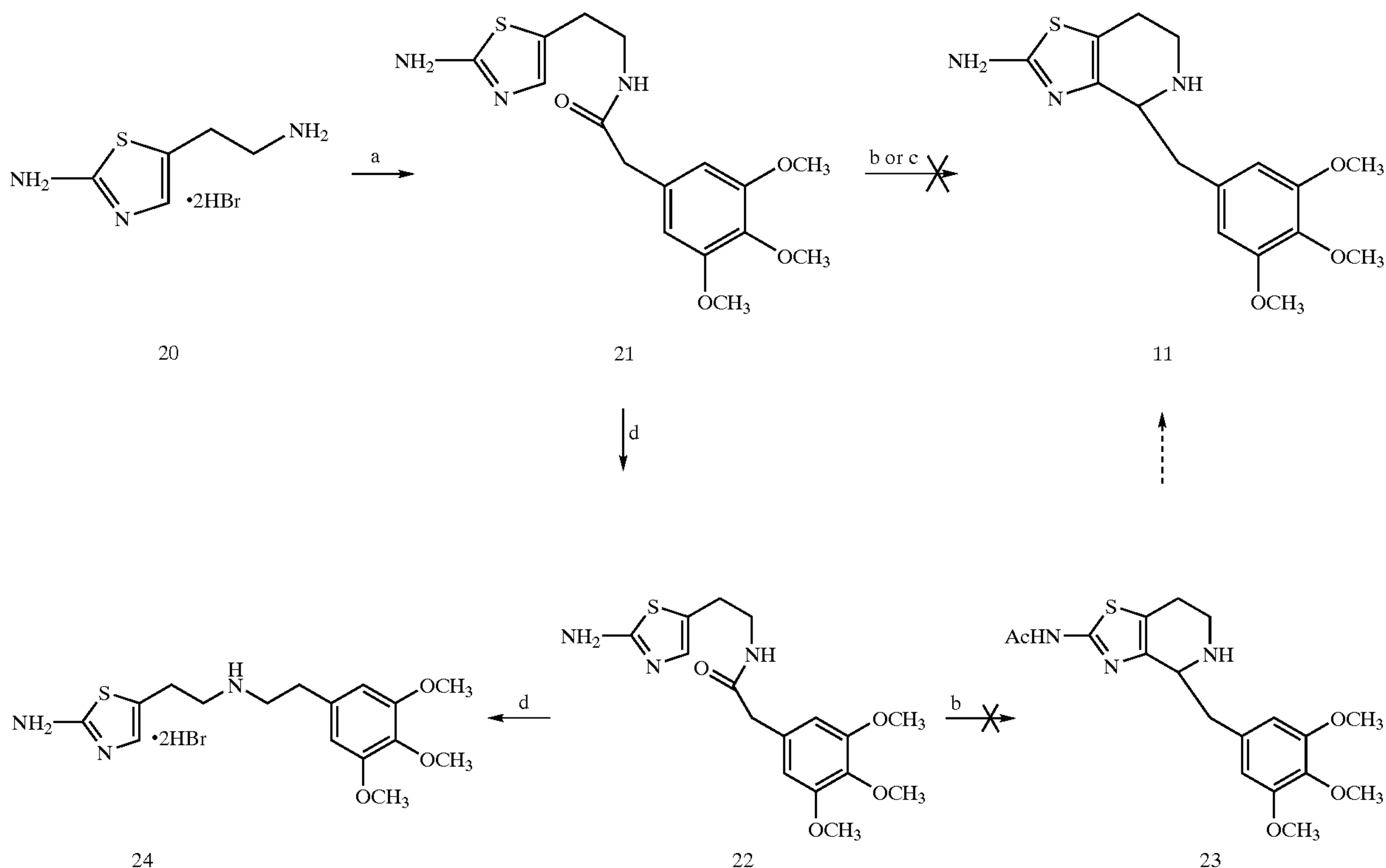
Scheme 4
