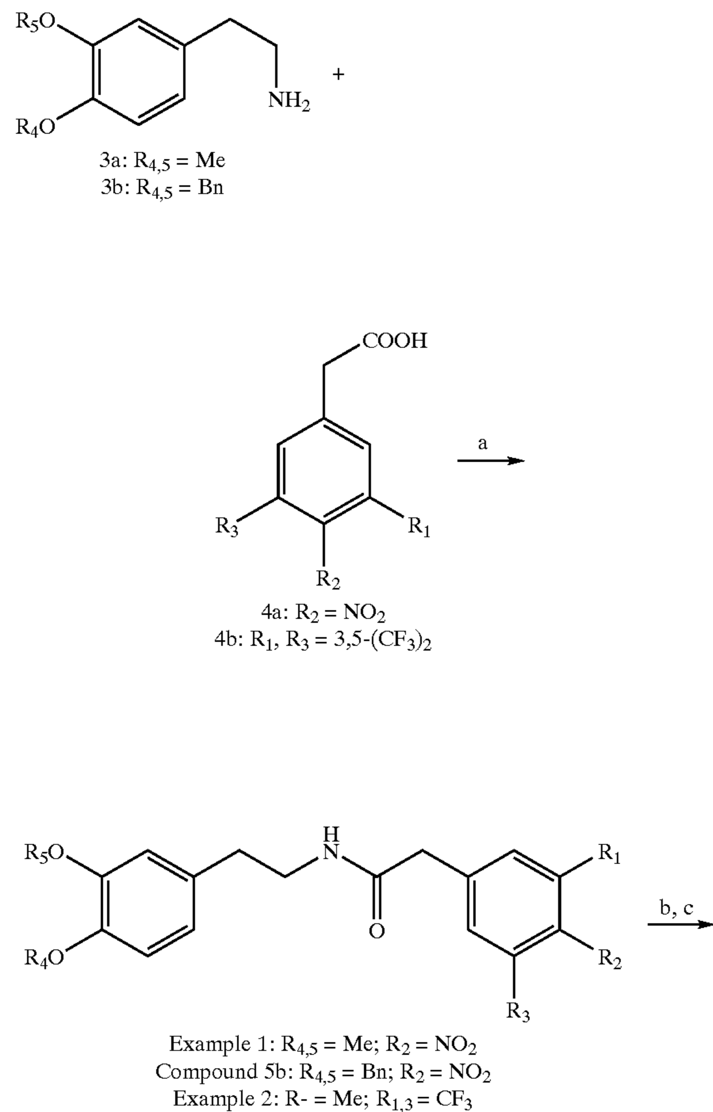
Reaction Scheme 1
