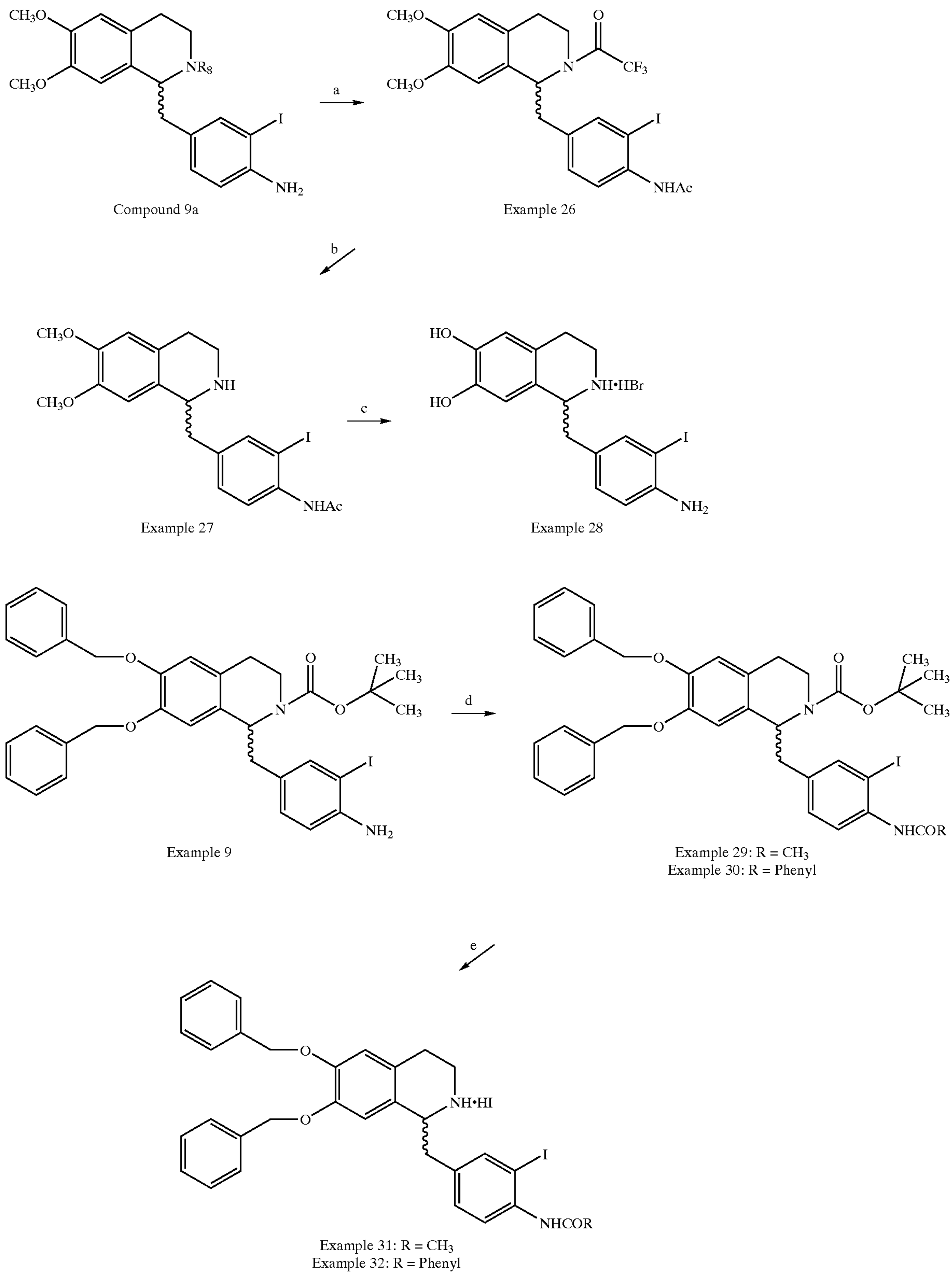
Reaction Scheme 4
