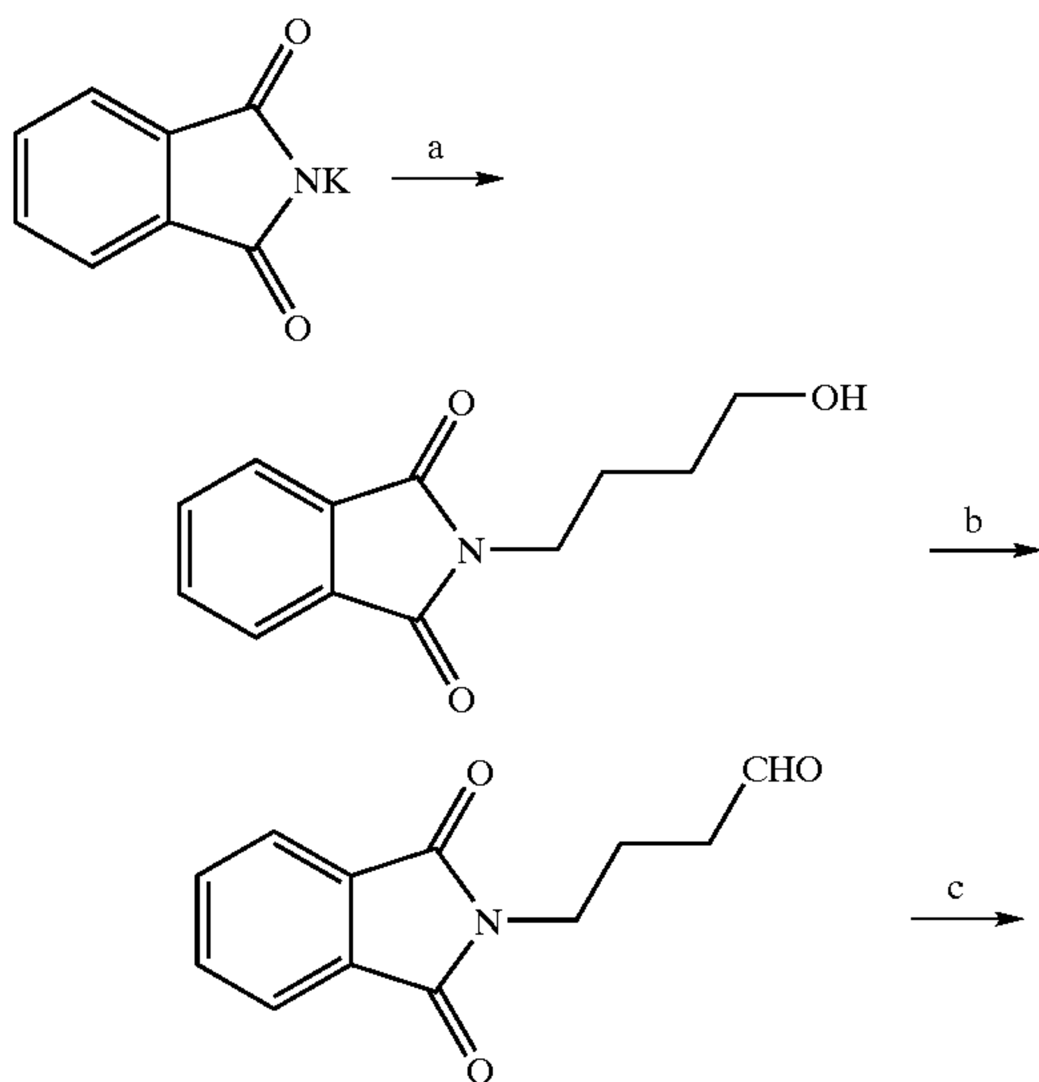
Scheme 5
