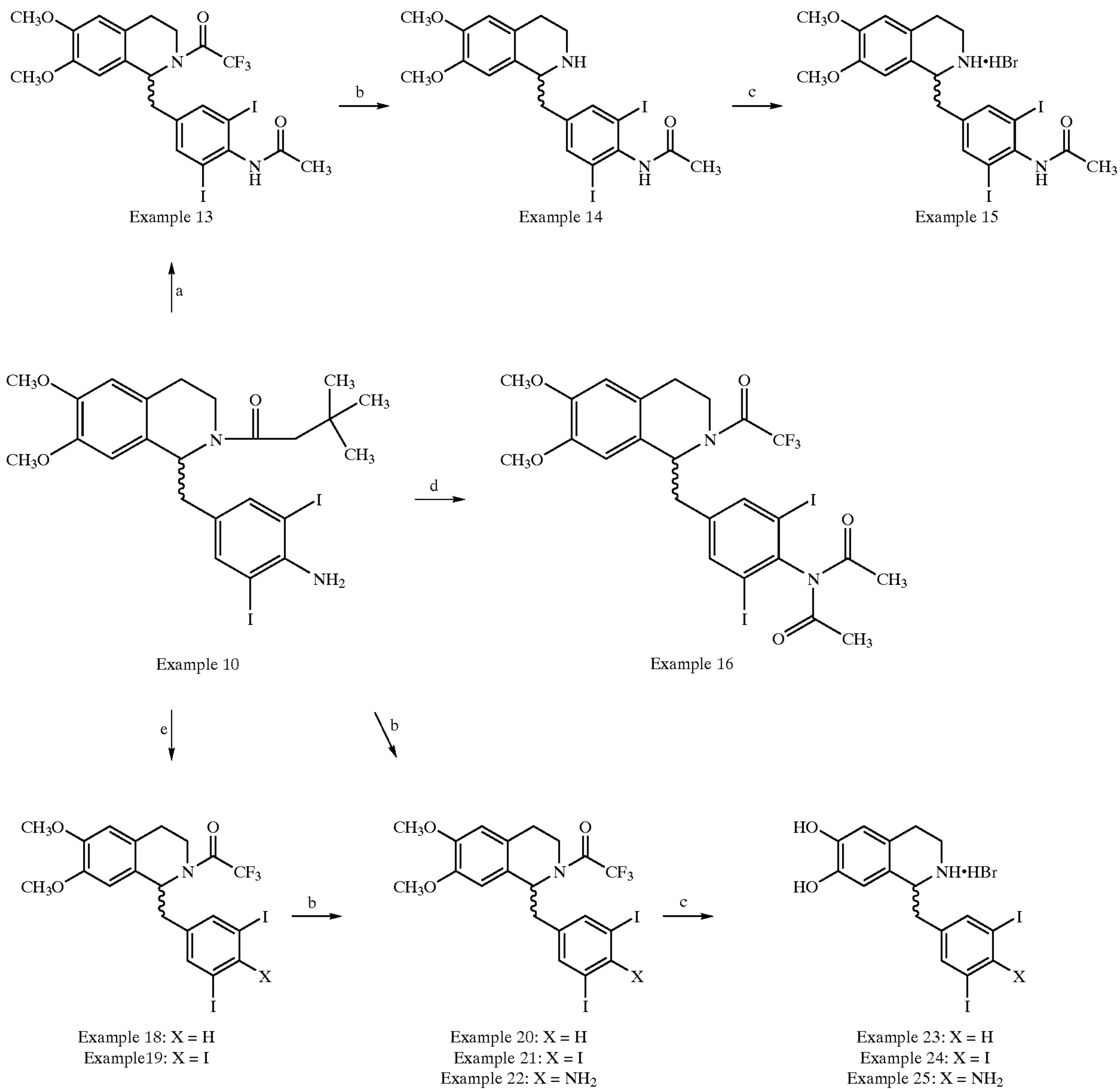
Reaction Scheme 3
