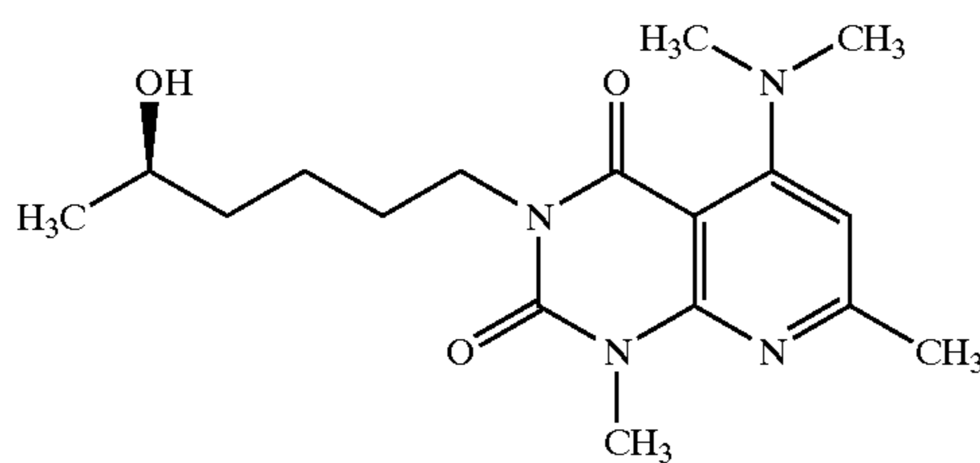
(R)-1,7-Dimethyl-5-(N,N-dimethylamino)-3-(5-hydroxyhexyl)prido[2,3-d]pyrimidine-2,4(1H,3H)-dione (CT-30103)
