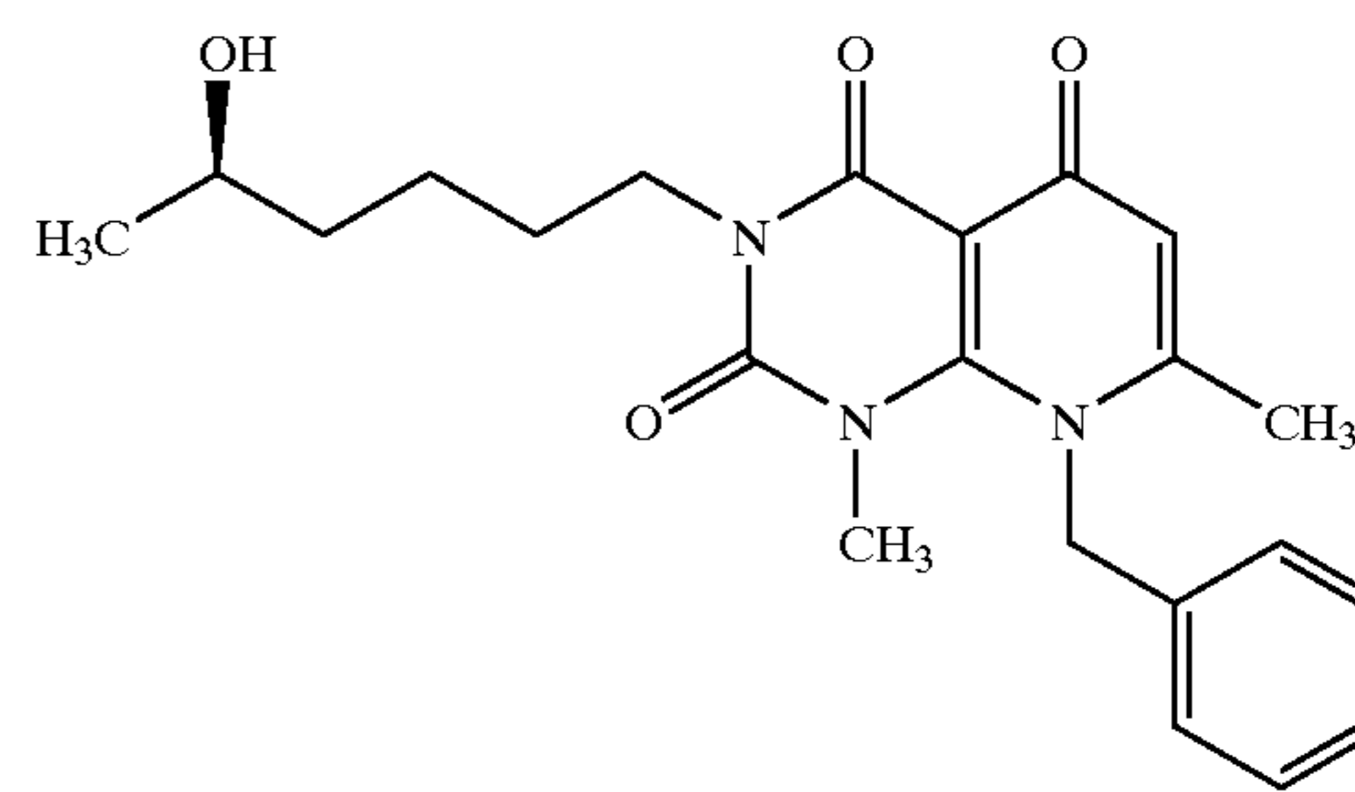
(R)-8-Benzyl-1,7-dimethyl-3-(5-hydroxyhexyl)prido[2,3-d]pyrimidine-2,4,5(1H,3H,8H)-trione
