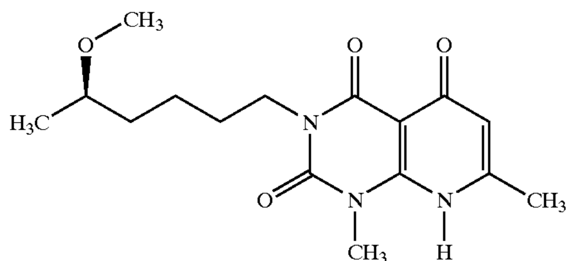
(R)-1,7-Dimethyl-3-(5-methoxyhexyl)pyrido[2,3-d]pyrimidine-2,4,5(1H,3H,8H)-trione (CT-13415)
