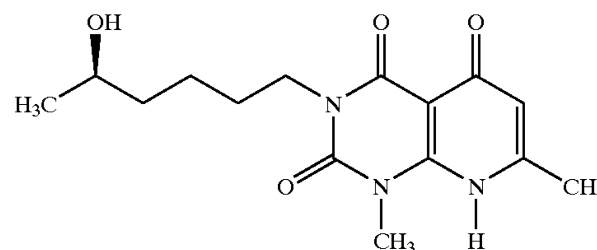
(R)-1,7-Dimethyl-3-(5-hydroxyhexyl)pyrido[2,3-d]pyrimidine-2,4,5(1H,3H,8H)-trione (CT-12480)
