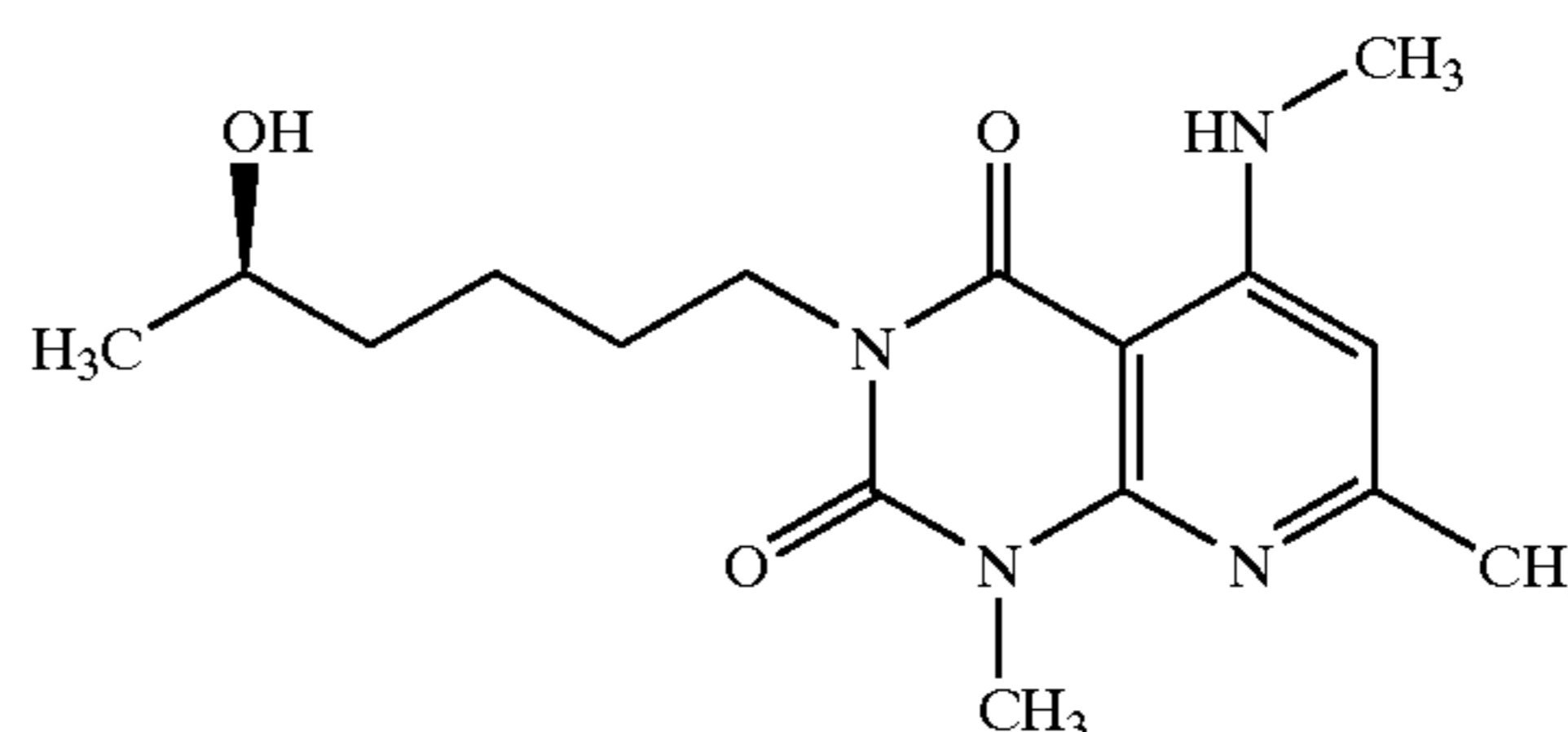
(R)-1,7-Dimethyl-3-(5-hydroxyhexyl)-5-(N-methylamino)pyrido[2,3-d]pyrimidine-2,4(1H,3H)-dione (CT-30102)
