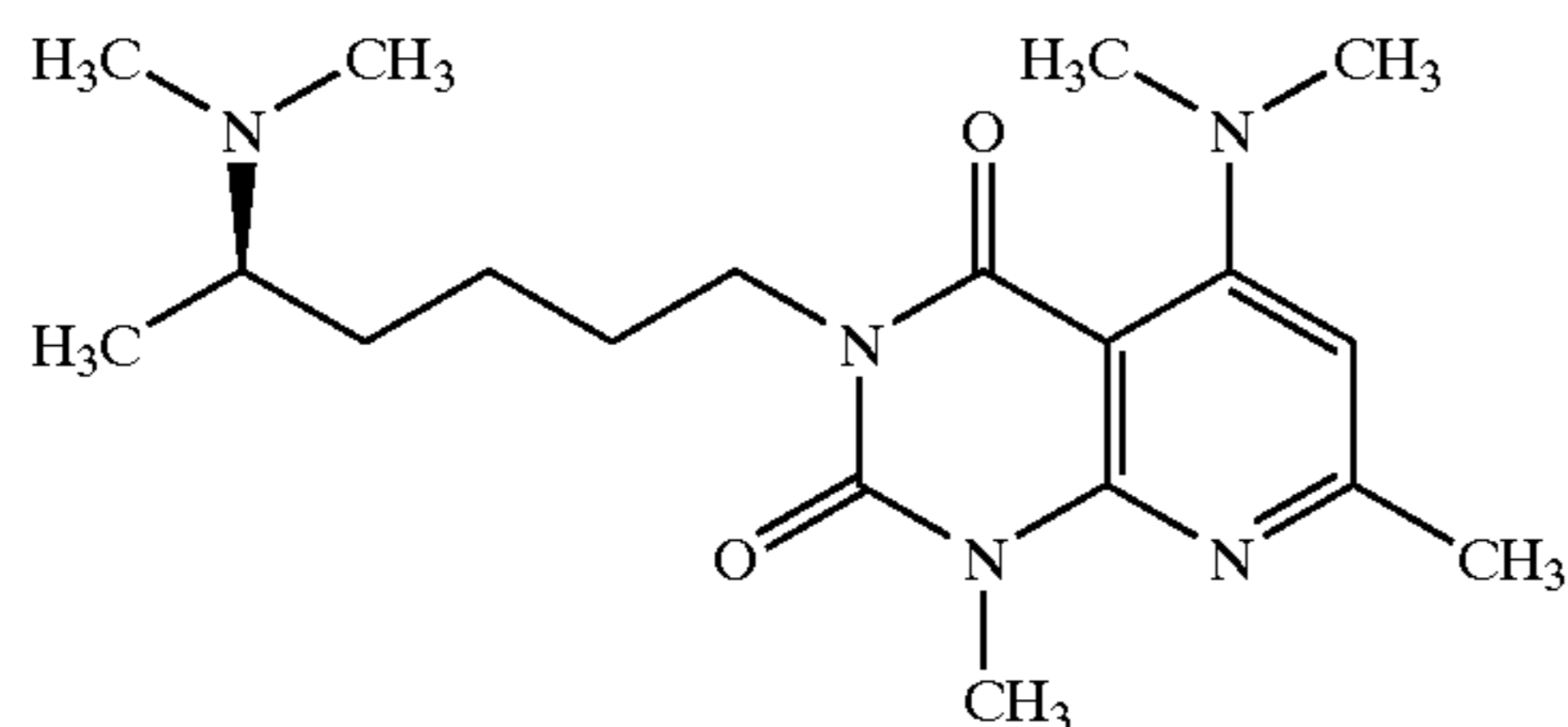
(R)-1,7-Dimethyl-5-(N,N-dimethylamino)-3-(5-(N,N-dimethylamino)hexyl)pyrido[2,3-d]pyrimidine-2,4(1H,3H)dione (CT-31818)
