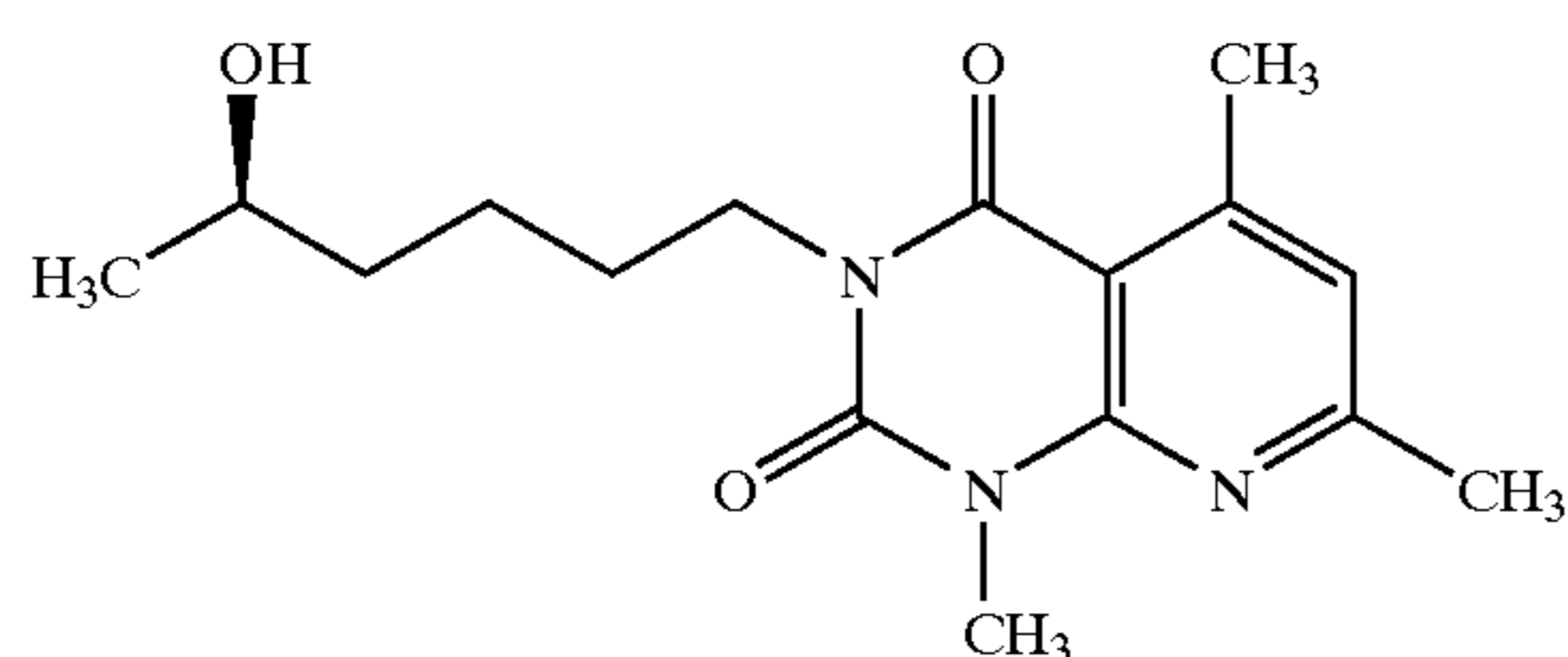
(R)-3-(5-Hydroxyhexyl)-1,5,7-trimethylpyrido[2,3-d]pyrimidine-2,4(1H,3H)-dione (CT-30144)
