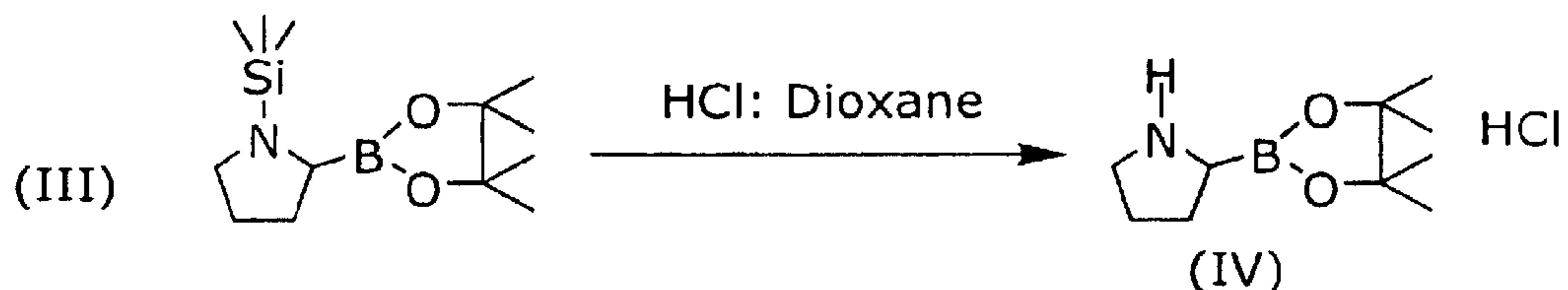
1-trimethylsilyl-boroProline pinacol boroProline-pinacol-HCl
