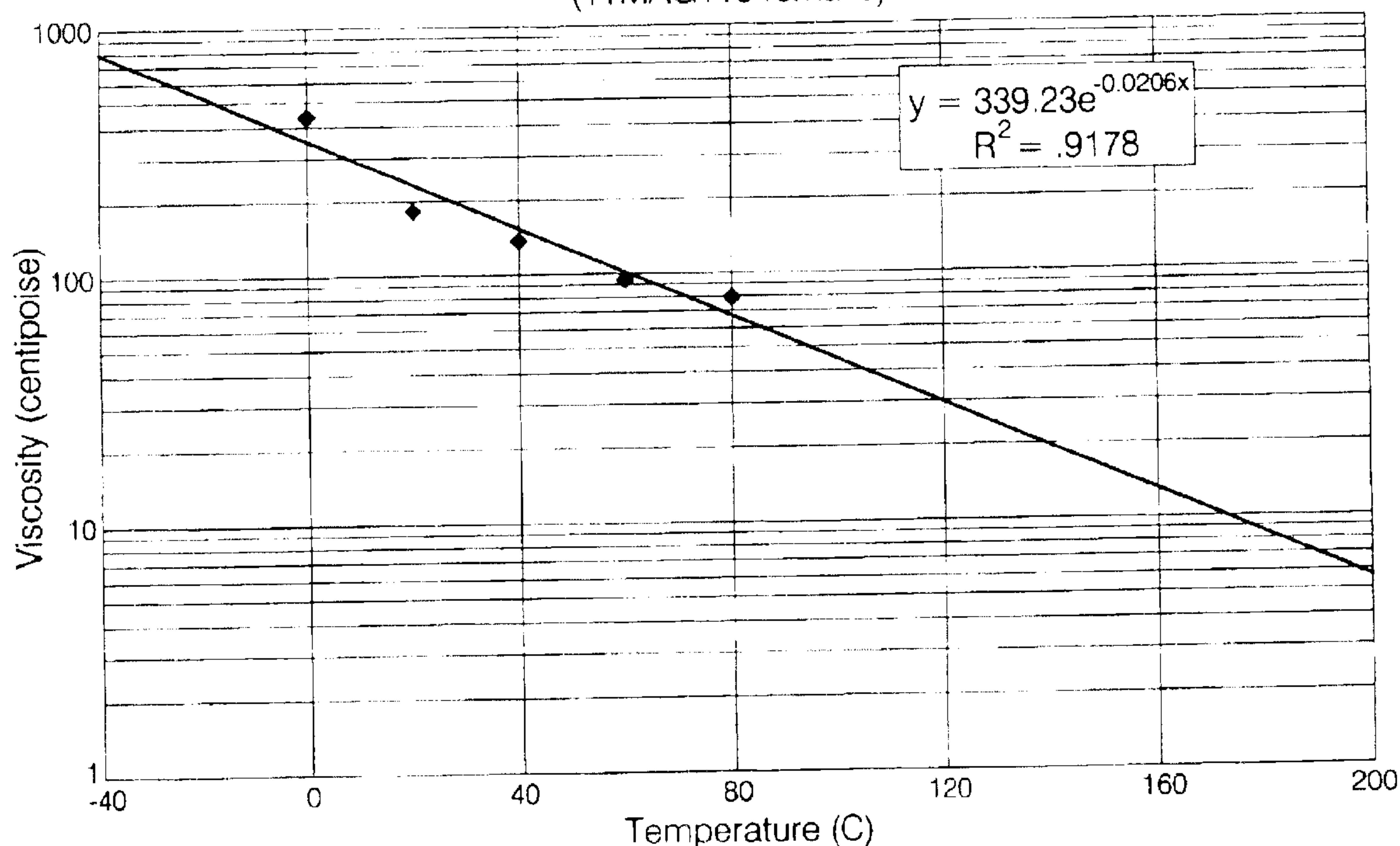
Viscosity versus Temperature for 12MAG001 (11MAG115 remake)
