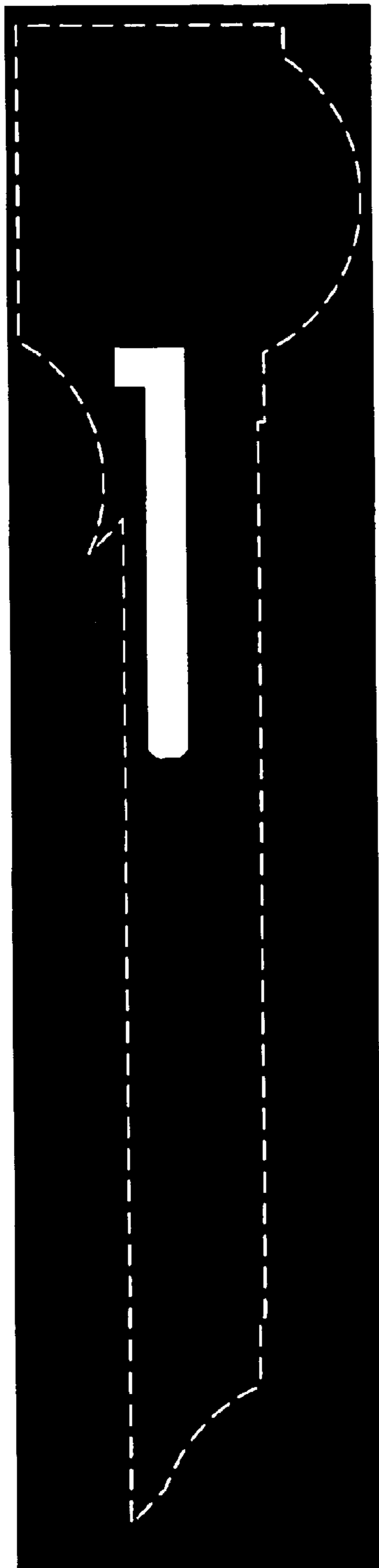
N-Well mask
