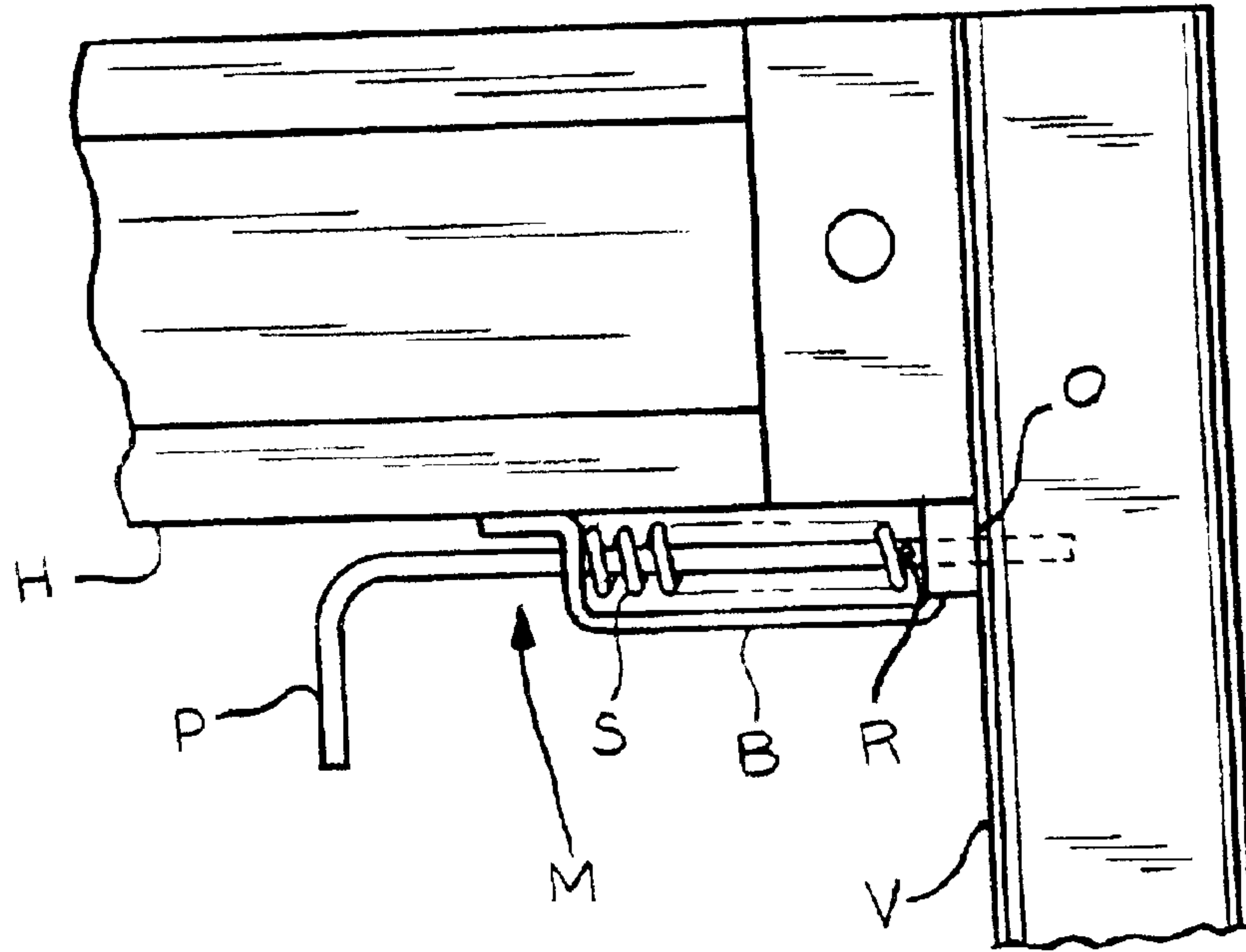
FIG. 6 PRIOR ART
