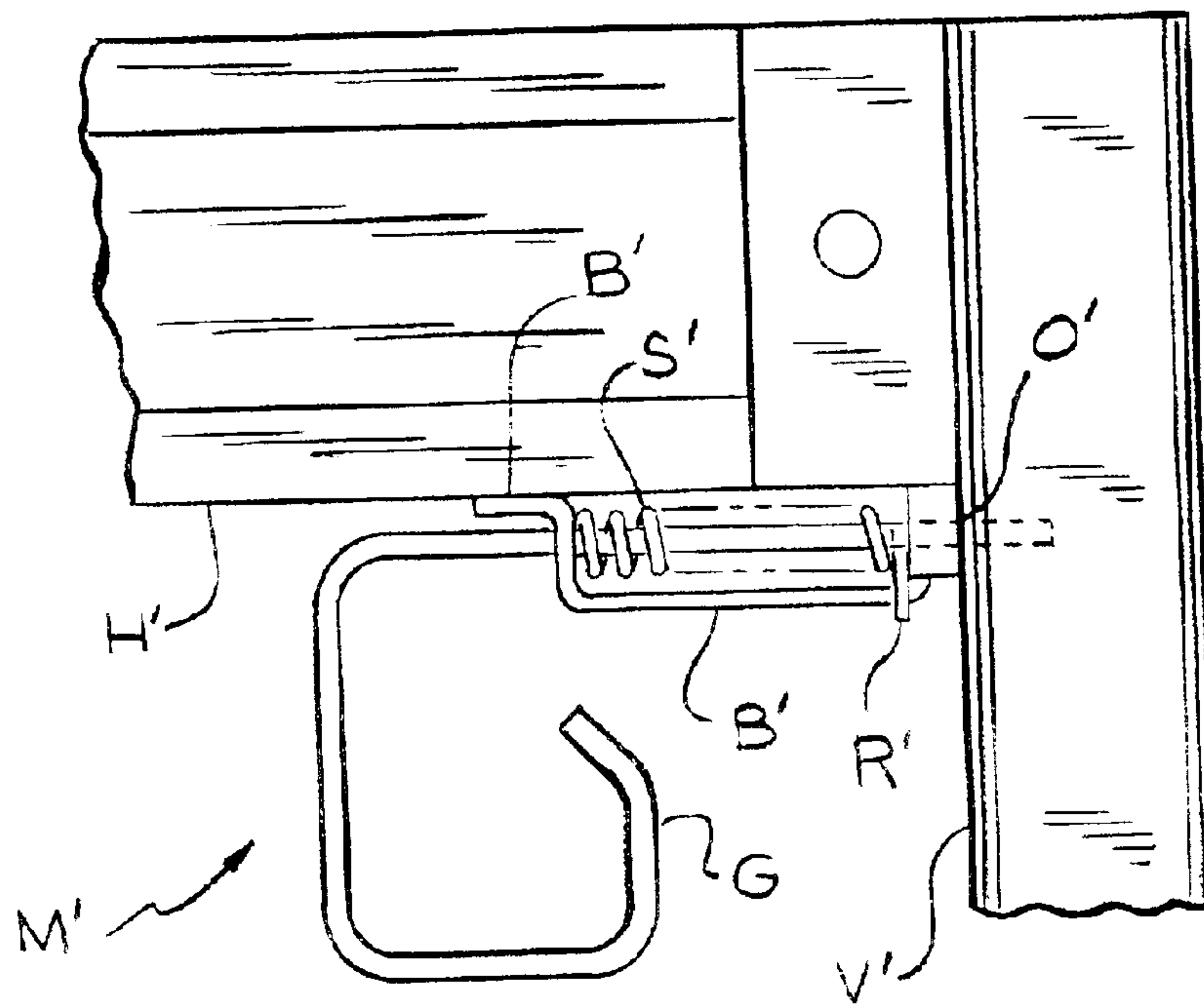
FIG. 7 PRIOR ART
