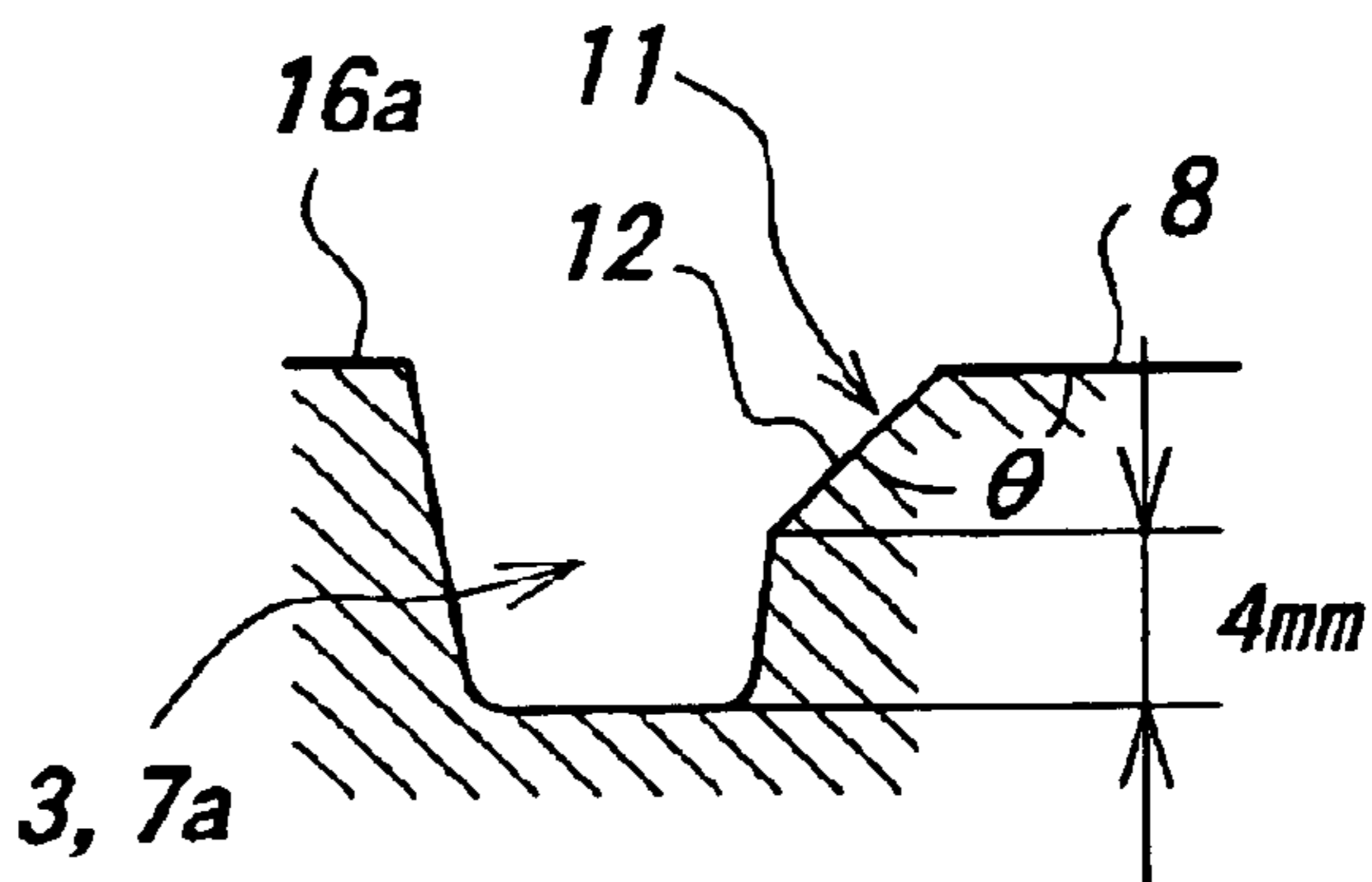
FIG. 9b II-II section
