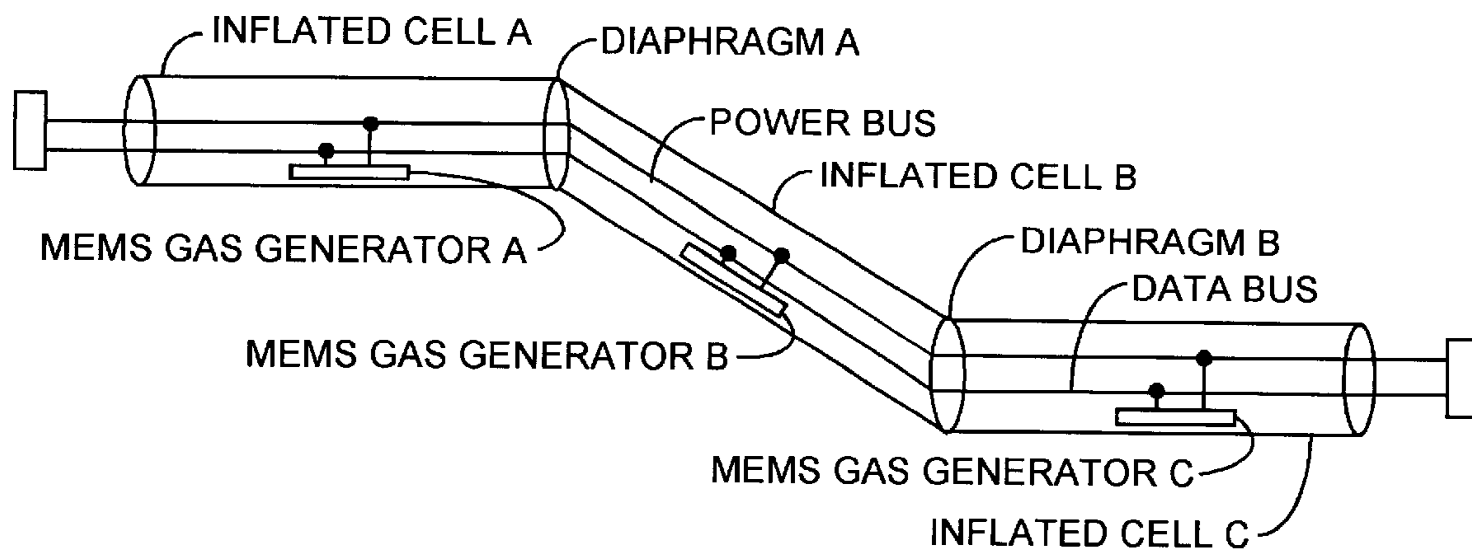
INFLATED INFLATABLE STRUCTURE
