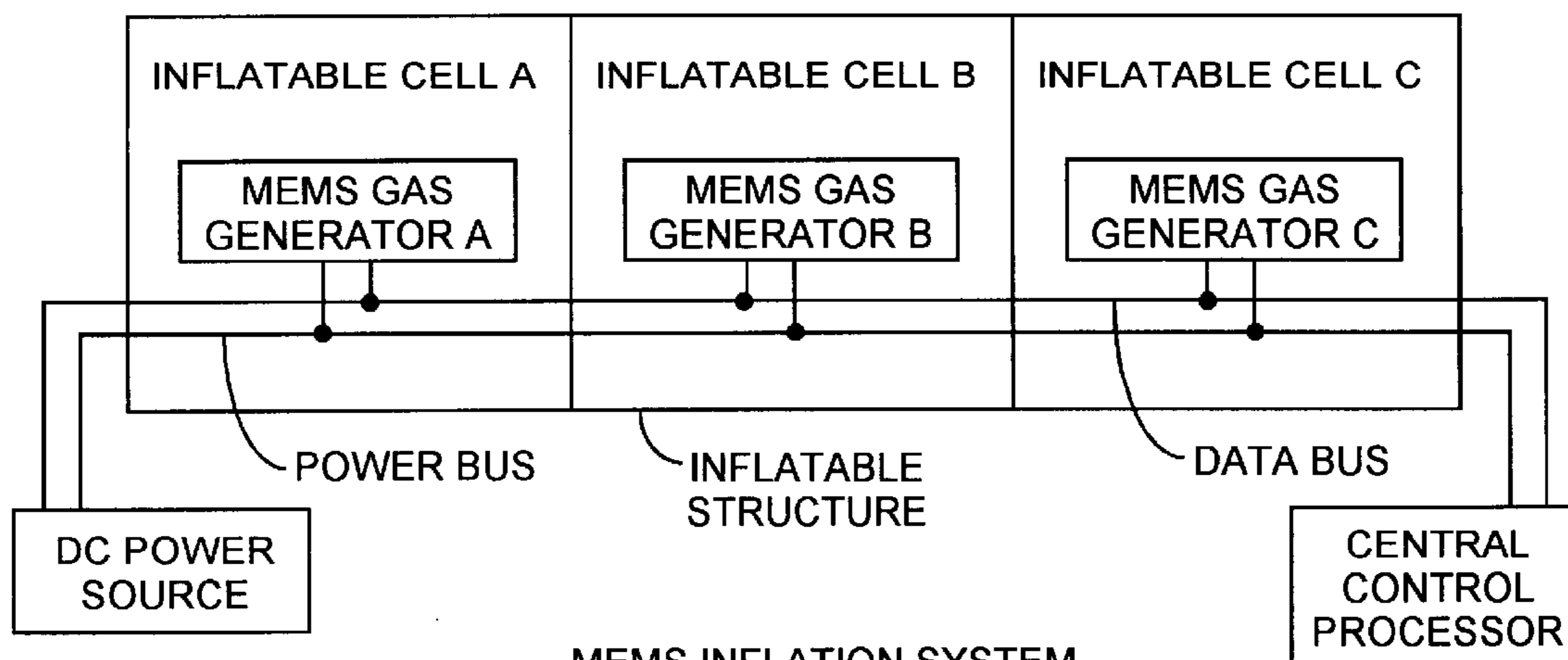
MEMS INFLATION SYSTEM FIG. 1
