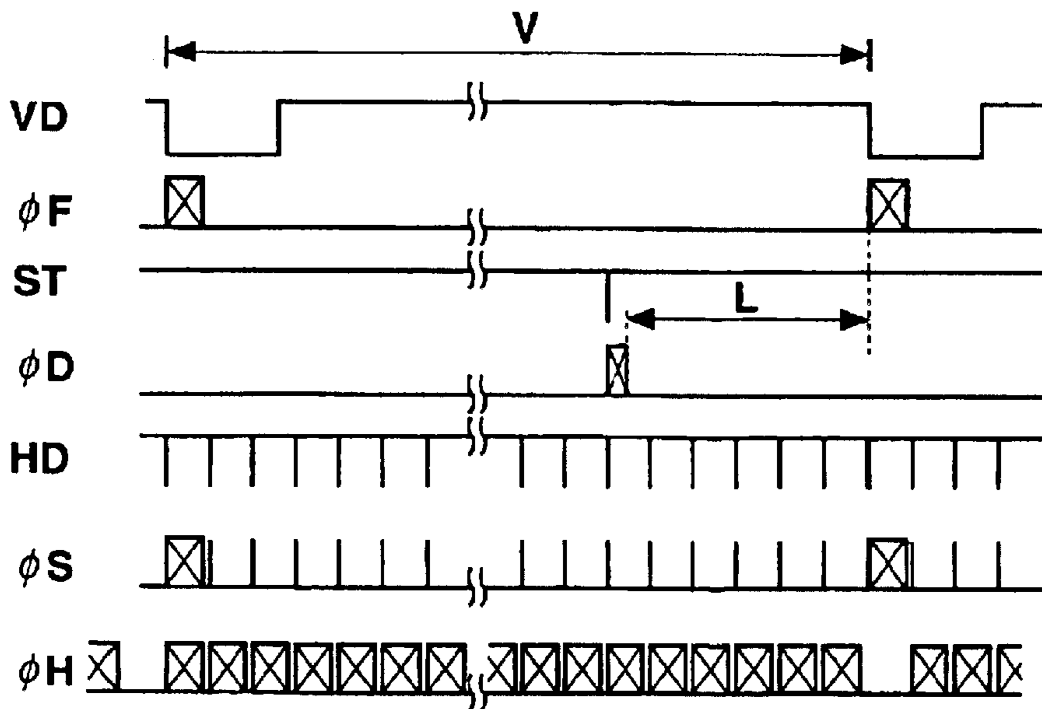
Fig. 2 PRIOR ART
