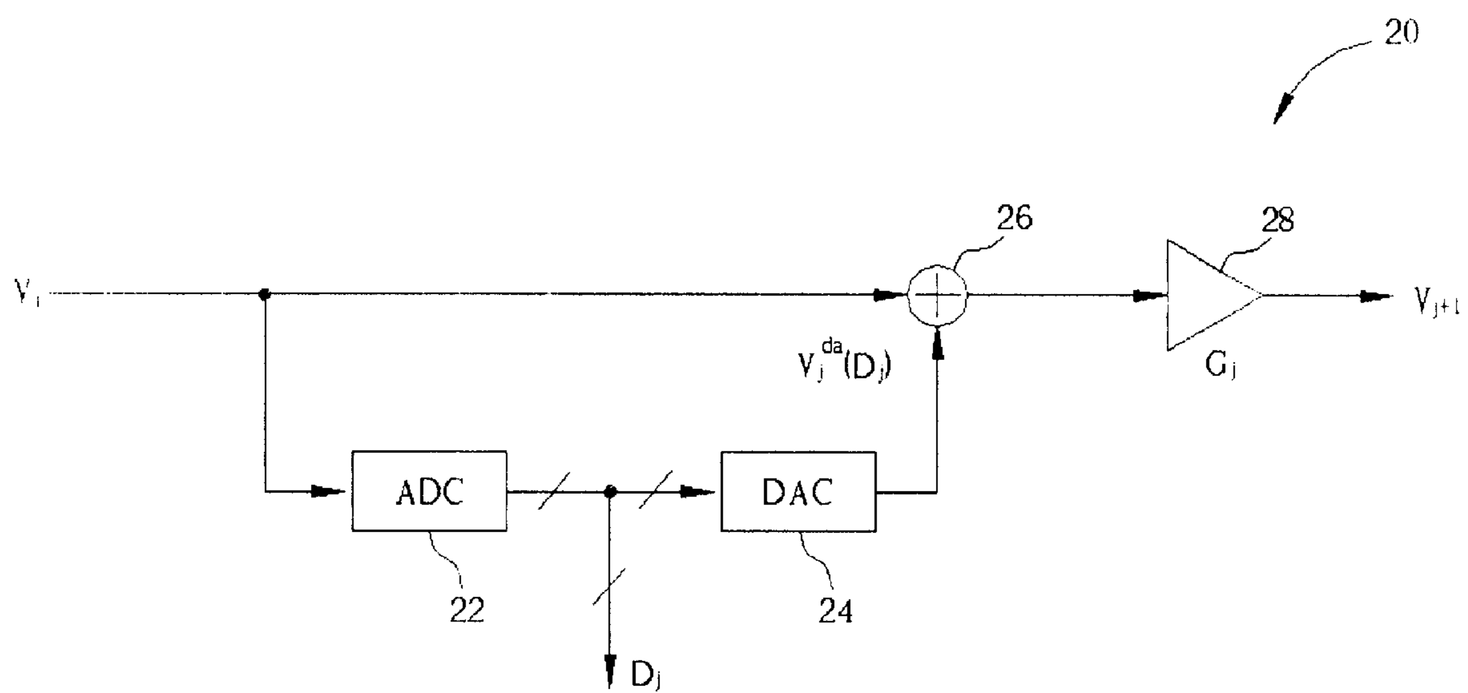
Fig. 2 Prior Art
