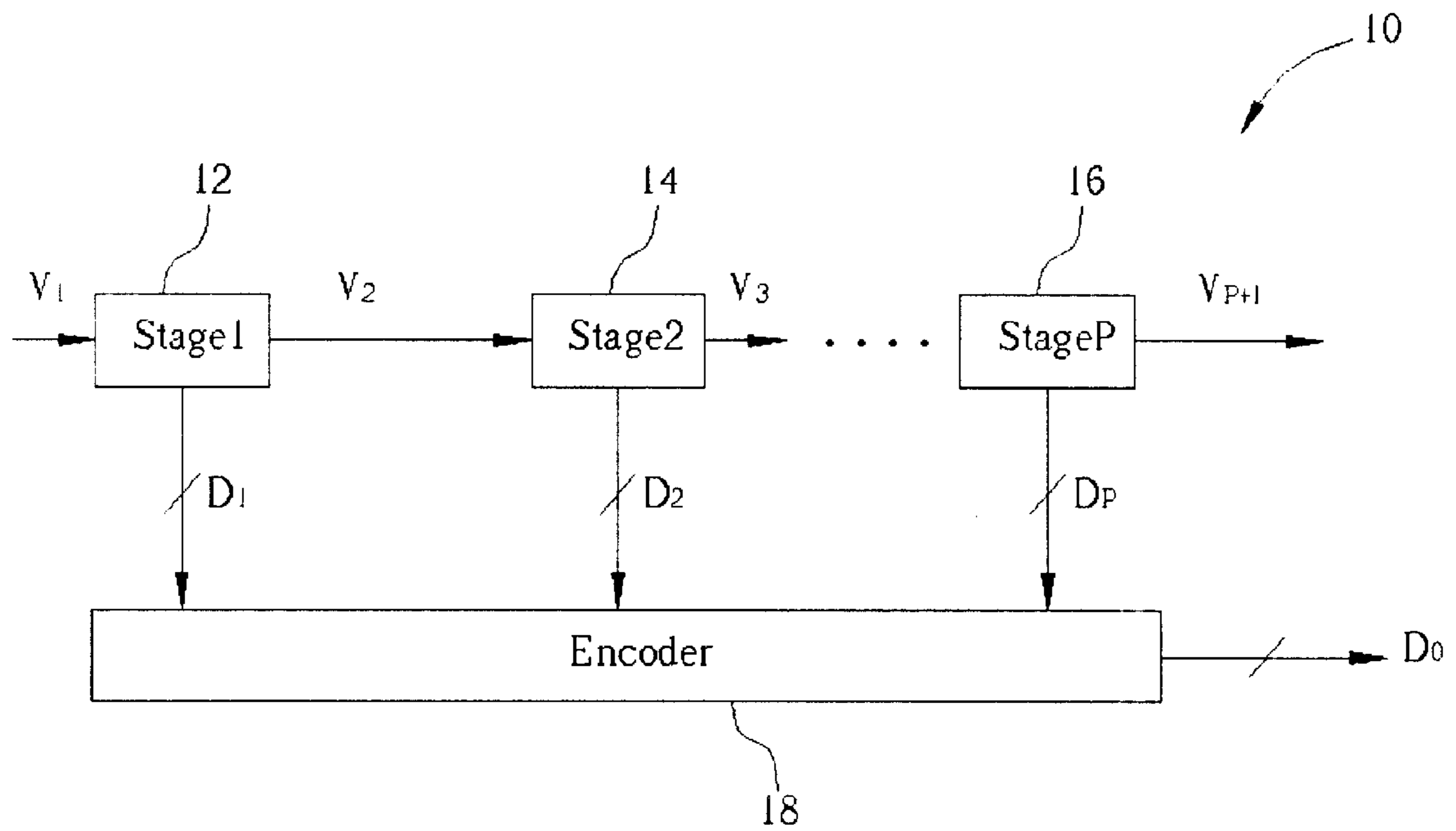
Fig. 1 Prior Art
