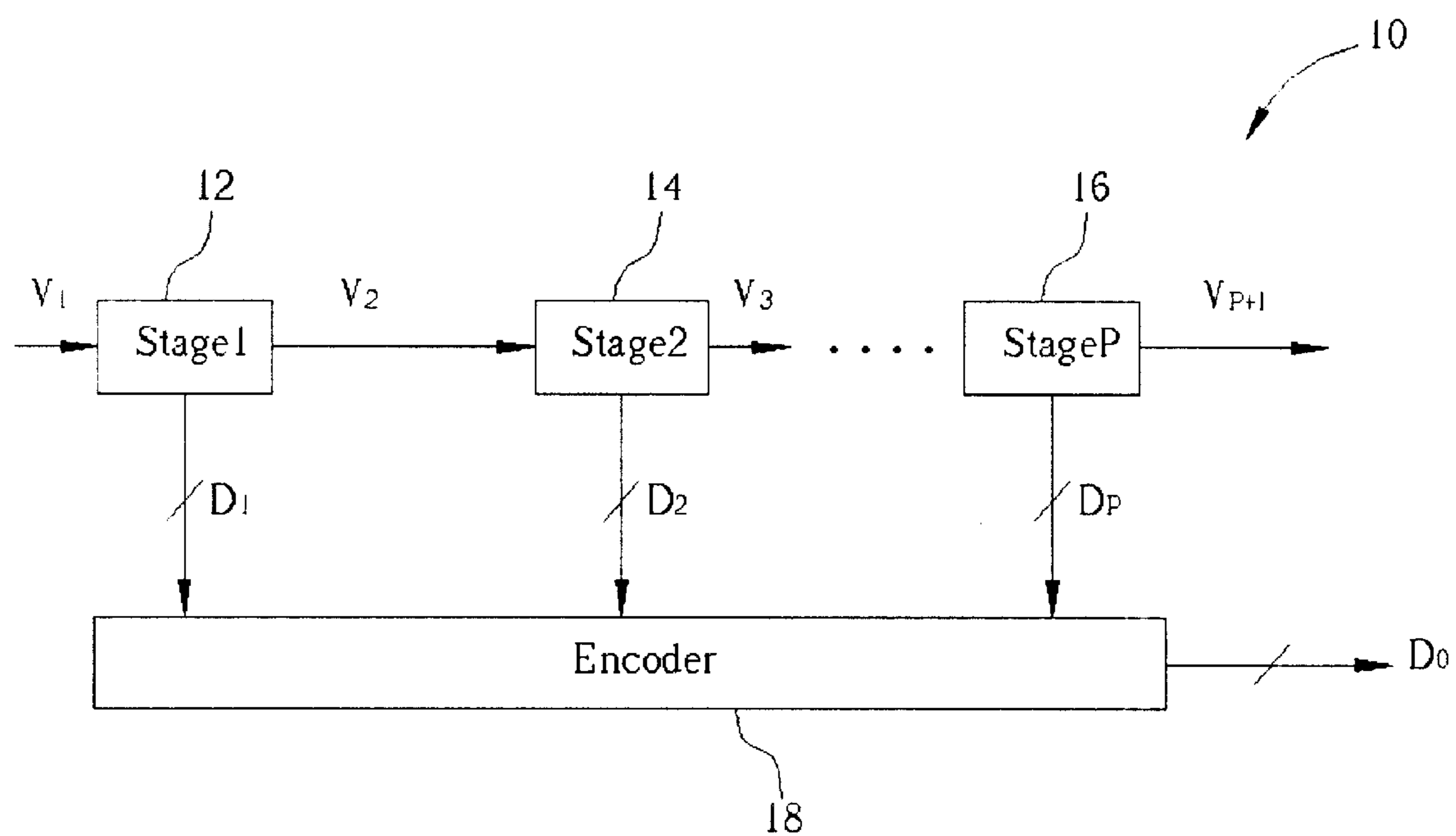
Fig. 1 Prior Art
