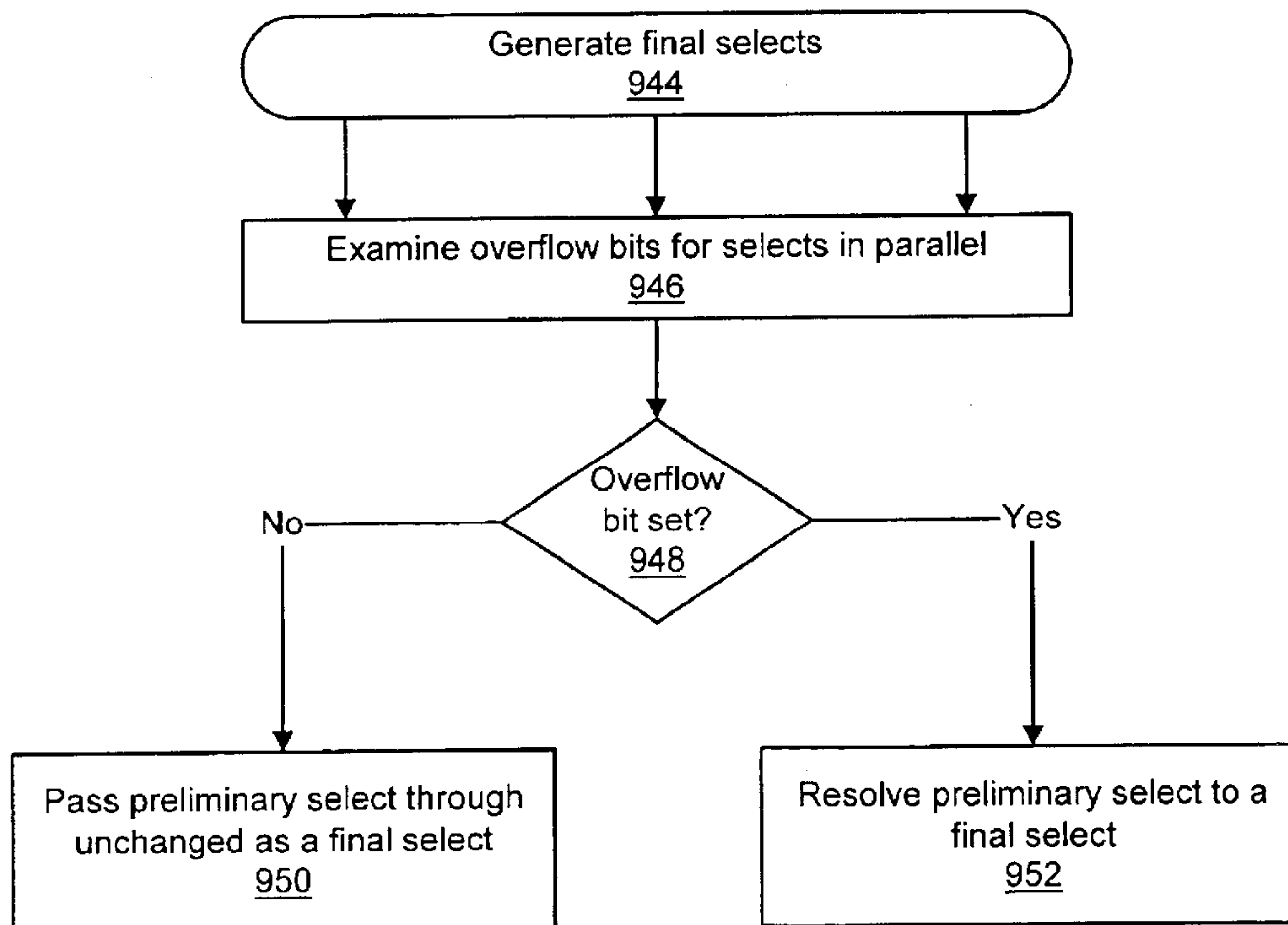
Figure 43h Decompression flowchart
