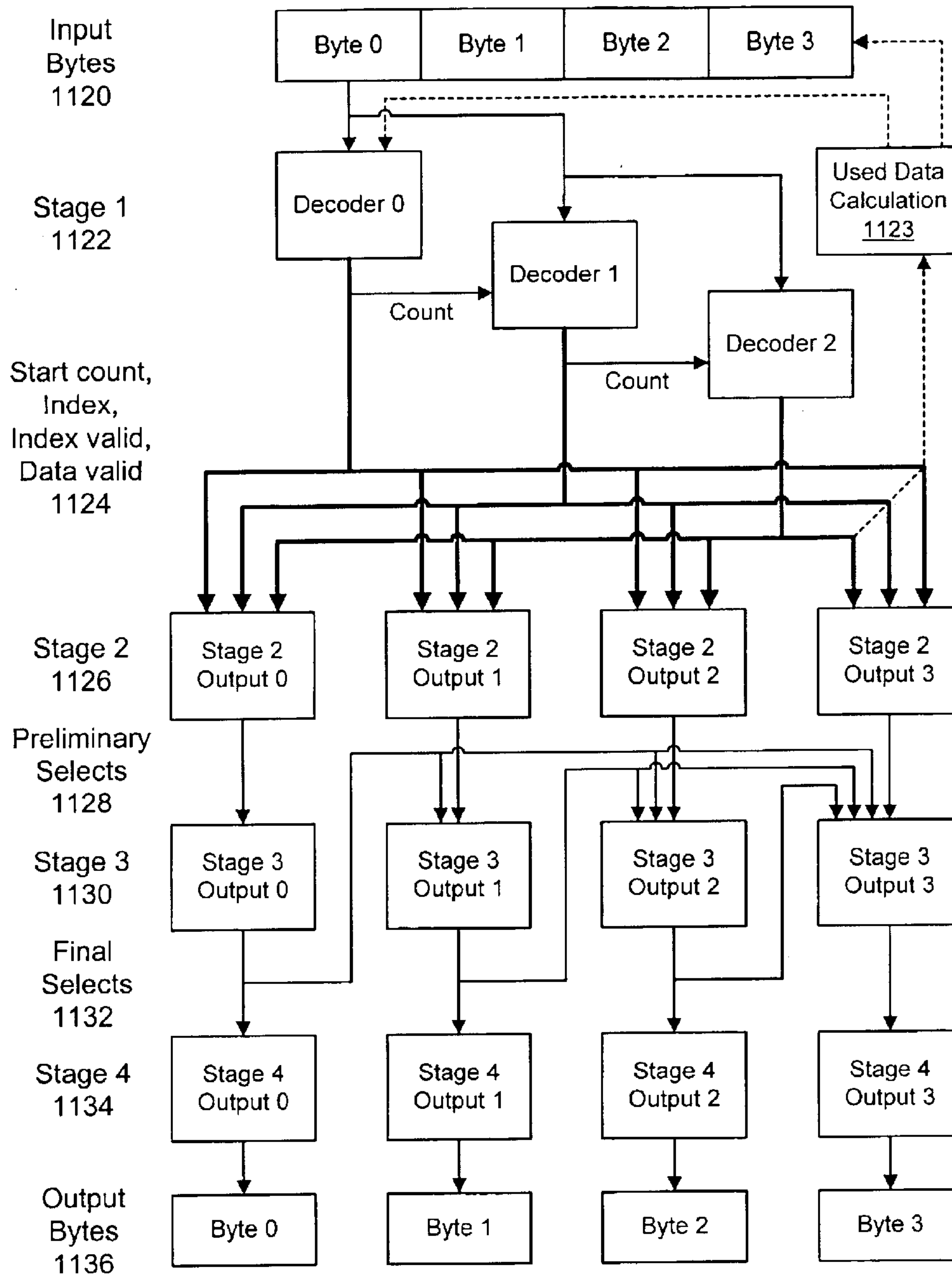
Figure 42a - 4 input bytes, 3 decoders, 4 output bytes
