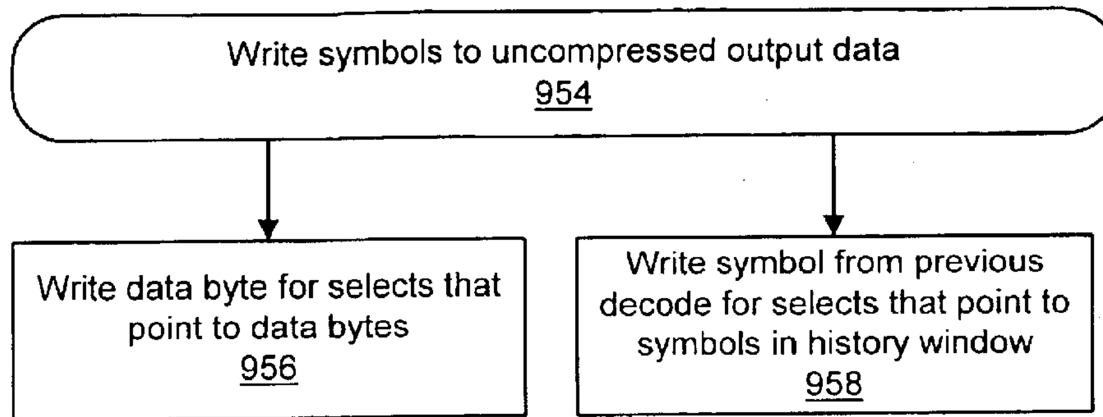
Figure 43i Decompression flowchart
