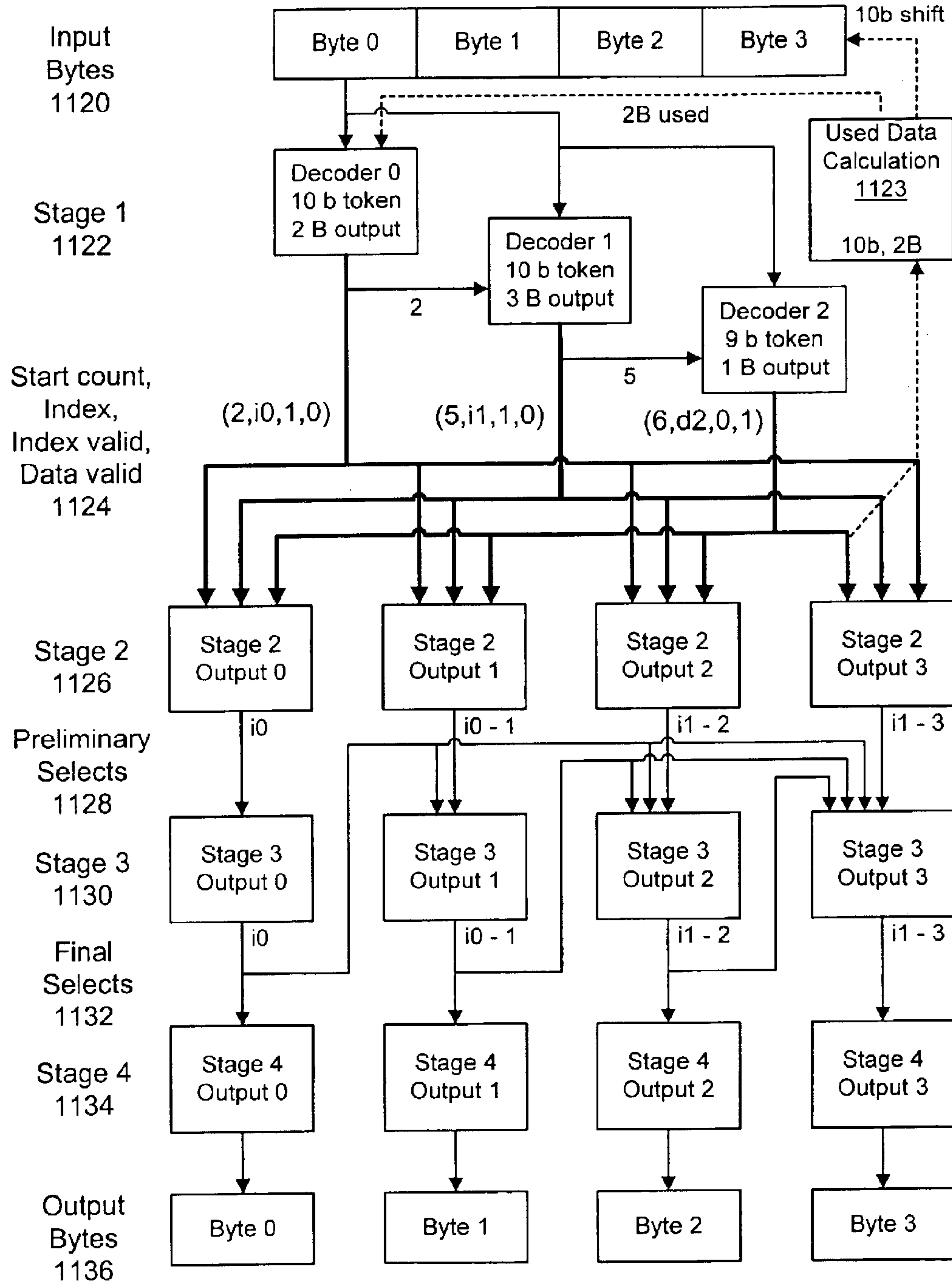
Figure 42b - example using 4 input bytes, 3 decoders, 4 output bytes
