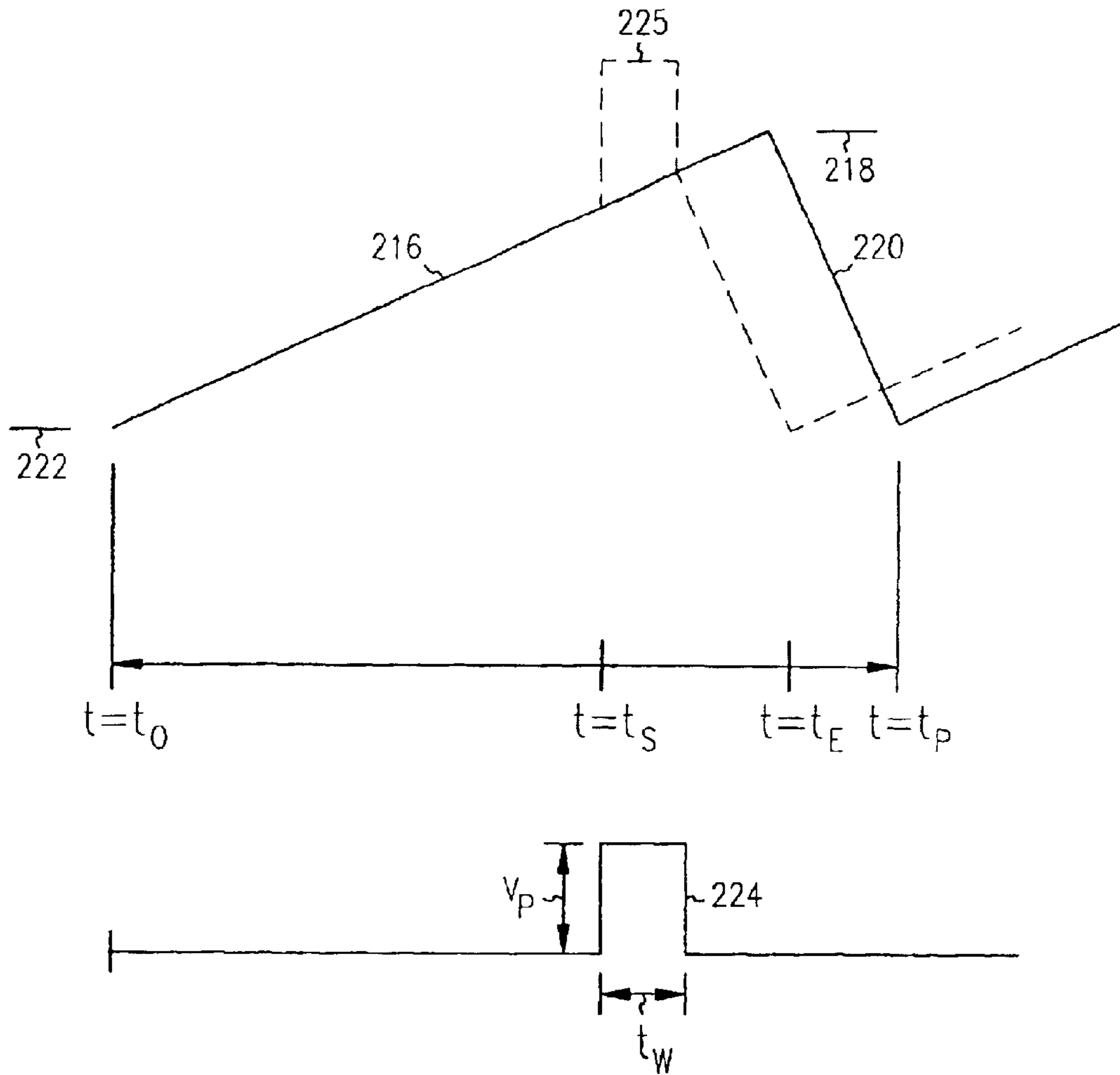
FIG. 2 (PRIOR ART)
