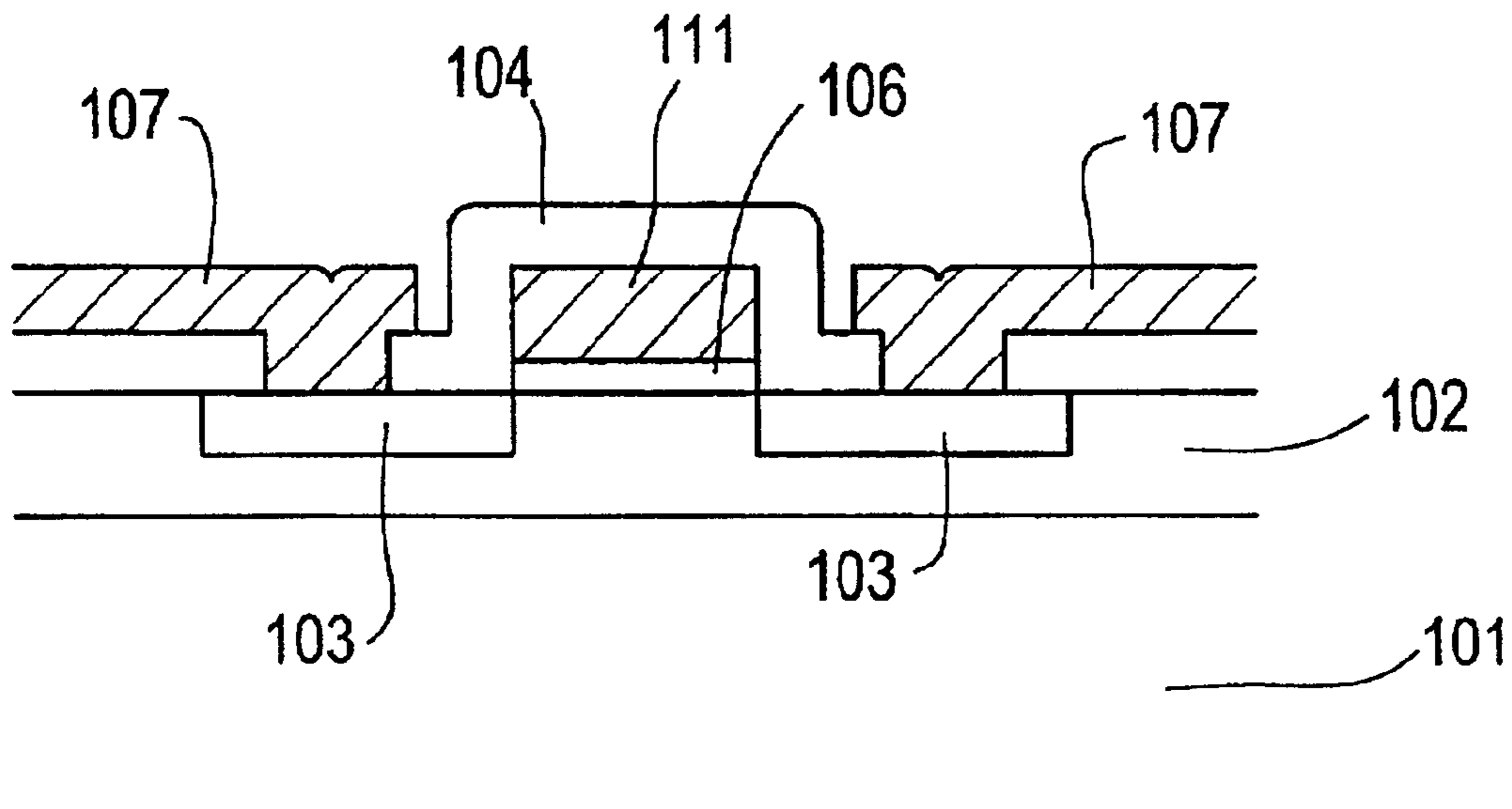
FIG. 6 PRIOR ART
