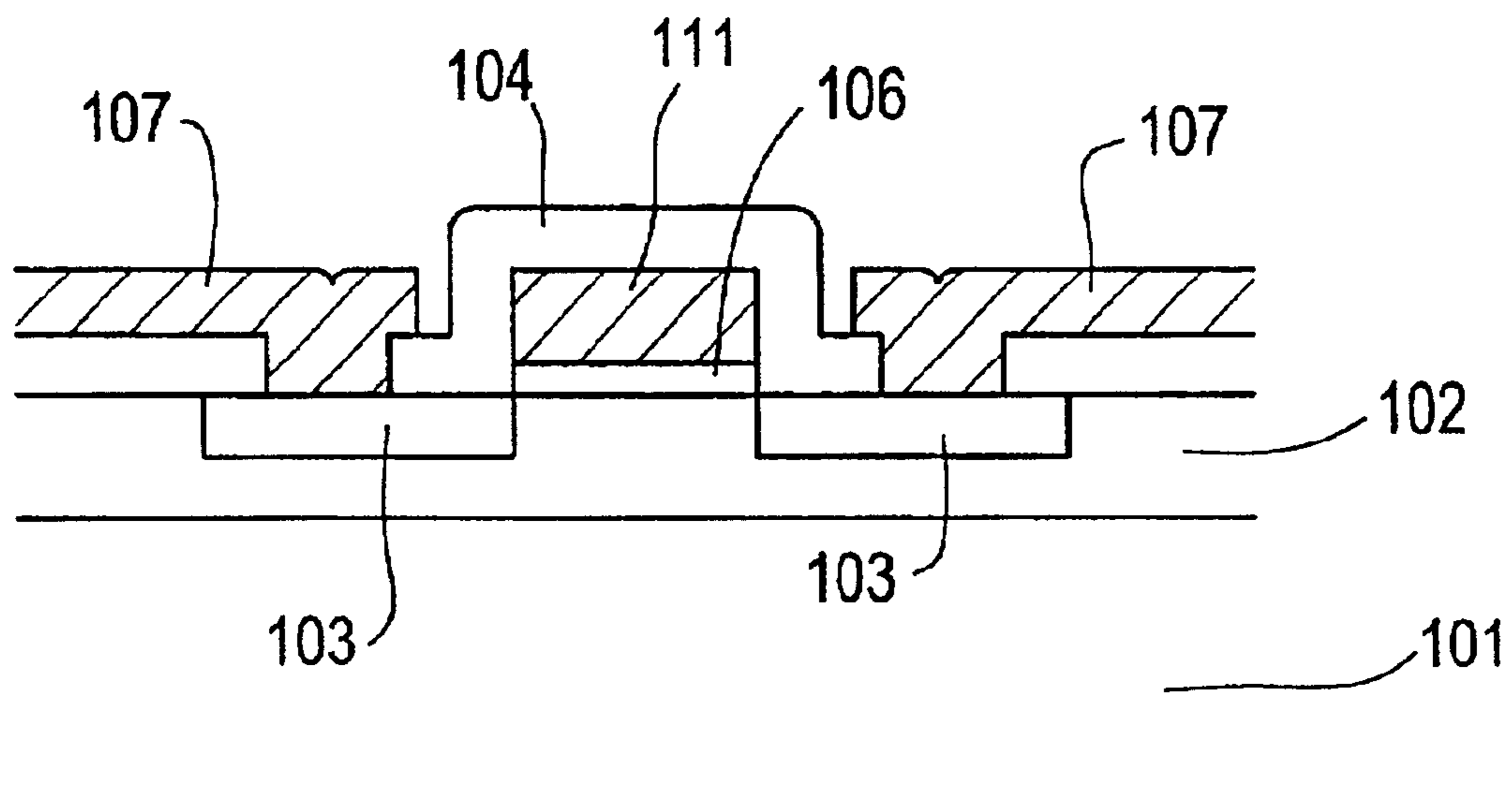
FIG. 6 PRIOR ART
