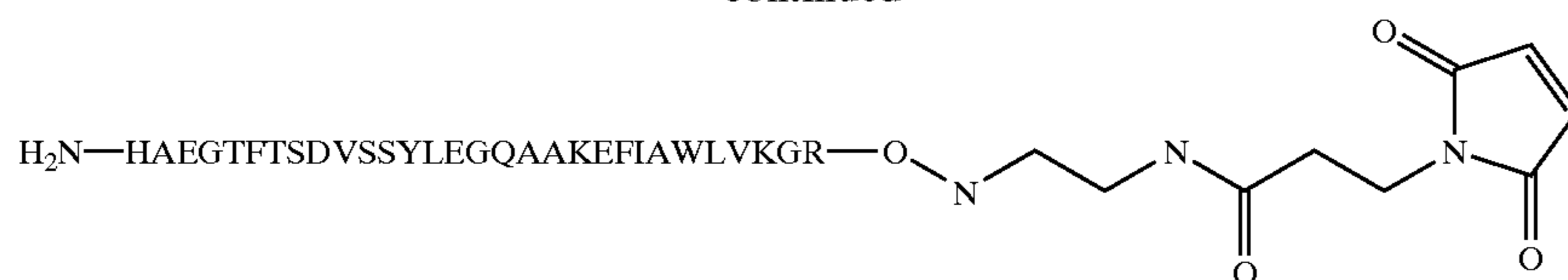
GLP-1 (7-36)-EDA-MPA
