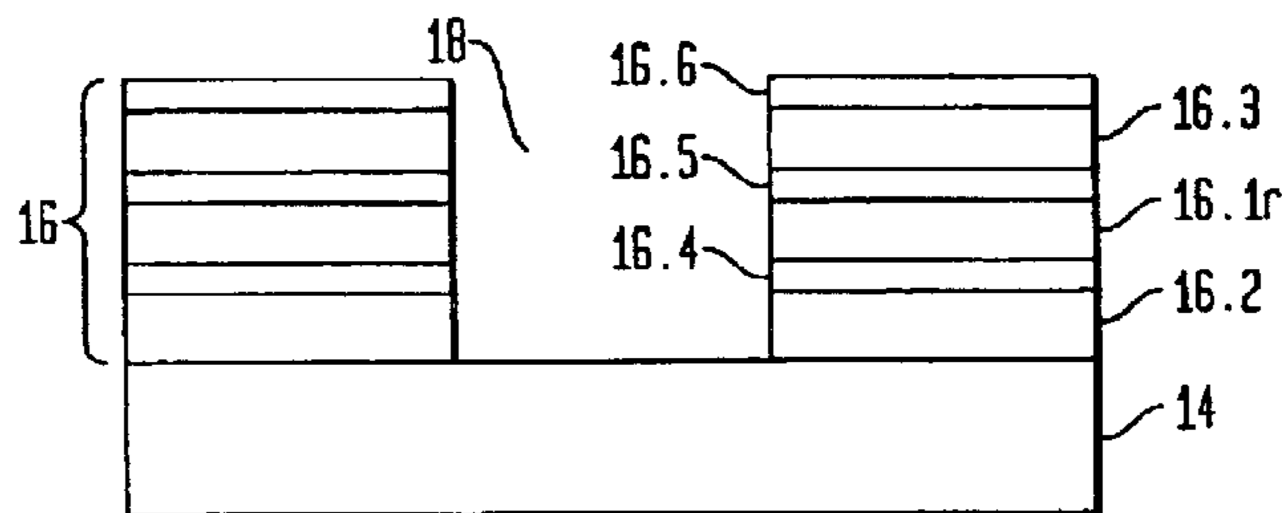
FIG. 2 (PRIOR ART)
