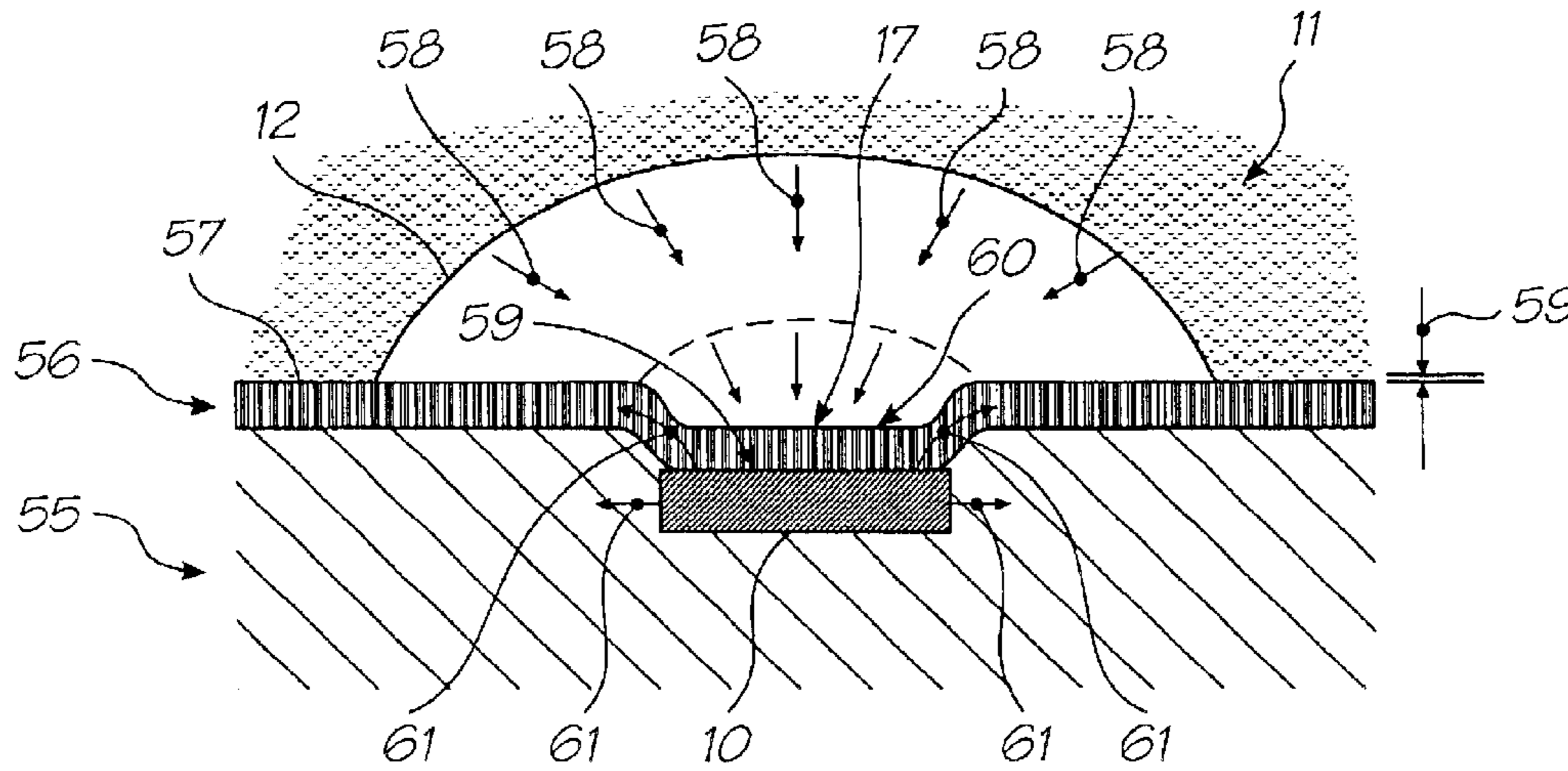
FIG. 47 (PRIOR ART)
