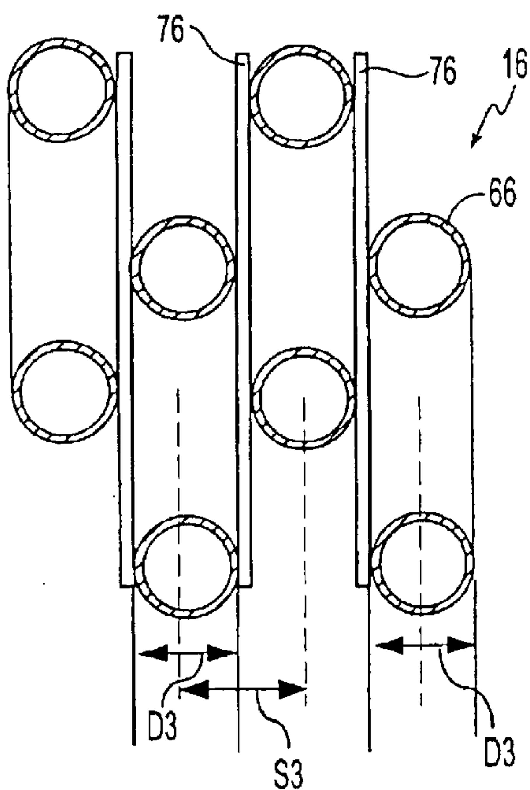
FIG. 7 PRIOR ART
