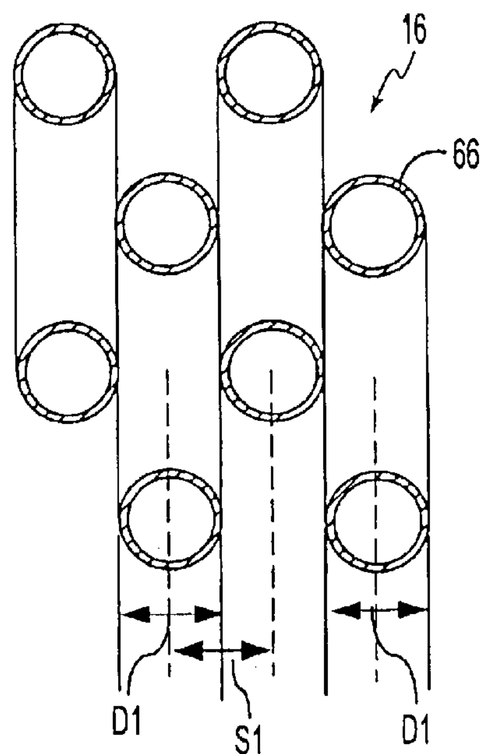
FIG. 5 PRIOR ART
