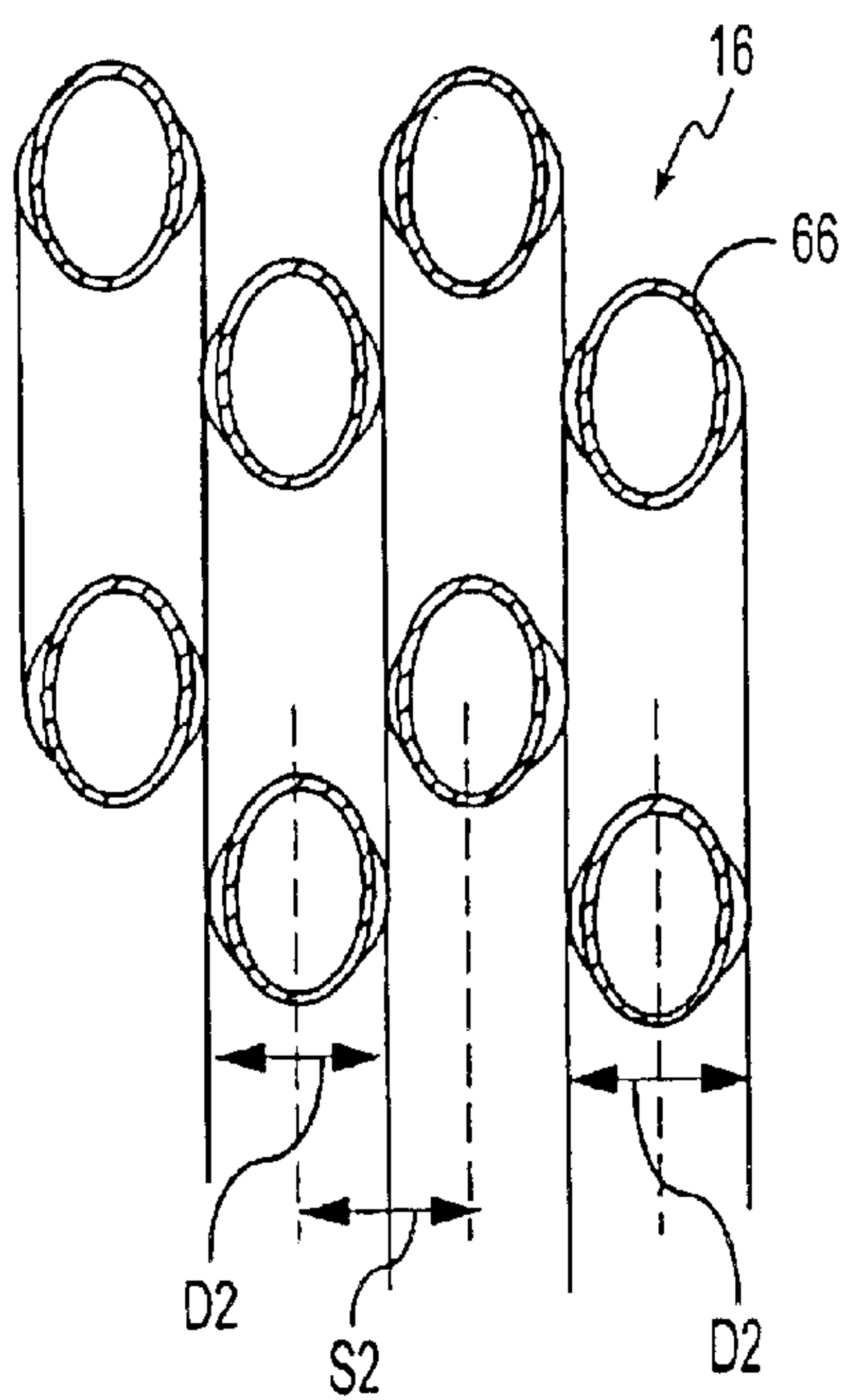
FIG. 6 PRIOR ART
