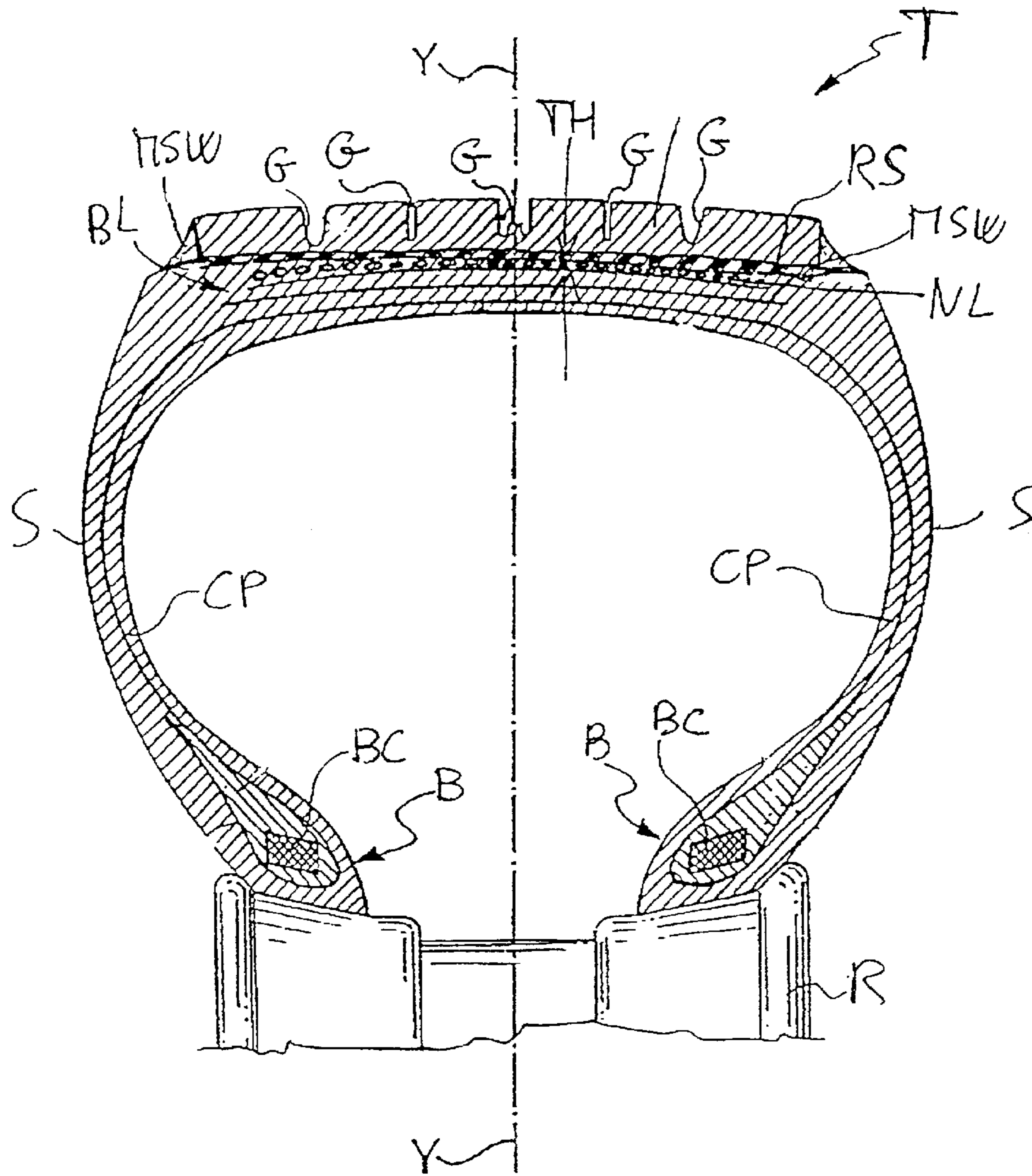
FIG. 1 PRIOR ART
