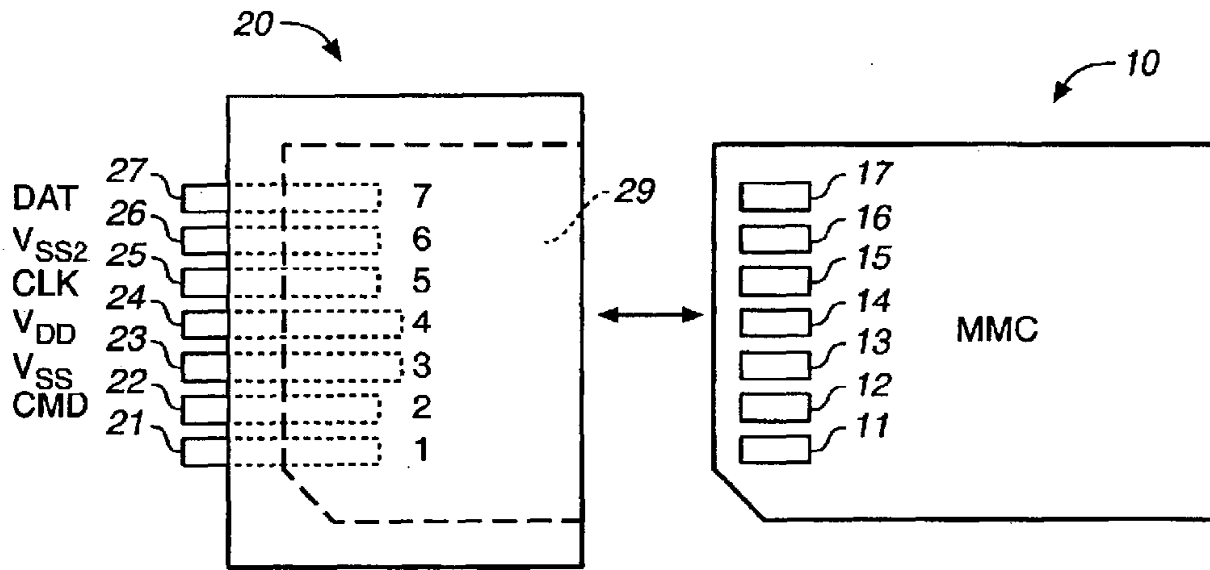
FIG. 1 (PRIOR ART)
