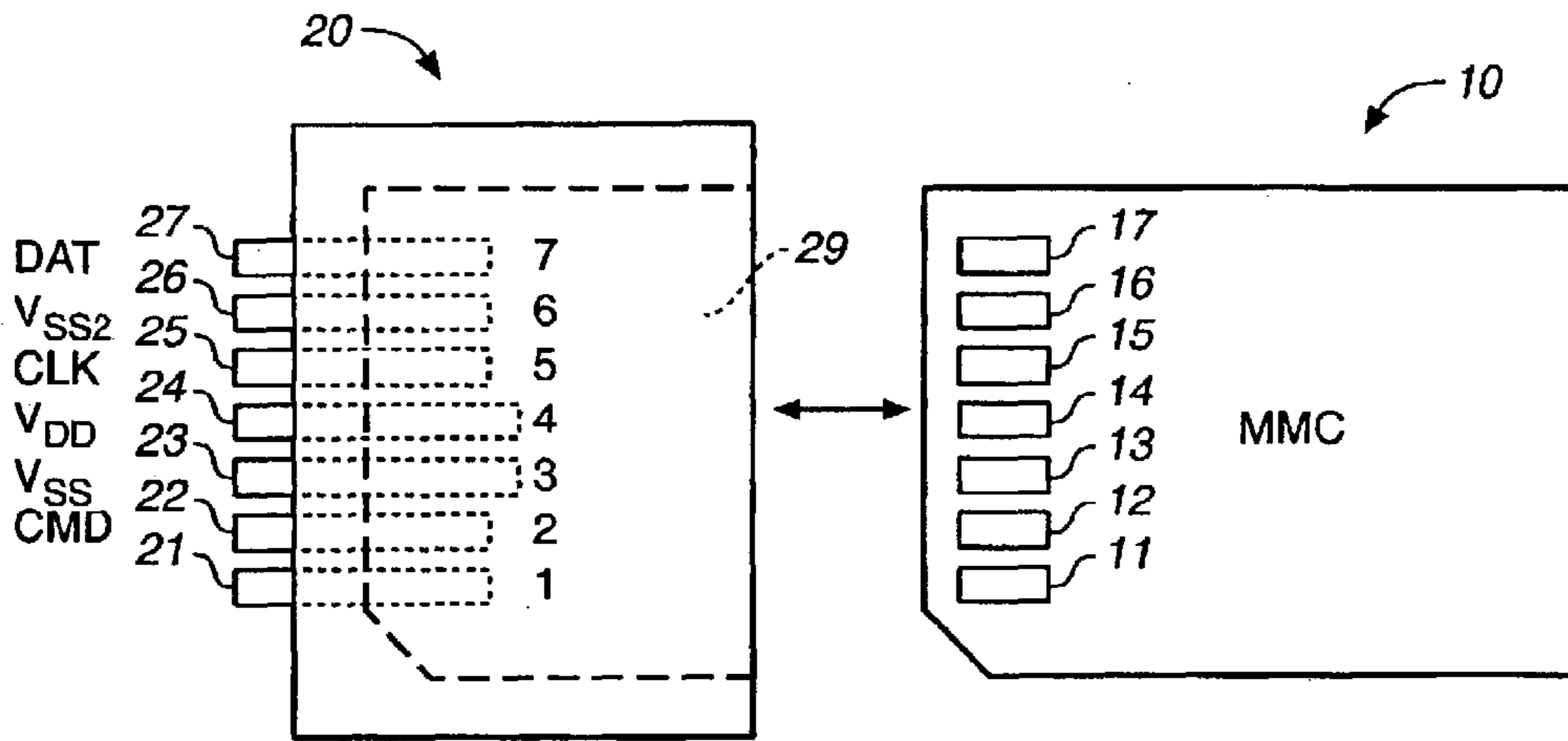
FIG. 1 (PRIOR ART)
