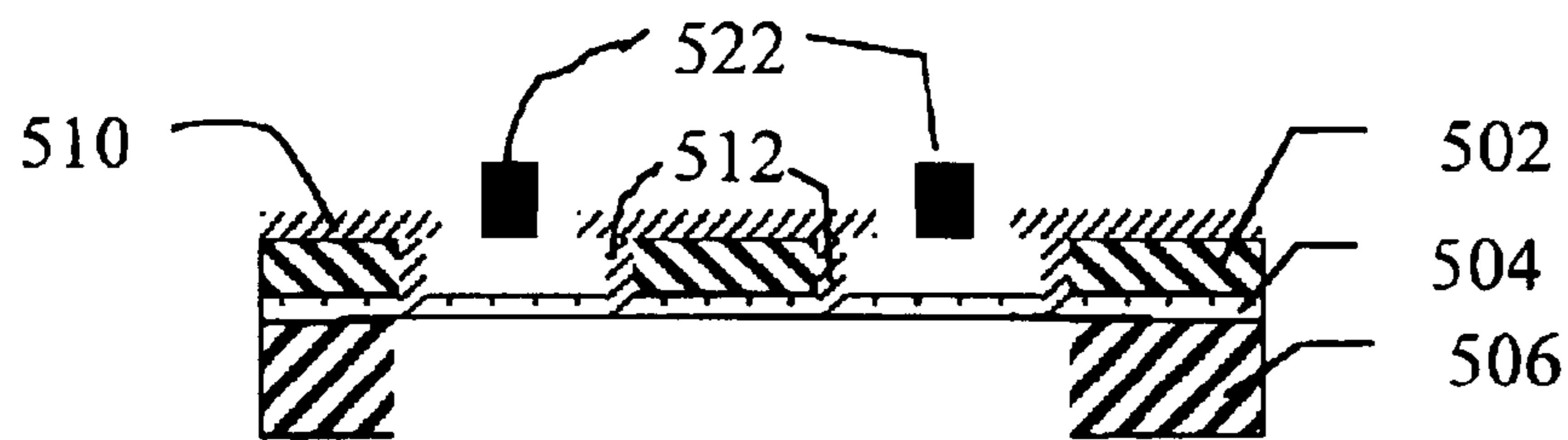
Formation of backside cavity
