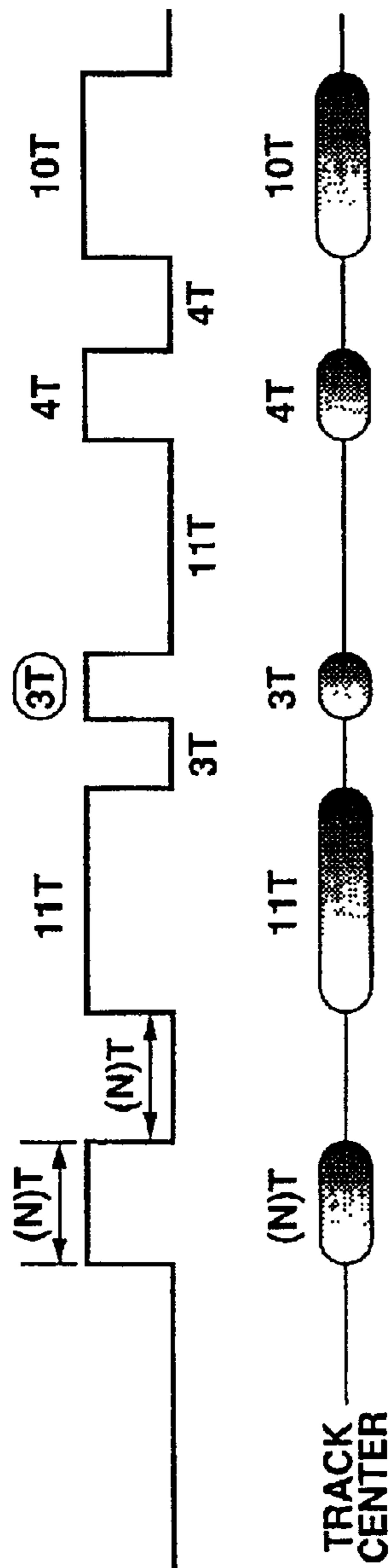
FIG.3A EFM DATA
