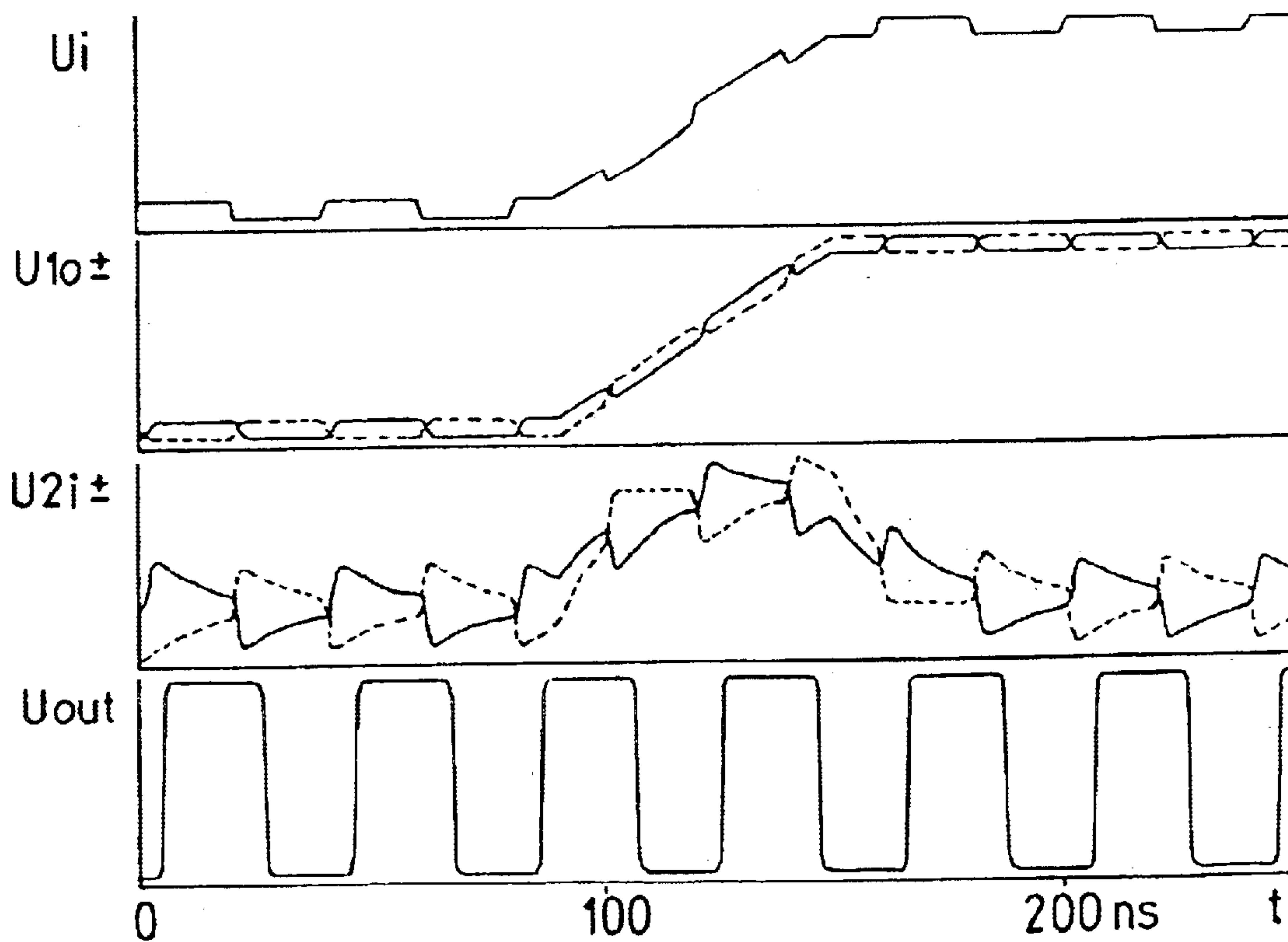
Fig. 2 (PRIOR ART)
