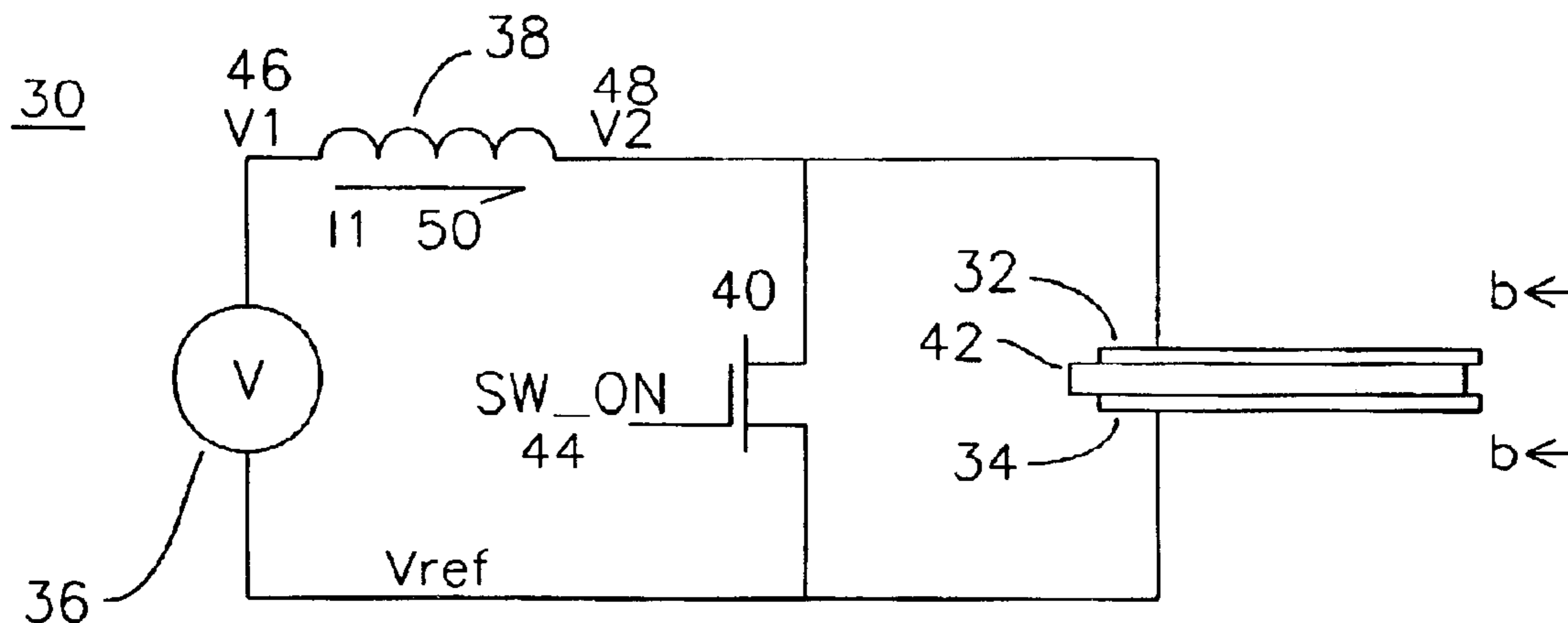
Low Voltage Pulsed Plasma Thruster
