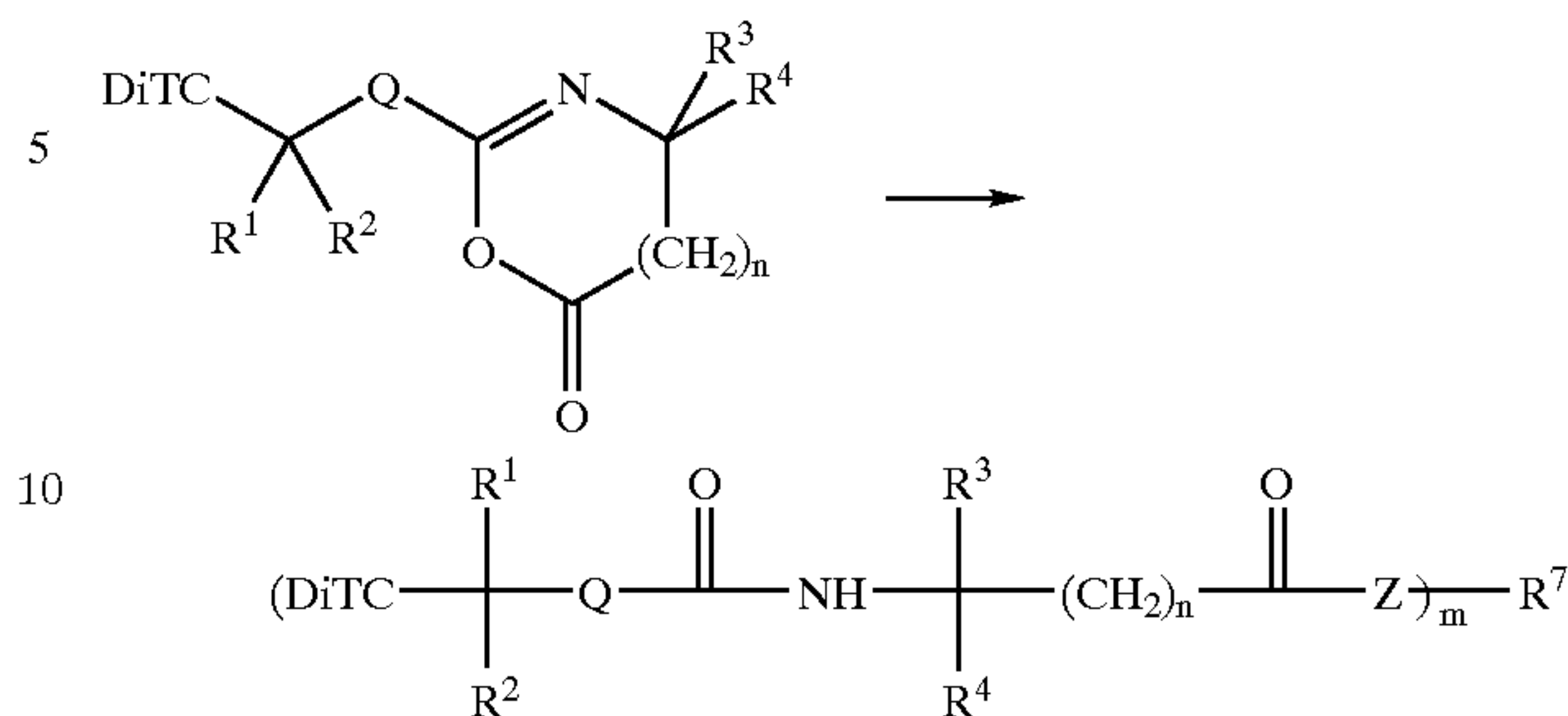
Scheme II
