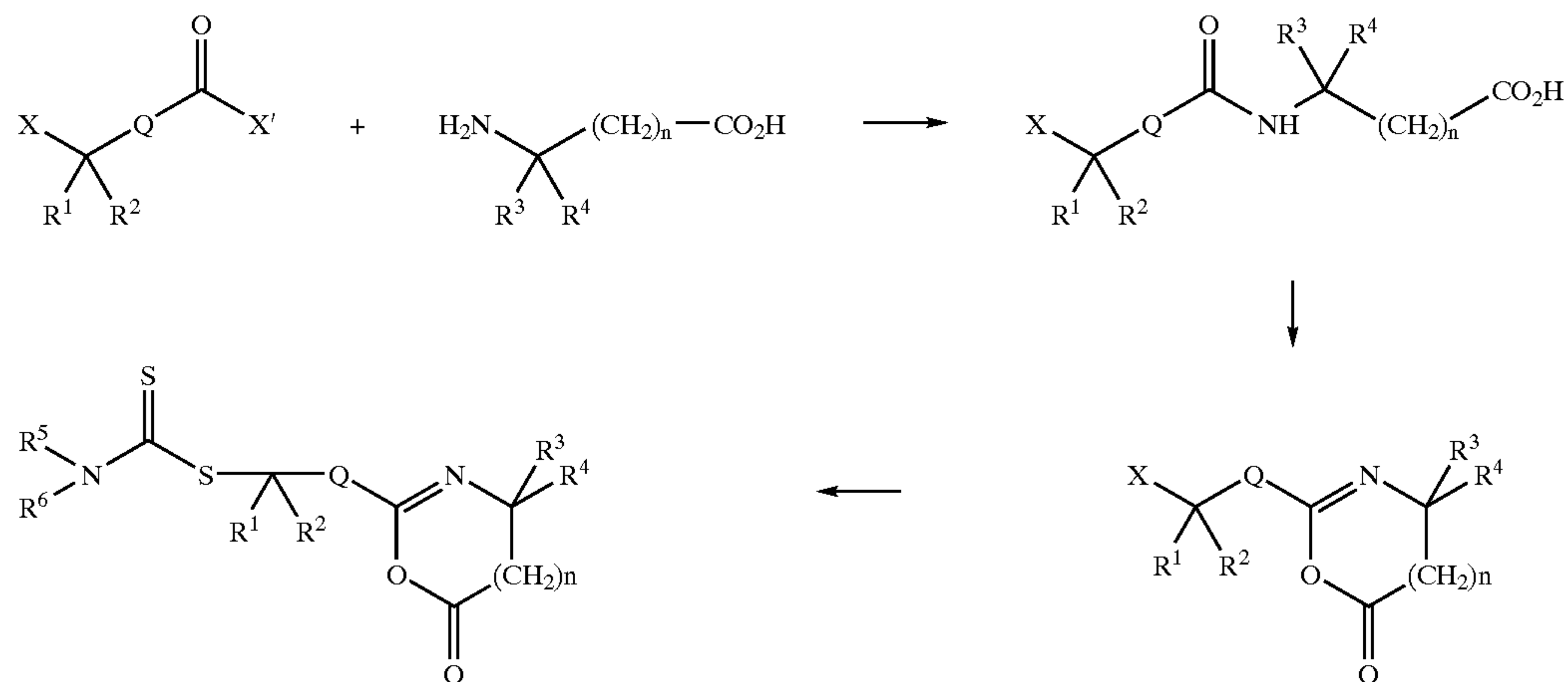
Scheme I
