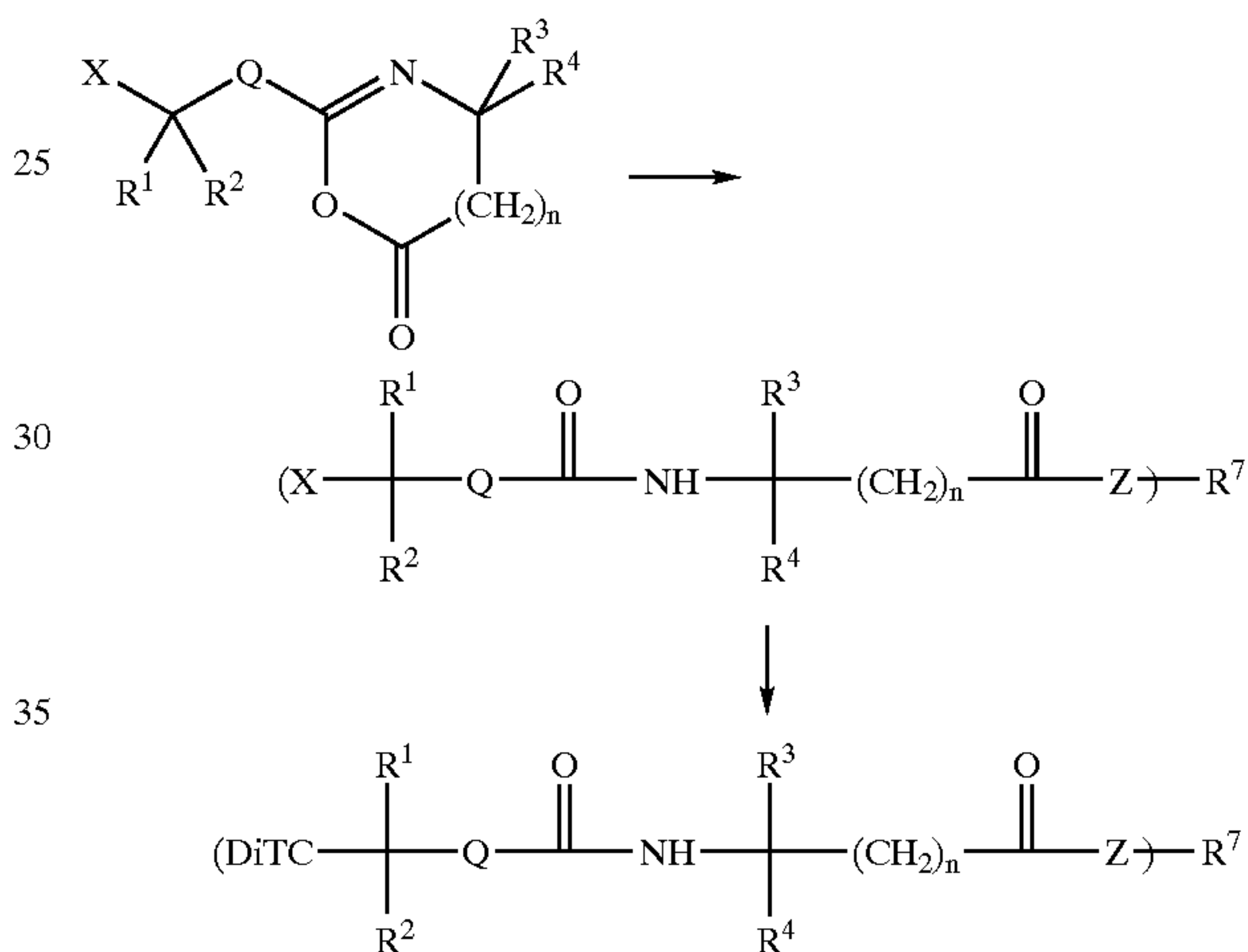
Scheme III
