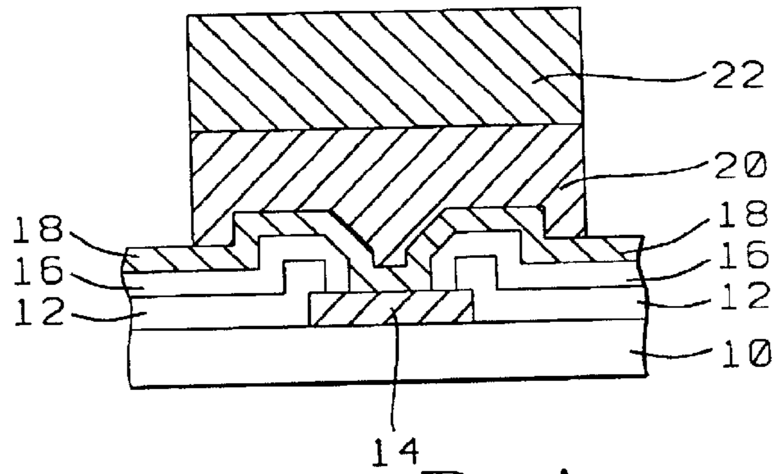
FIG. 3 - Prior Art
