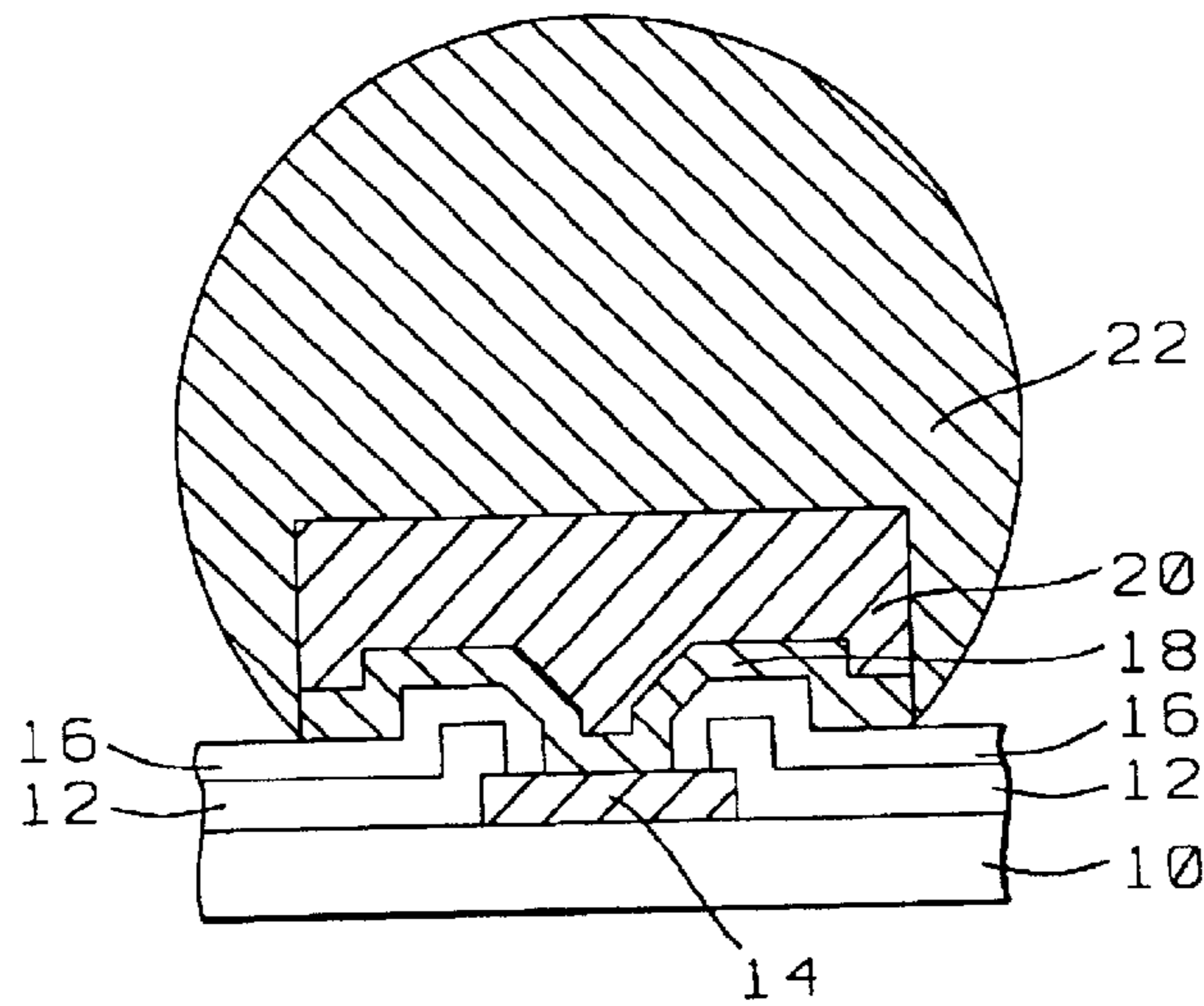
FIG. 4 - Prior Art
