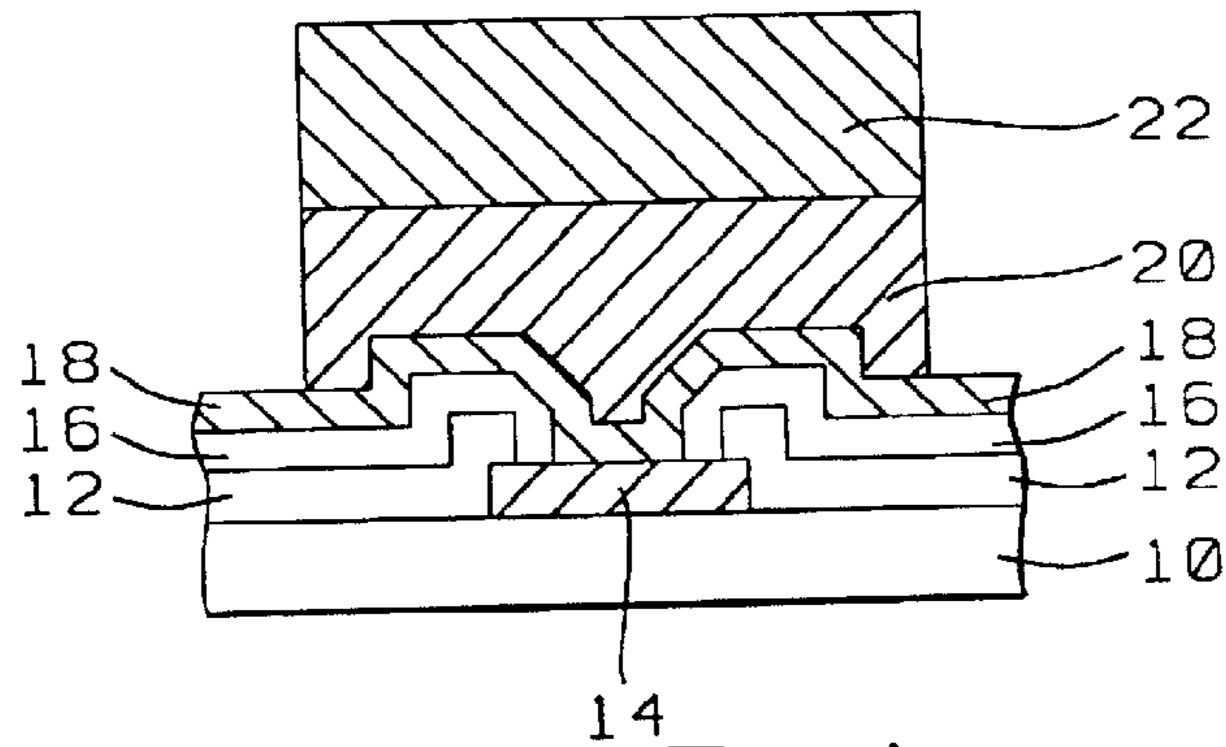
FIG. 3 - Prior Art
