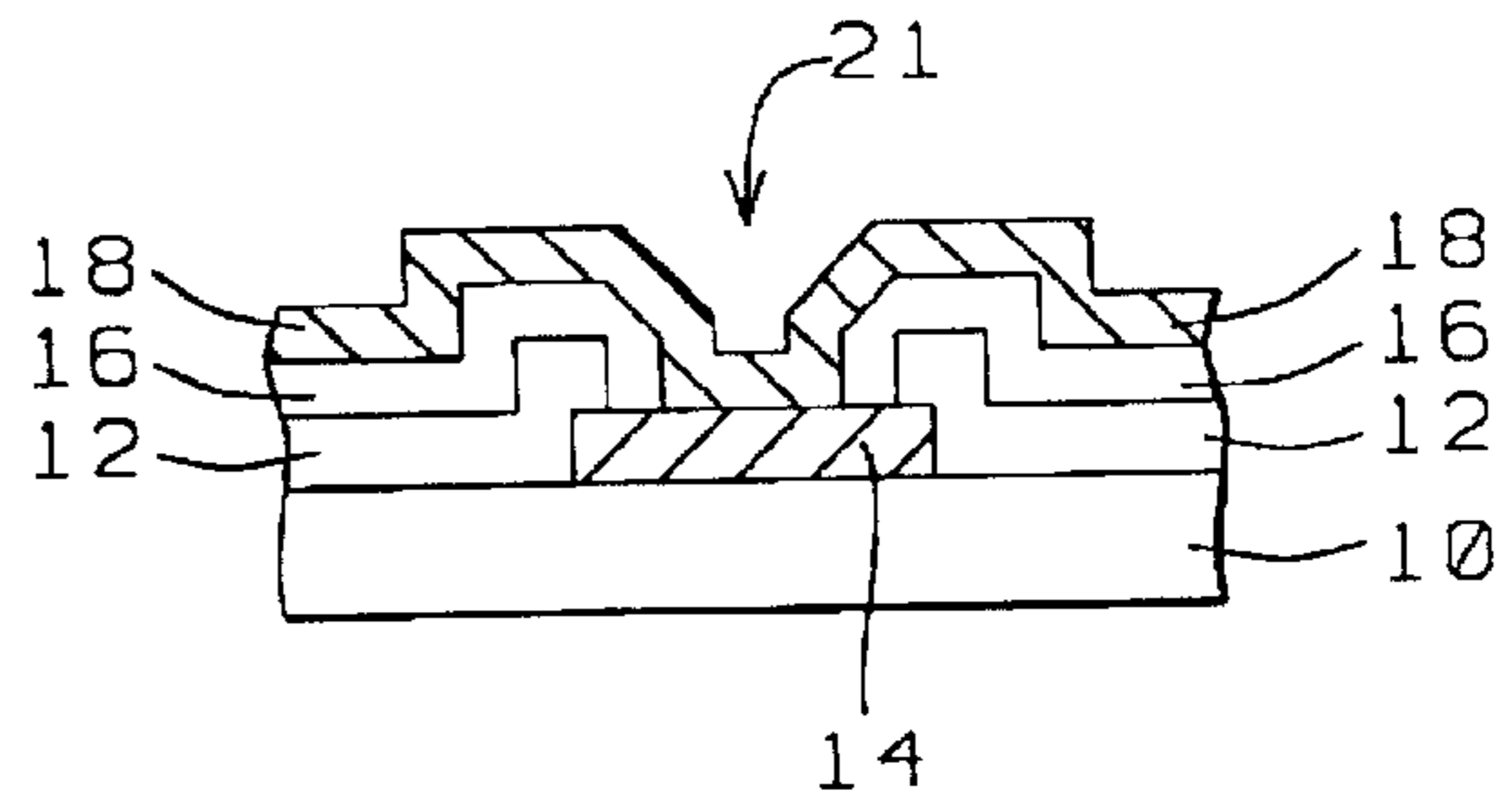
FIG. 2 - Prior Art
