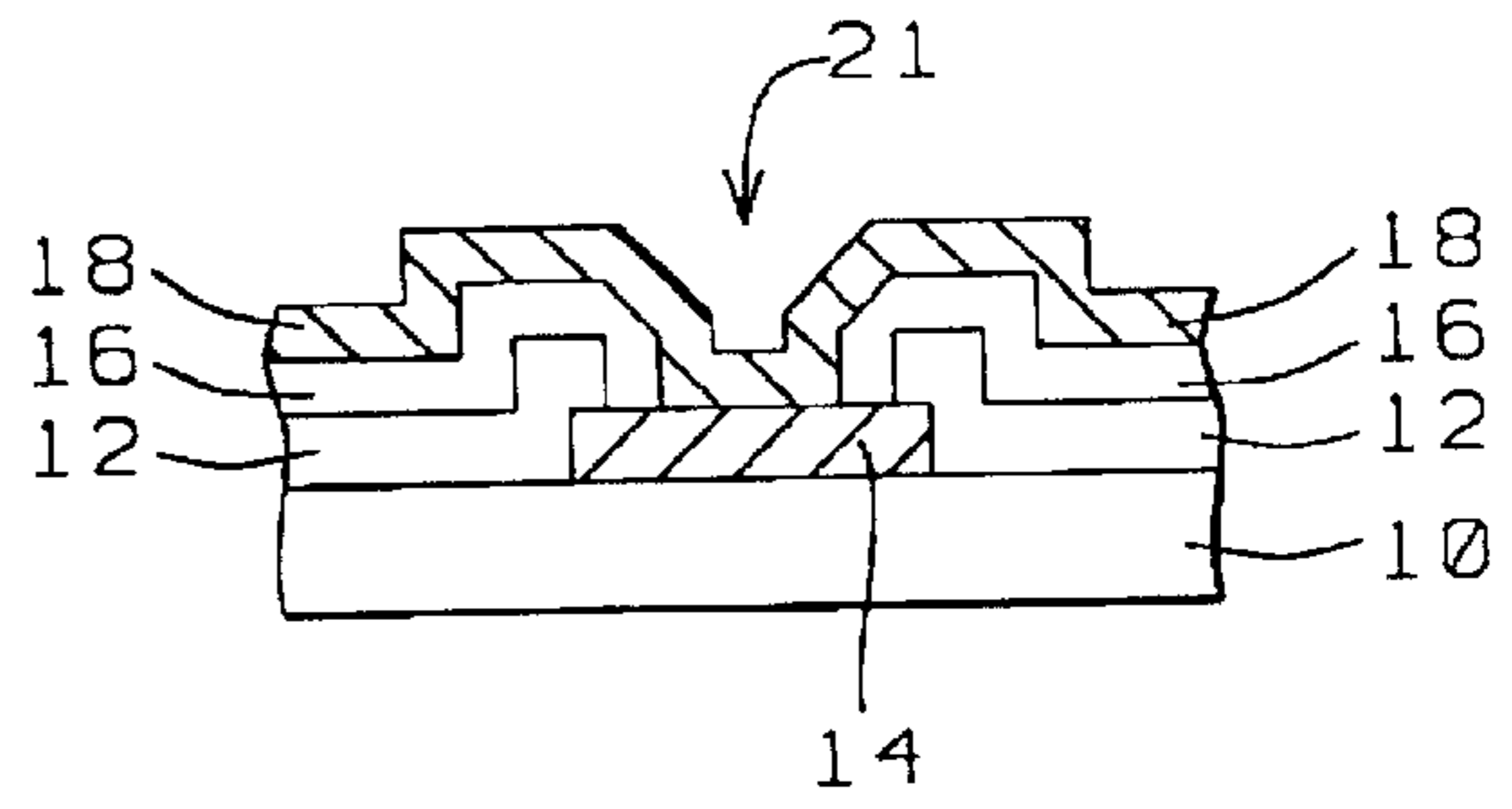
FIG. 2 - Prior Art
