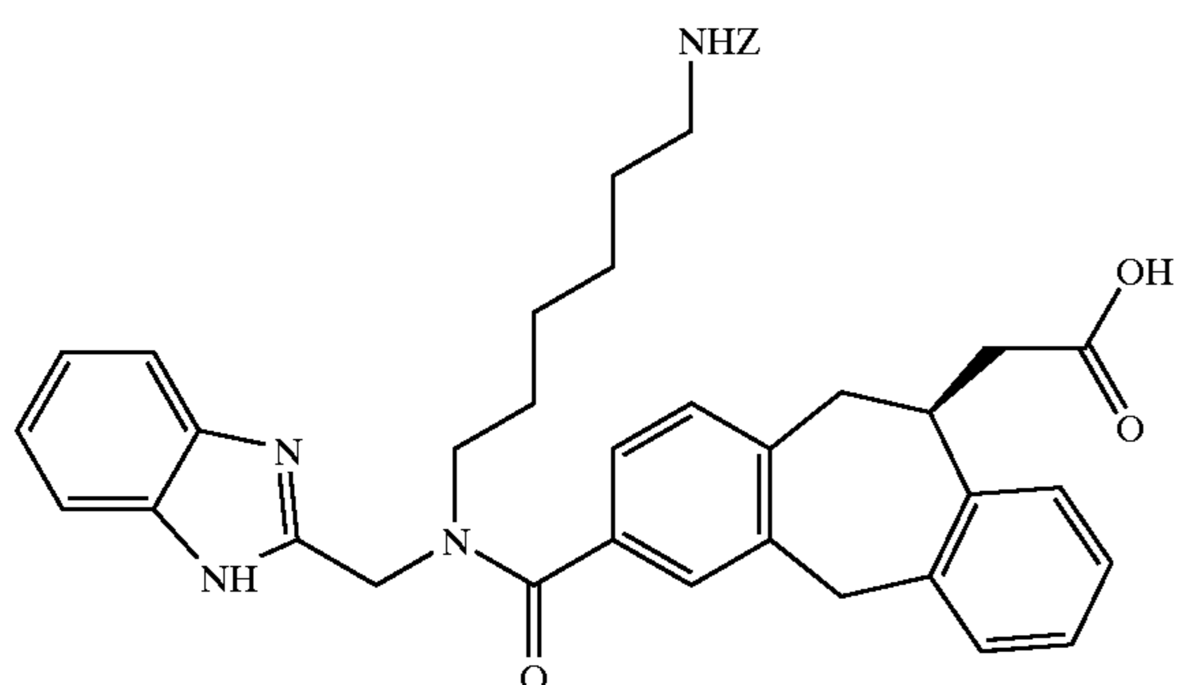
Step 31B: Synthesis of
