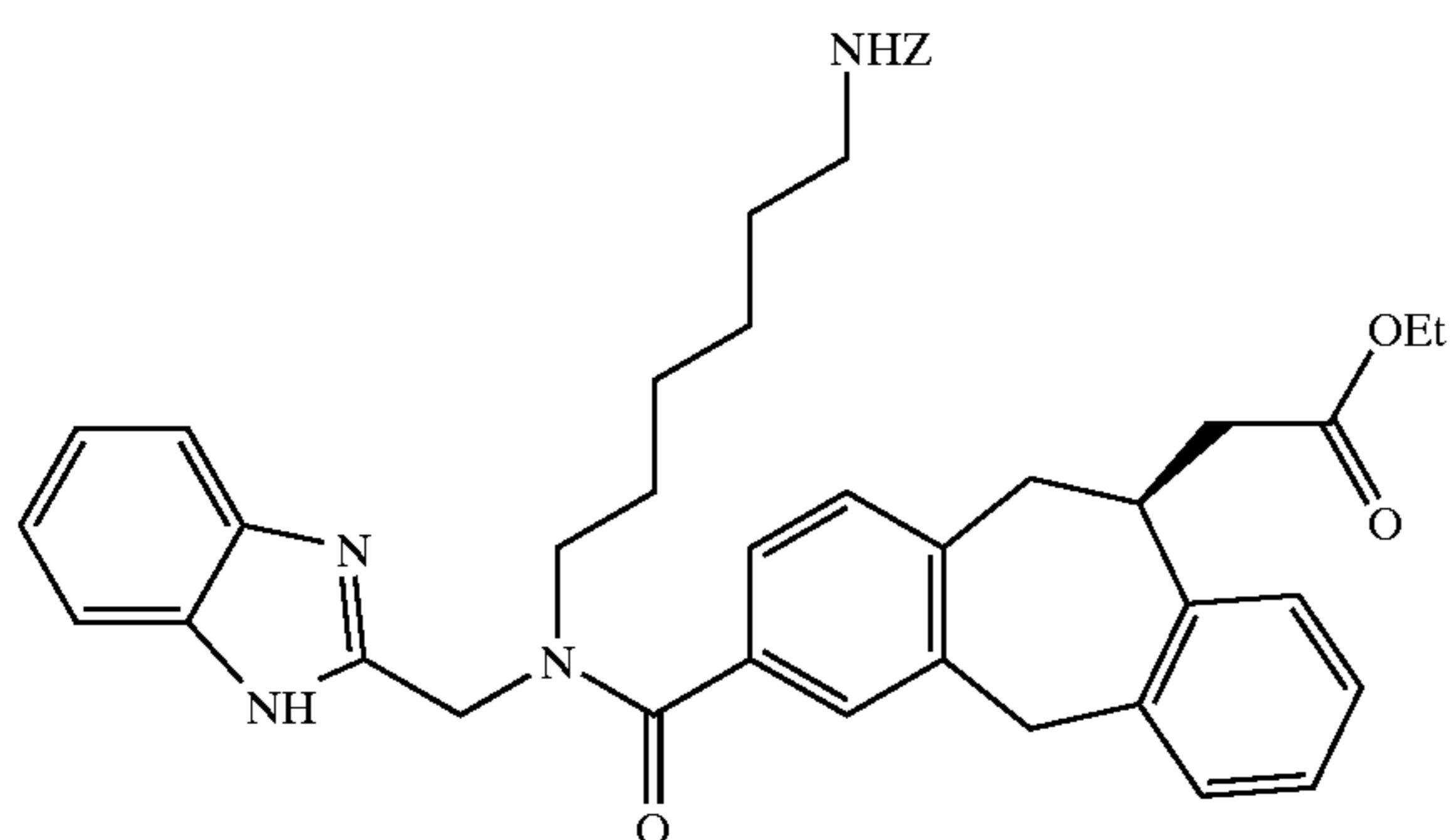
Step 31A: Synthesis of
