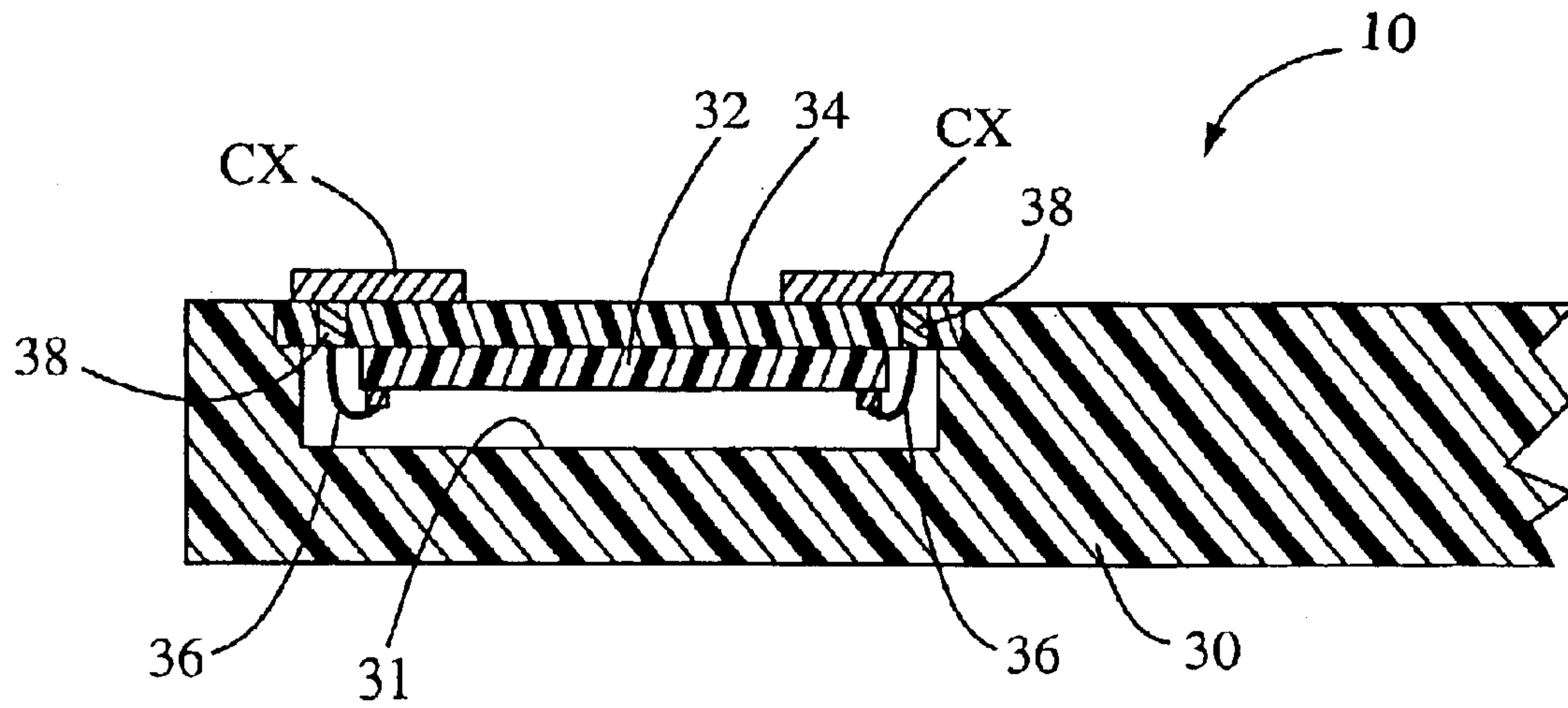
Fig. 3 (PRIOR ART)
