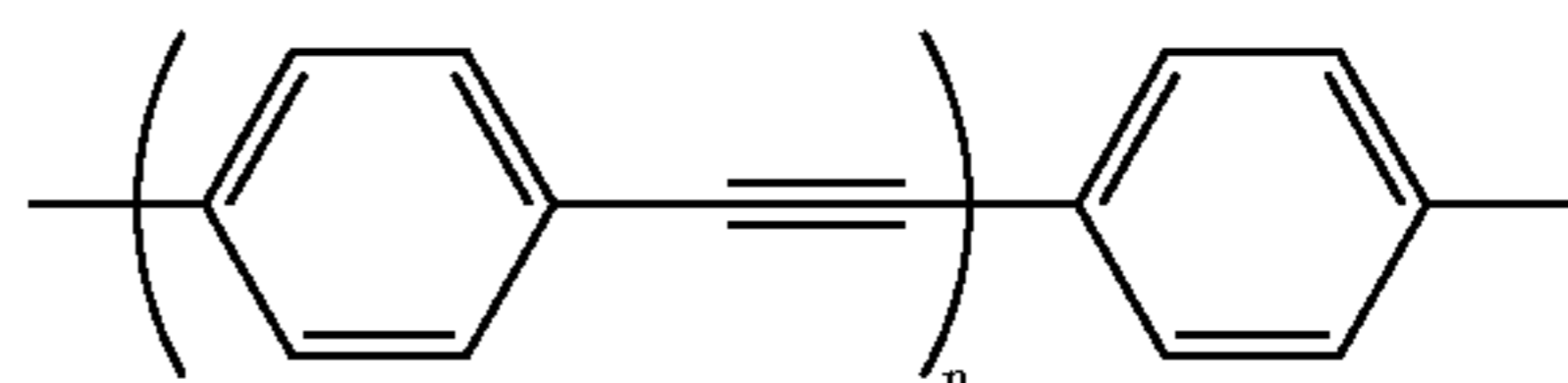
Structural formula (3)
