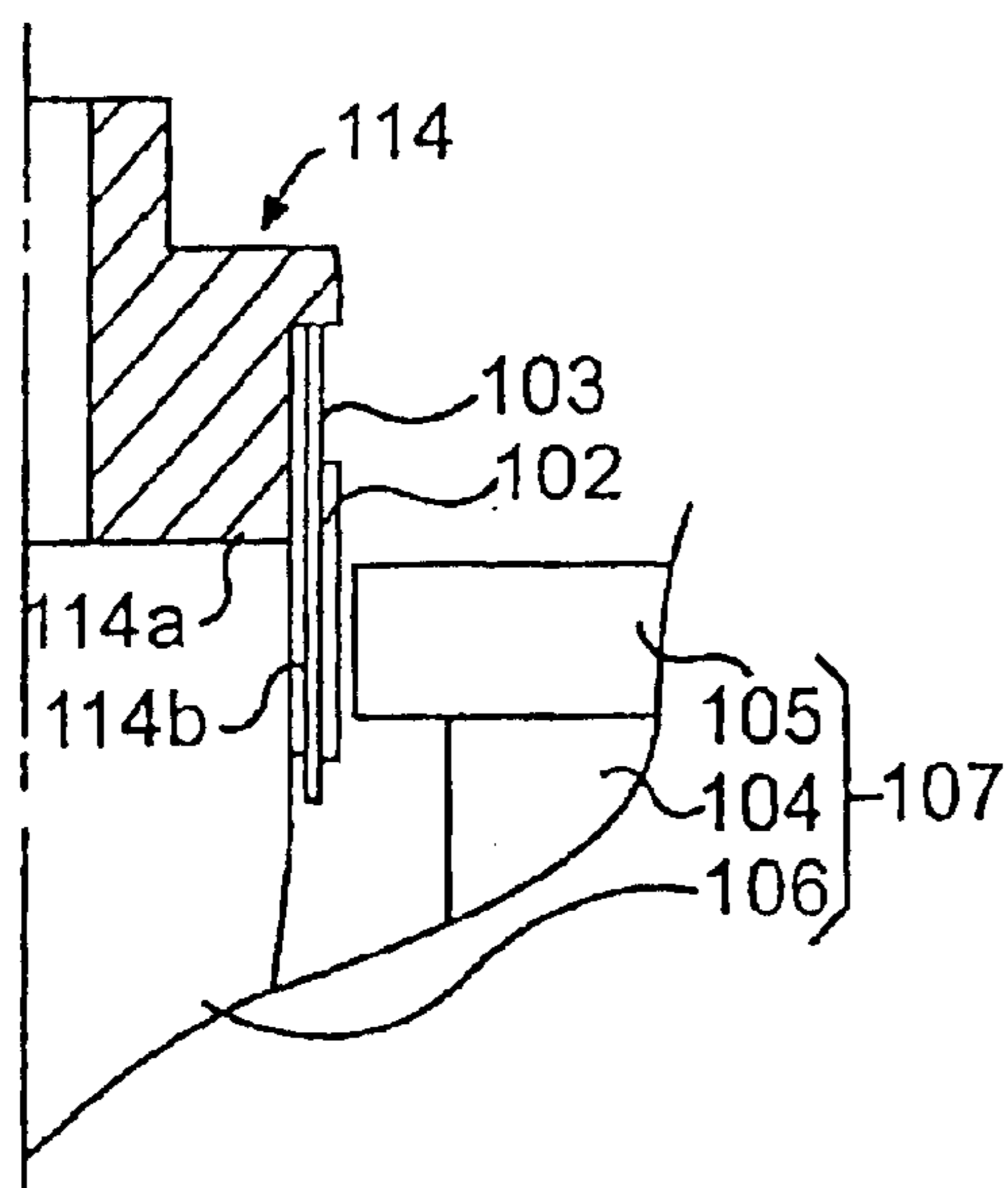
FIG. 12C PRIOR ART
