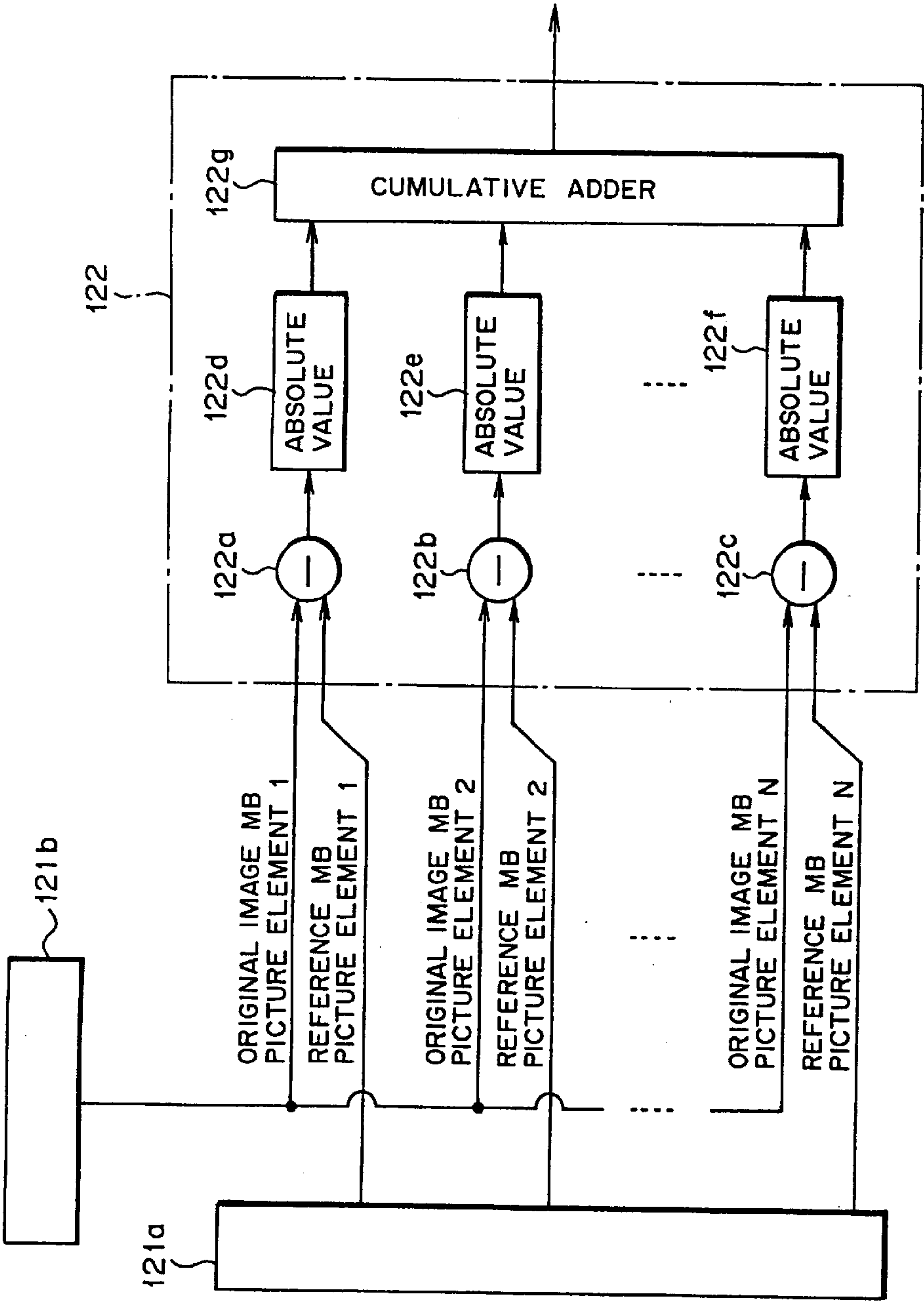
FIG. 19 (PRIOR ART)
