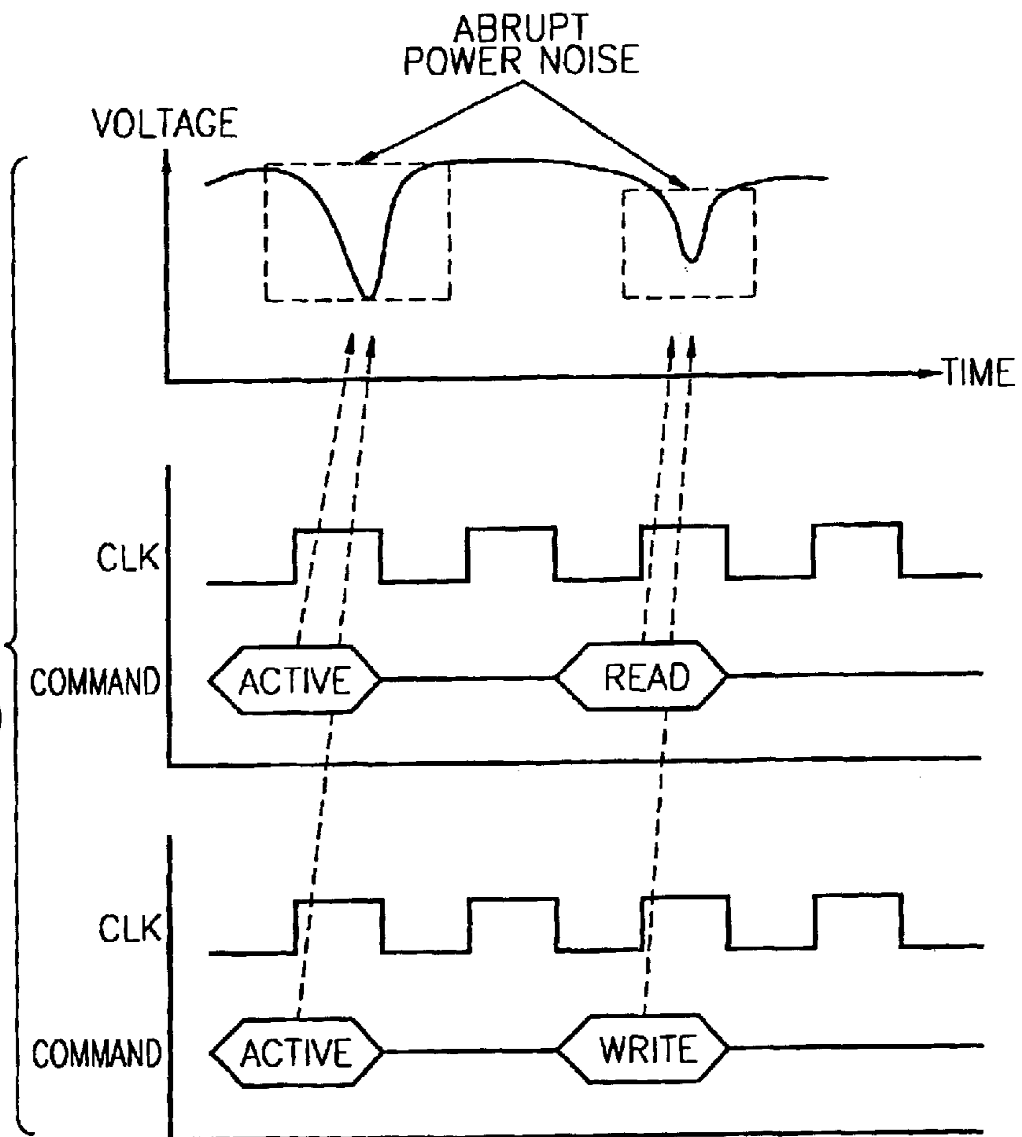
FIG. 2 (PRIOR ART)
