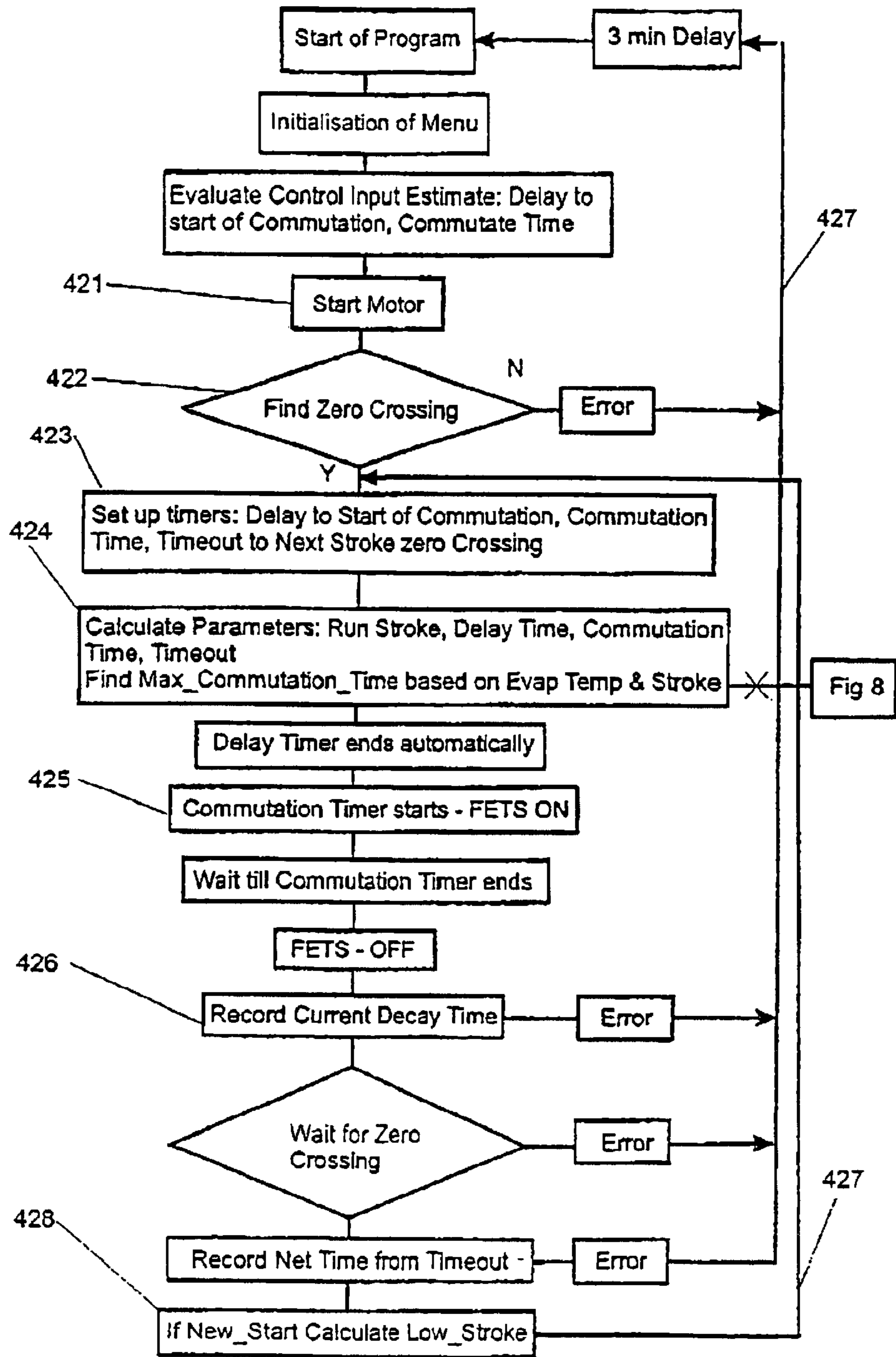
FIGURE 13 Control Microcomputer Motor Control Timing Flow Chart
