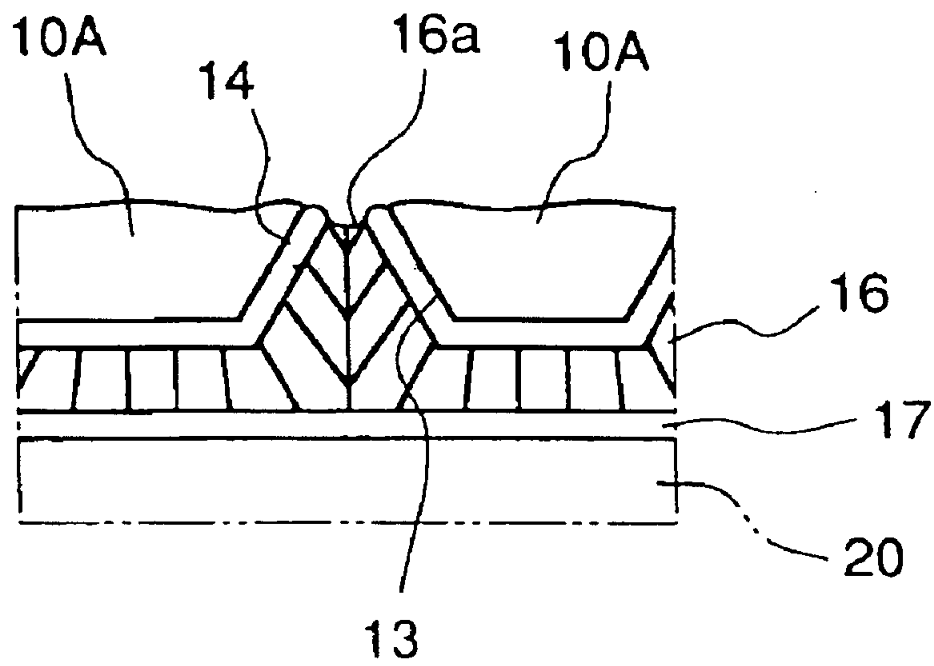
Fig. 14 PRIOR ART
