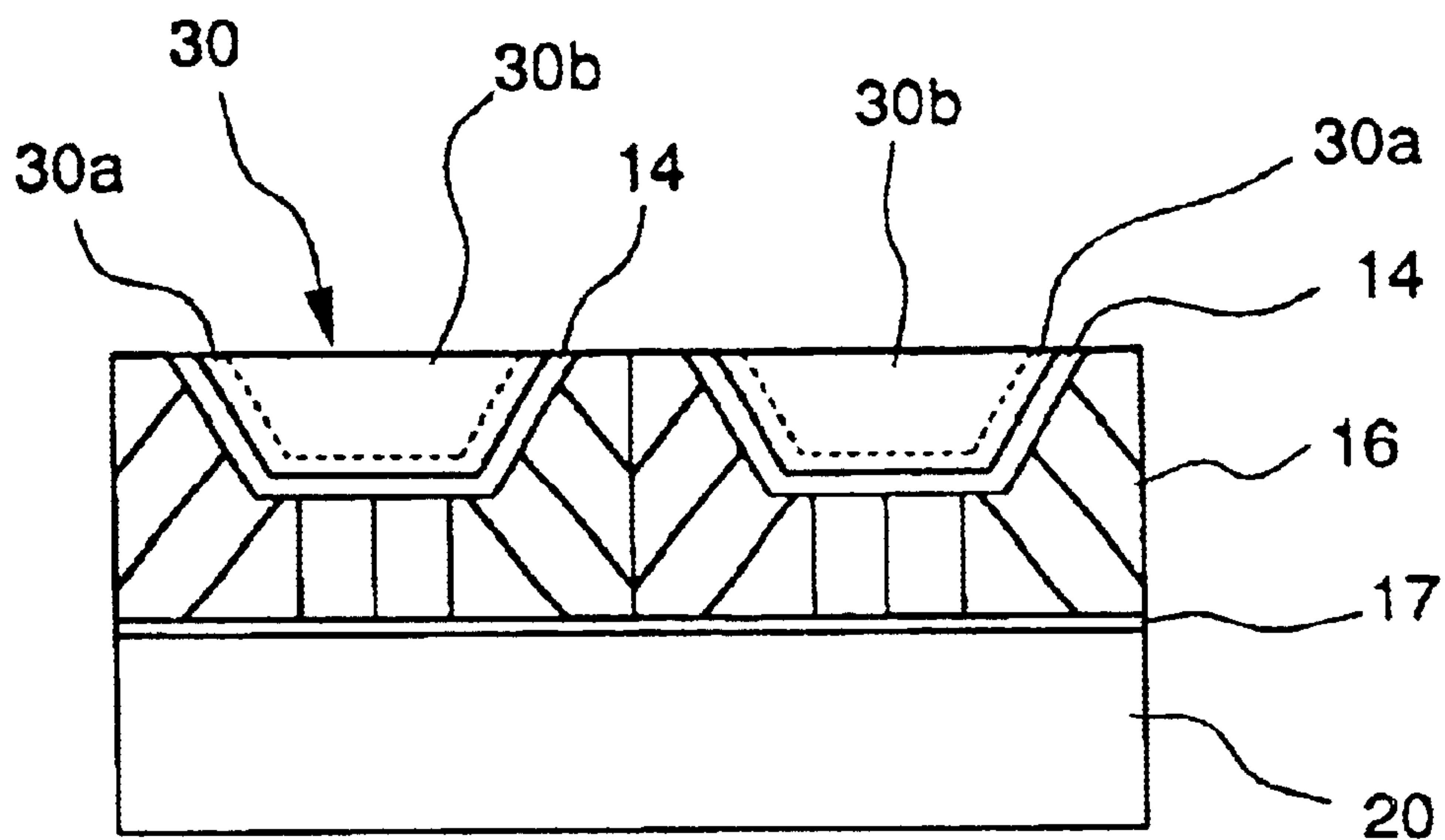
Fig. 16 (PRIOR ART)
