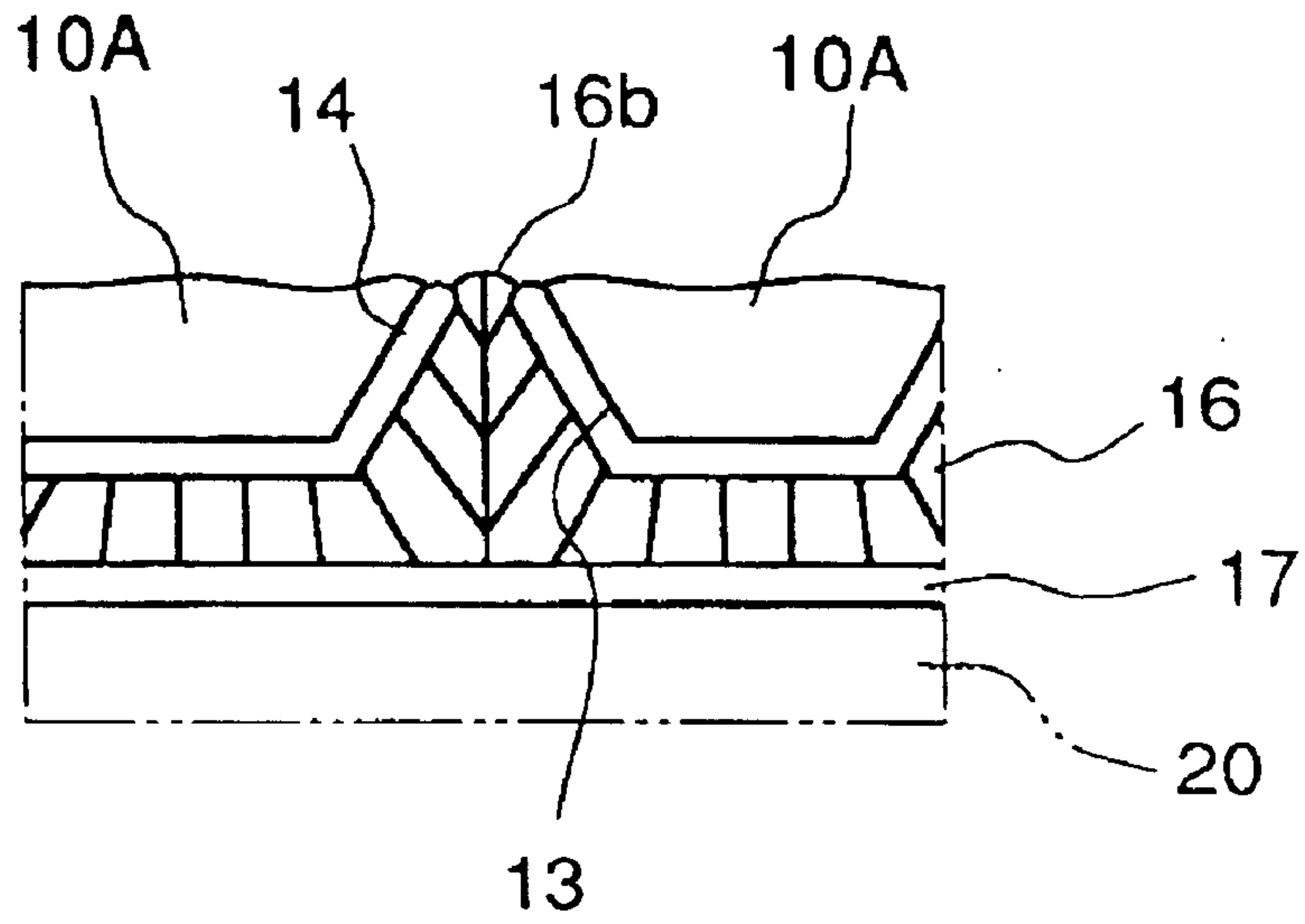
Fig. 13 PRIOR ART
