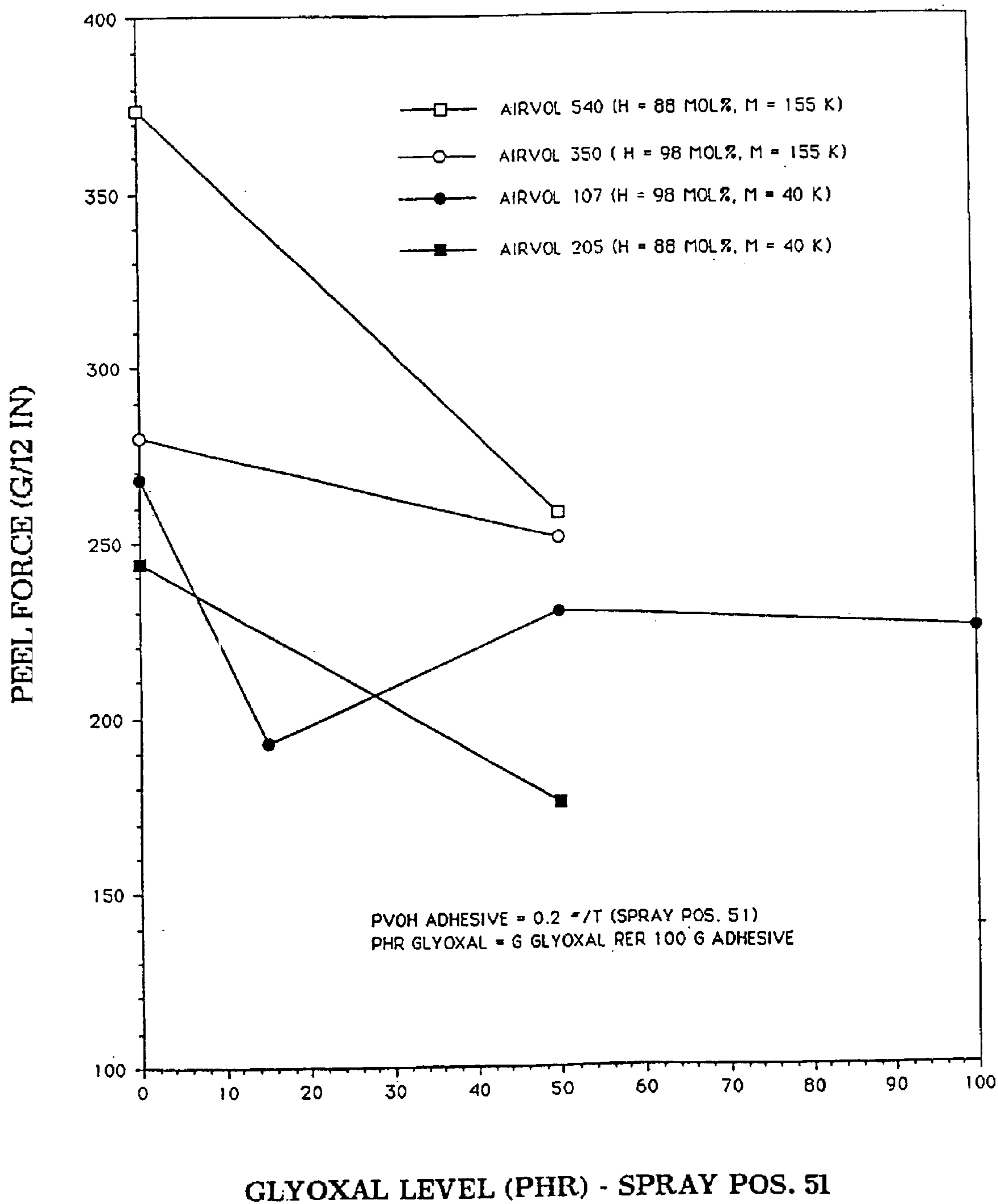
FIGURE 3 PEEL FORCE VERSUS GLYOXAL LEVEL FOR UNFUNCTIONALIZED PVOH
