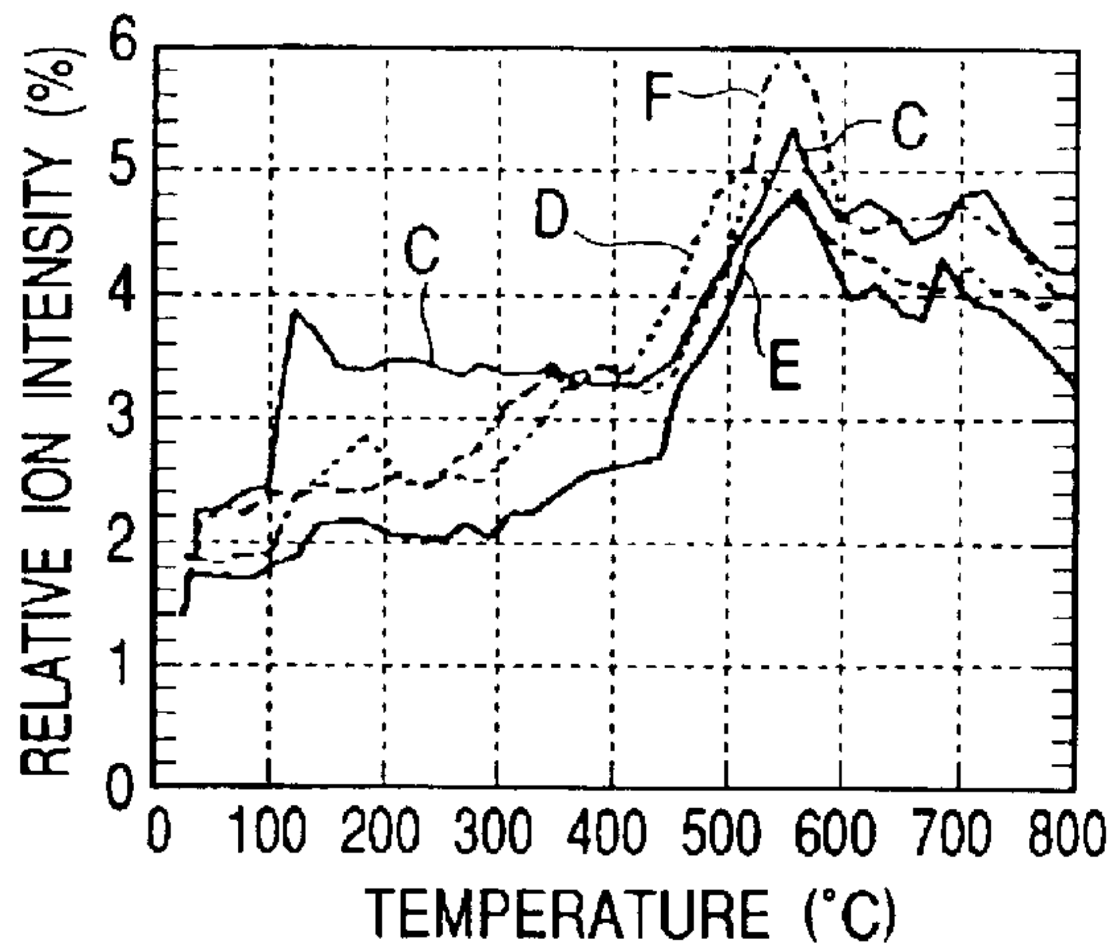
THERMAL ELIMINATION OF HYDROGEN Ar-H m/z=41
