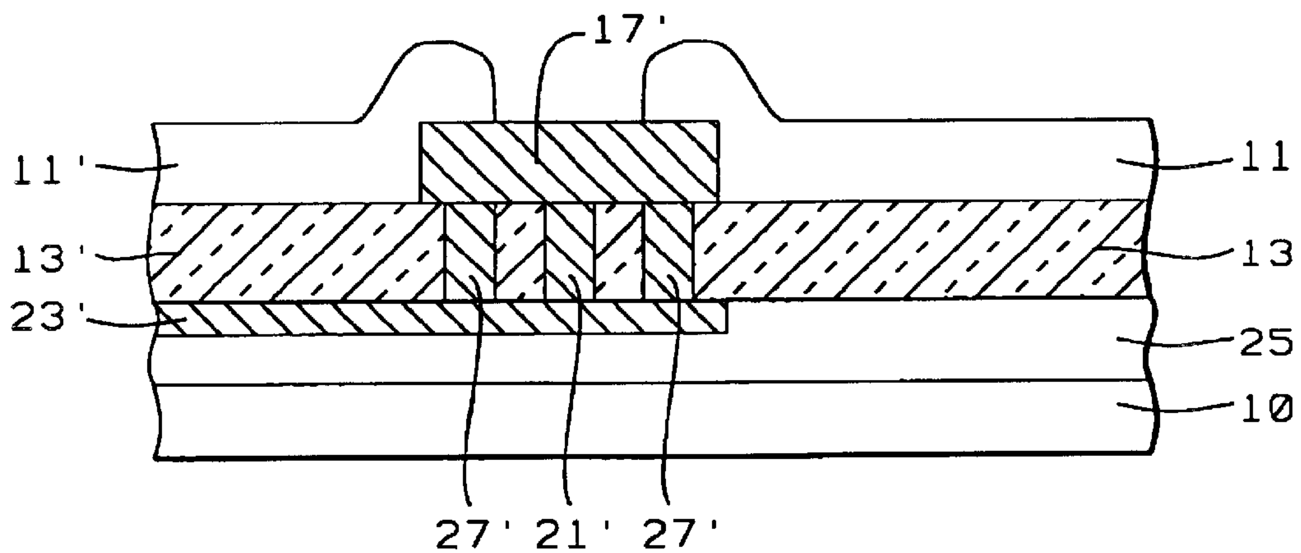
FIG. 20d - Prior Art
