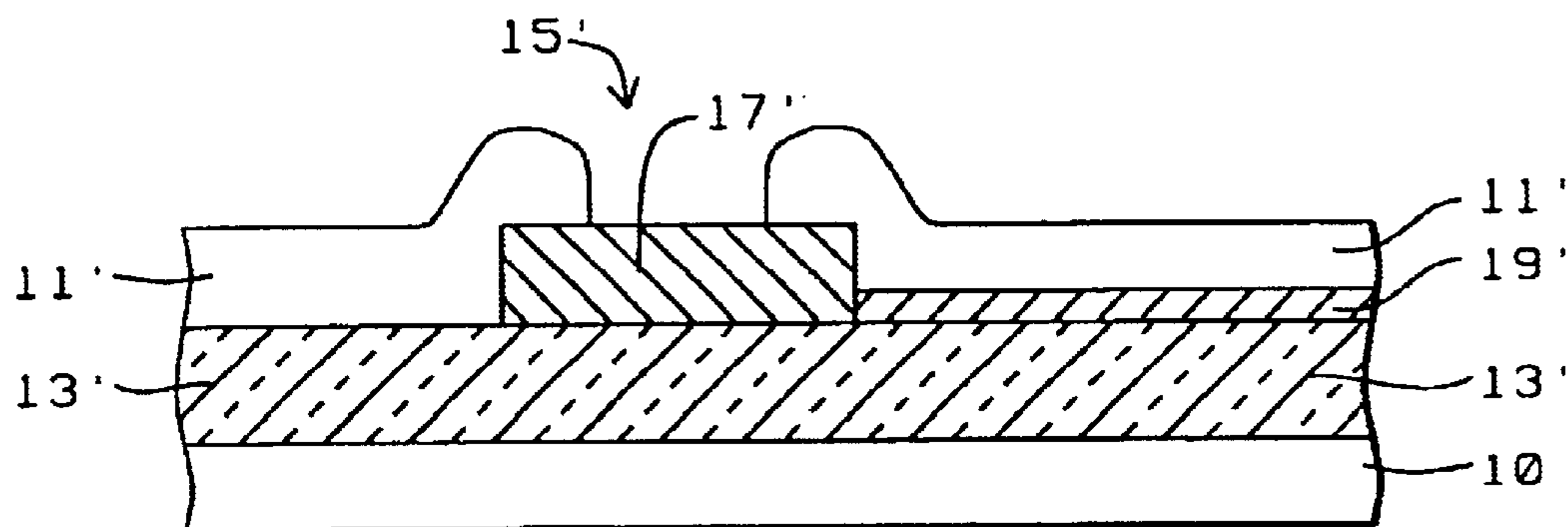
FIG. 19a - Prior Art
