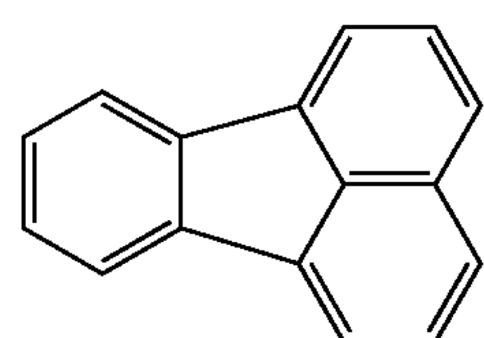
(16) fluoranthene
