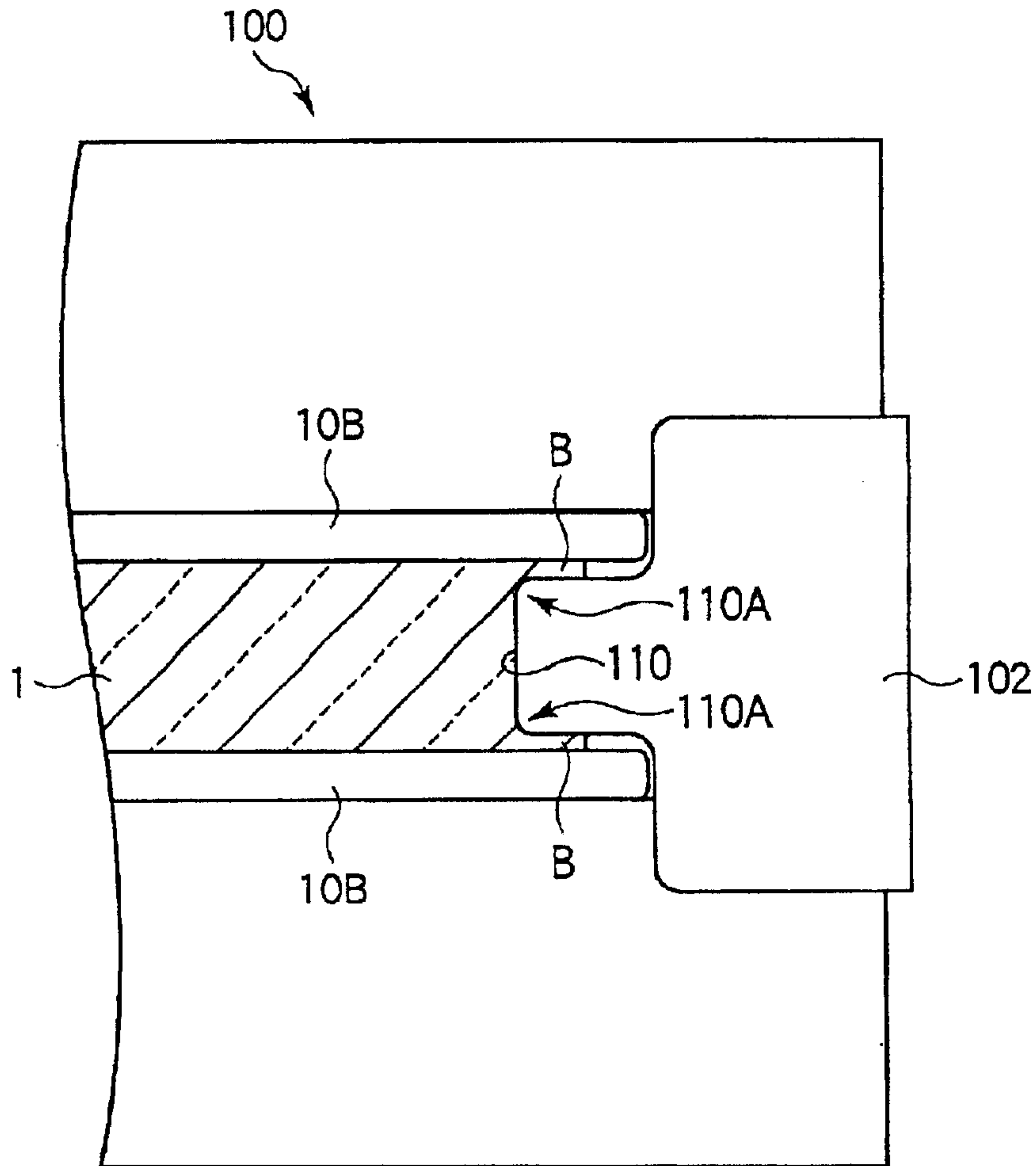
FIG.14A PRIOR ART
